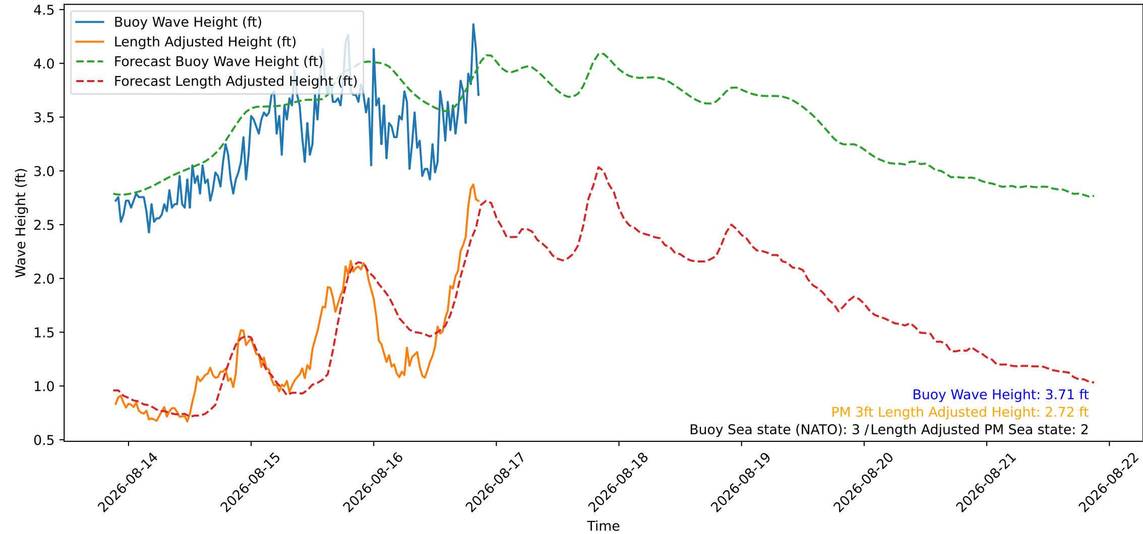
Wave Heights over Time for Green Beach at 2026-08-16 21:11:08
