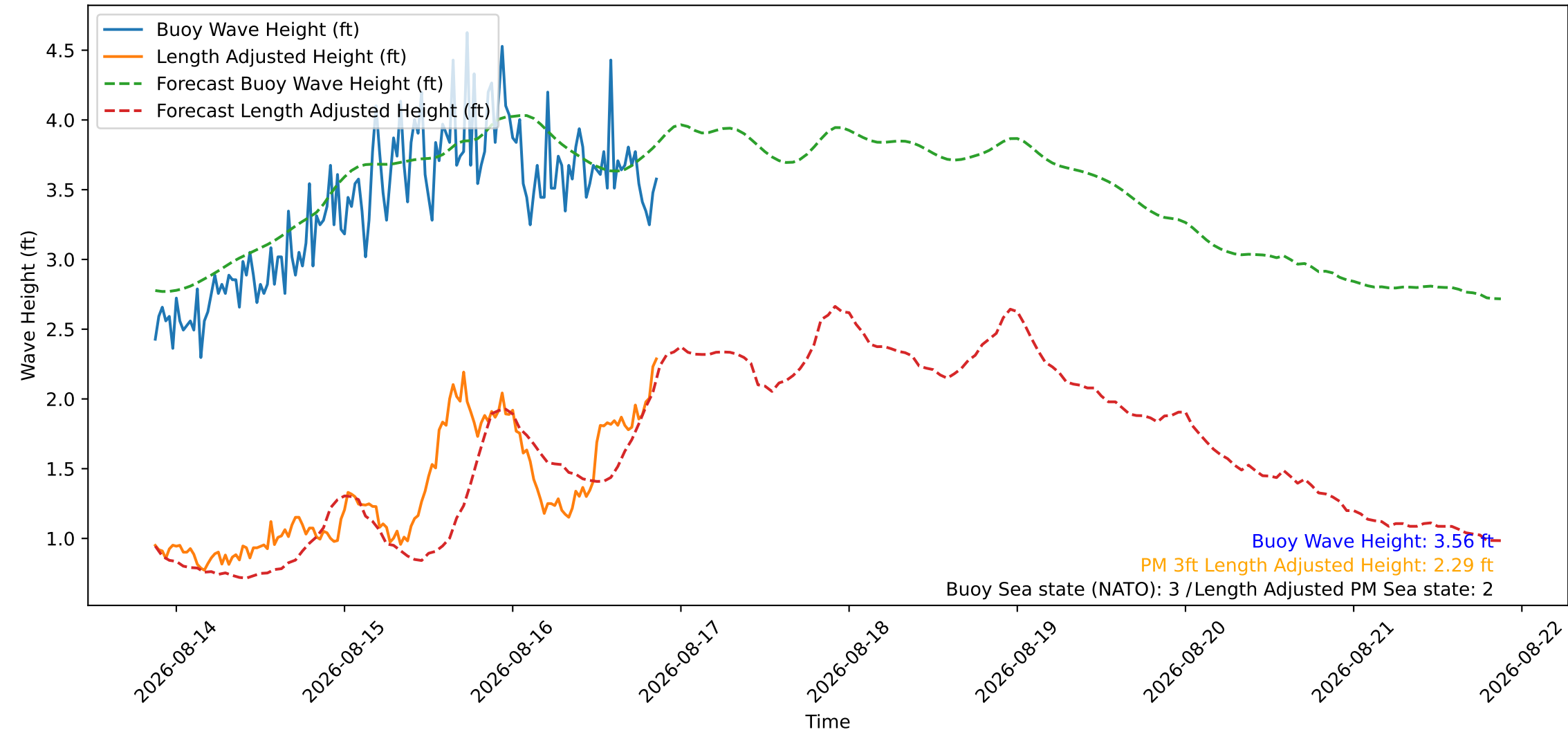
Wave Heights over Time for Oceanside Harbor at 2026-08-16 21:10:26
