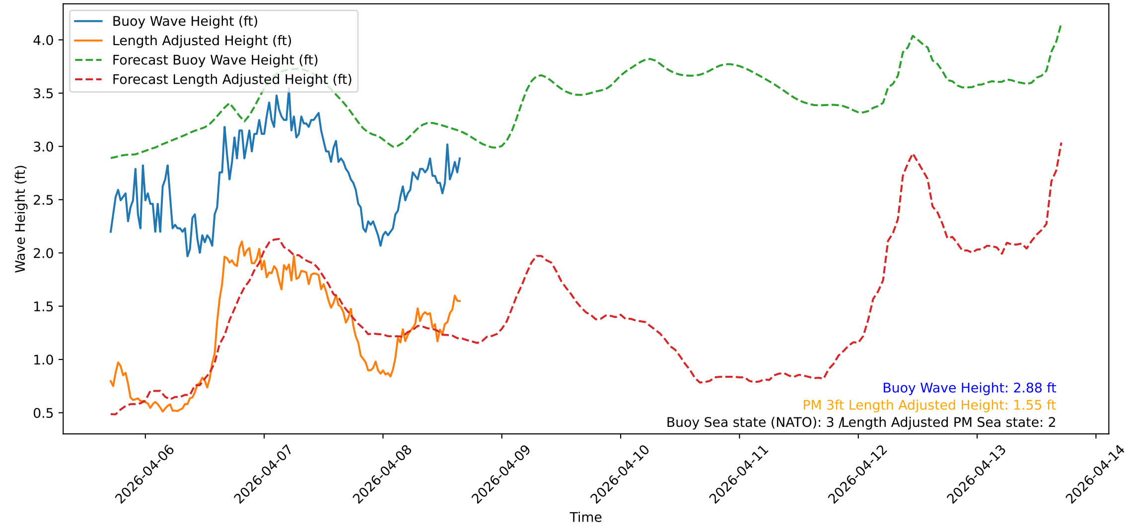
Wave Heights over Time for Red Beach at 2026-04-08 16:30:47
