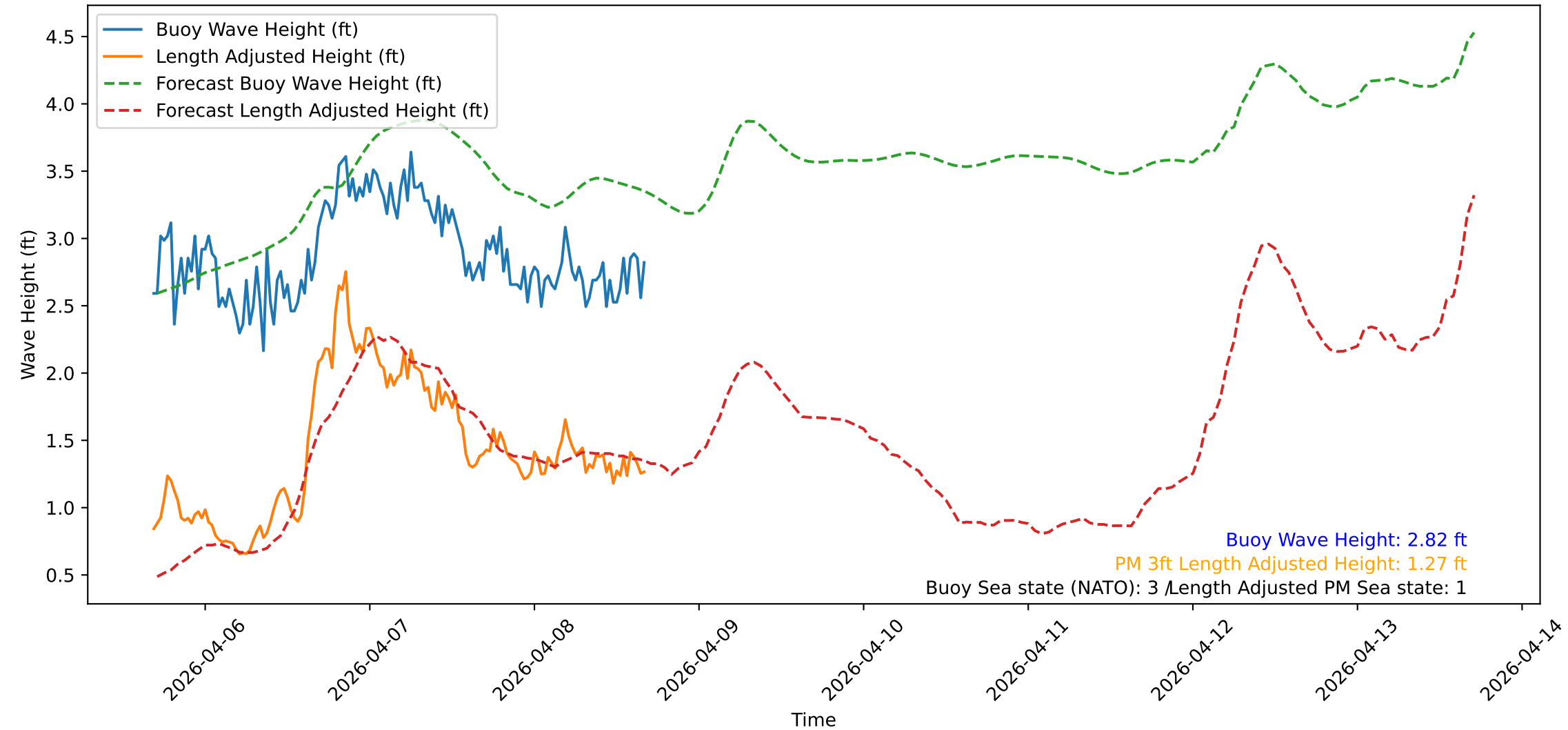
Wave Heights over Time for Oceanside Harbor at 2026-04-08 16:30:31
