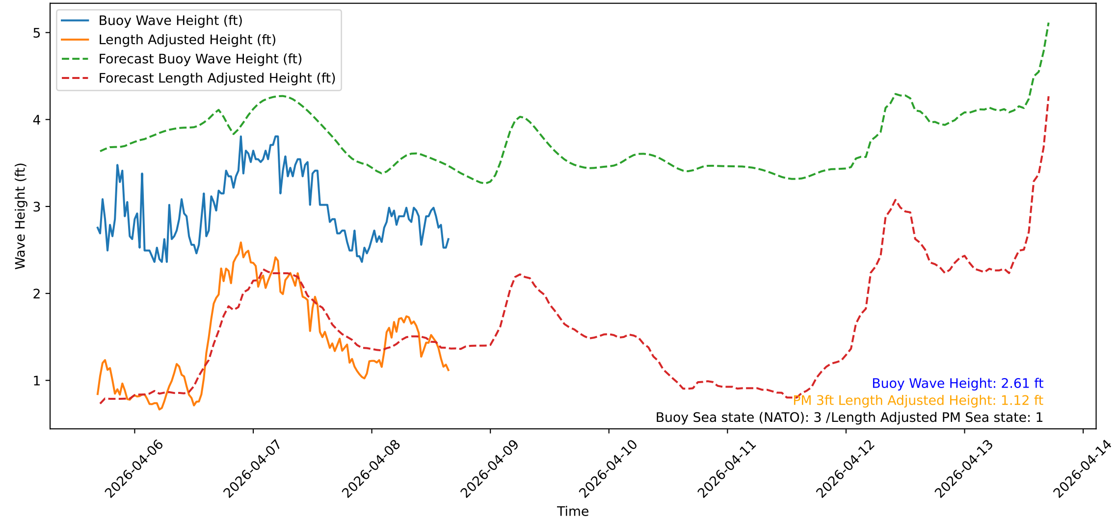
Wave Heights over Time for Green Beach at 2026-04-08 16:31:09
