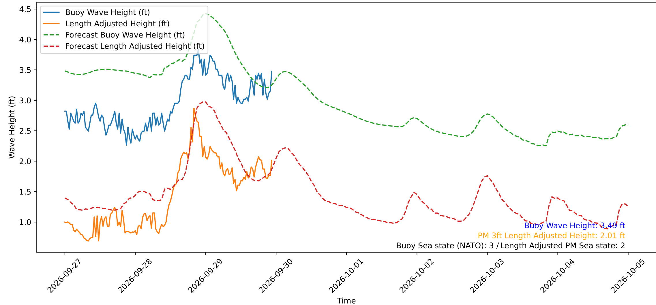
Wave Heights over Time for Red Beach at 2026-09-29 23:30:50
