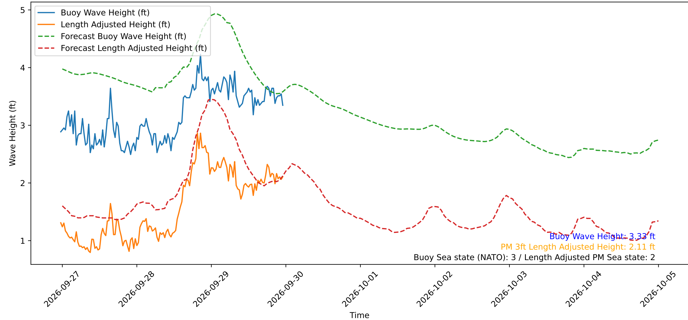
Wave Heights over Time for Oceanside Harbor at 2026-09-29 23:30:30
