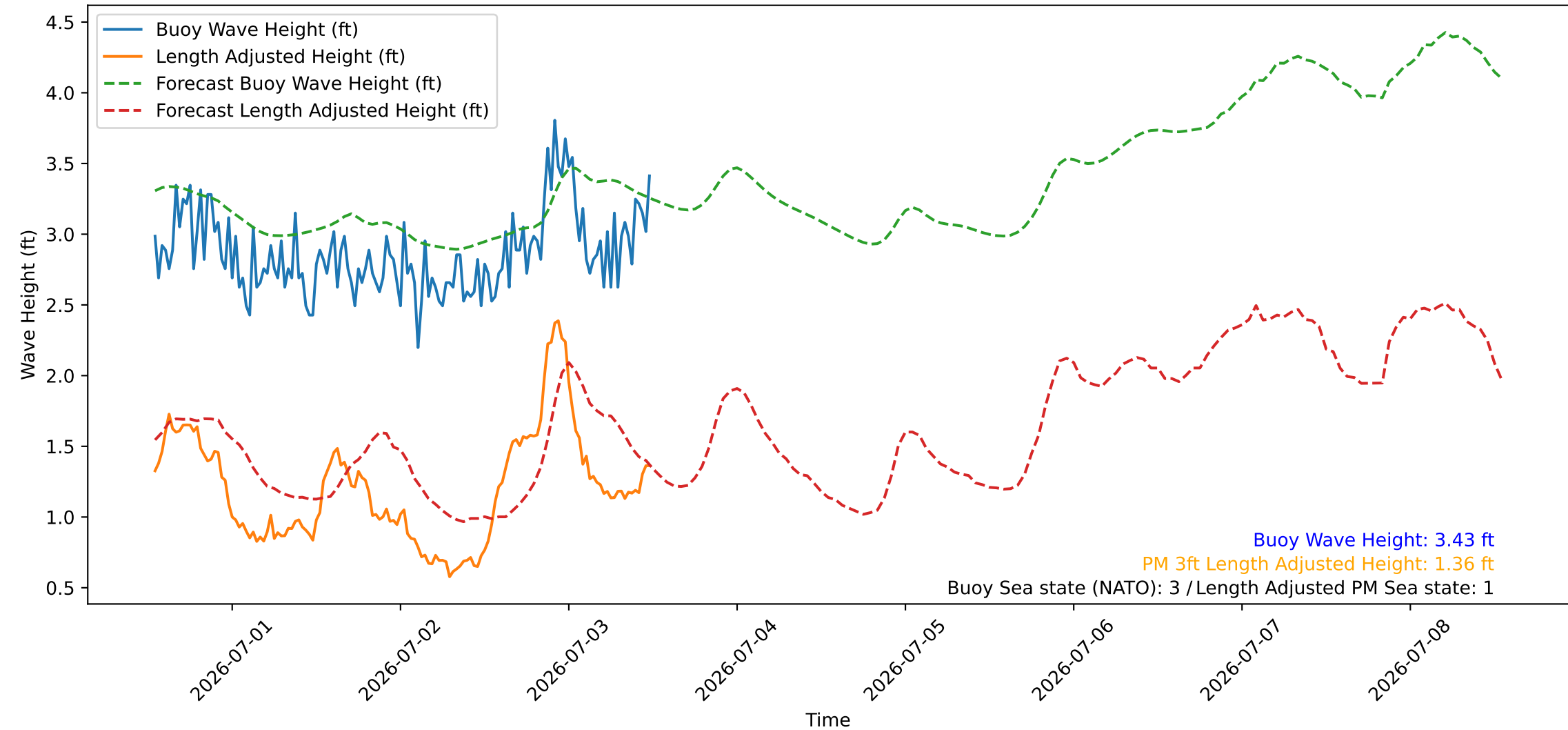
Wave Heights over Time for Red Beach at 2026-07-03 12:30:46
