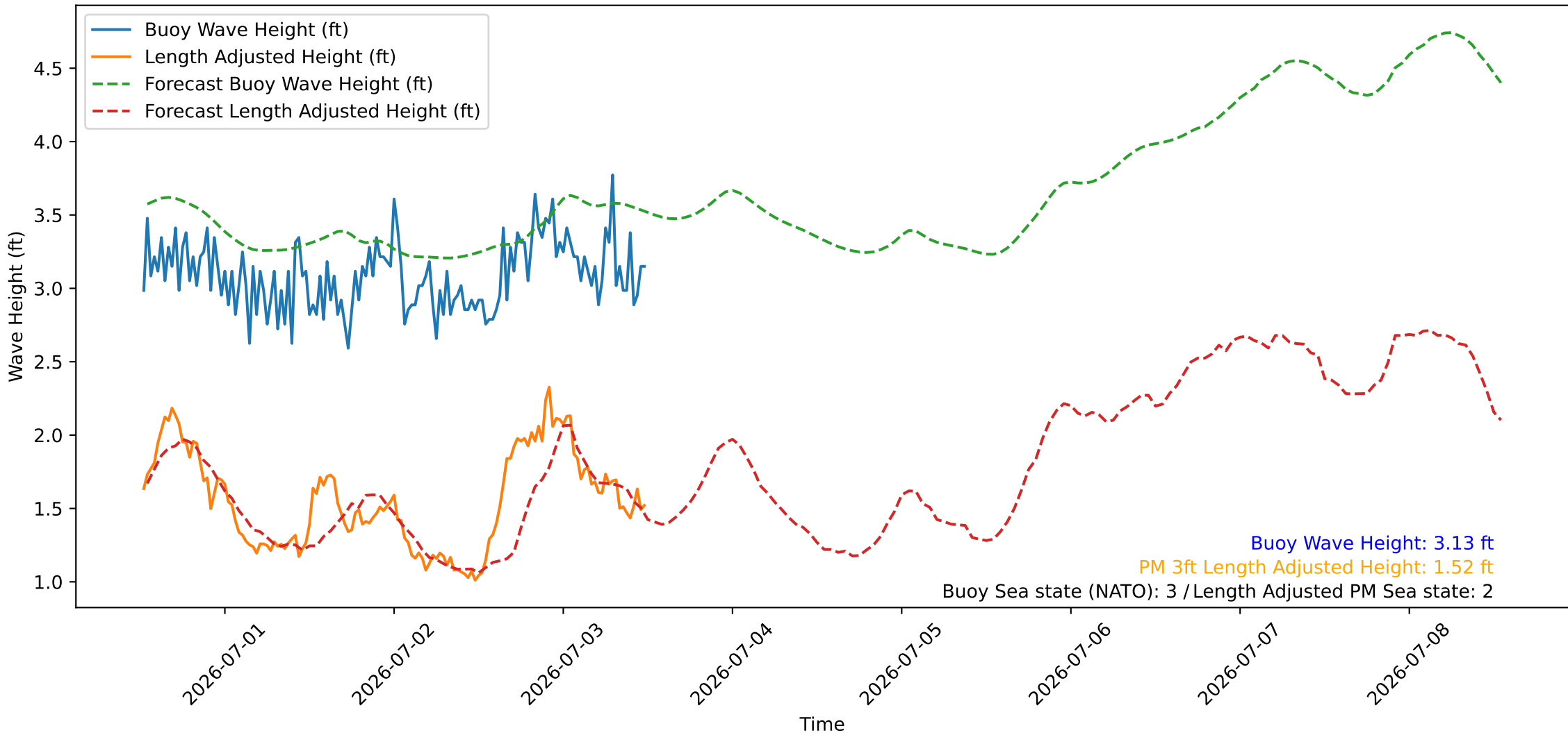
Wave Heights over Time for Oceanside Harbor at 2026-07-03 12:30:26
