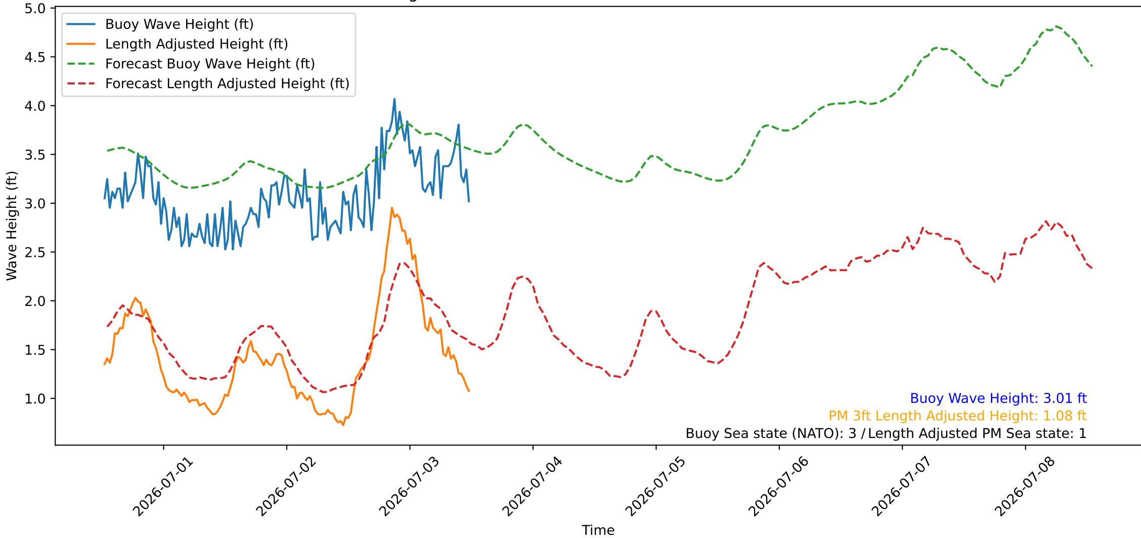
Wave Heights over Time for Green Beach at 2026-07-03 12:31:08
