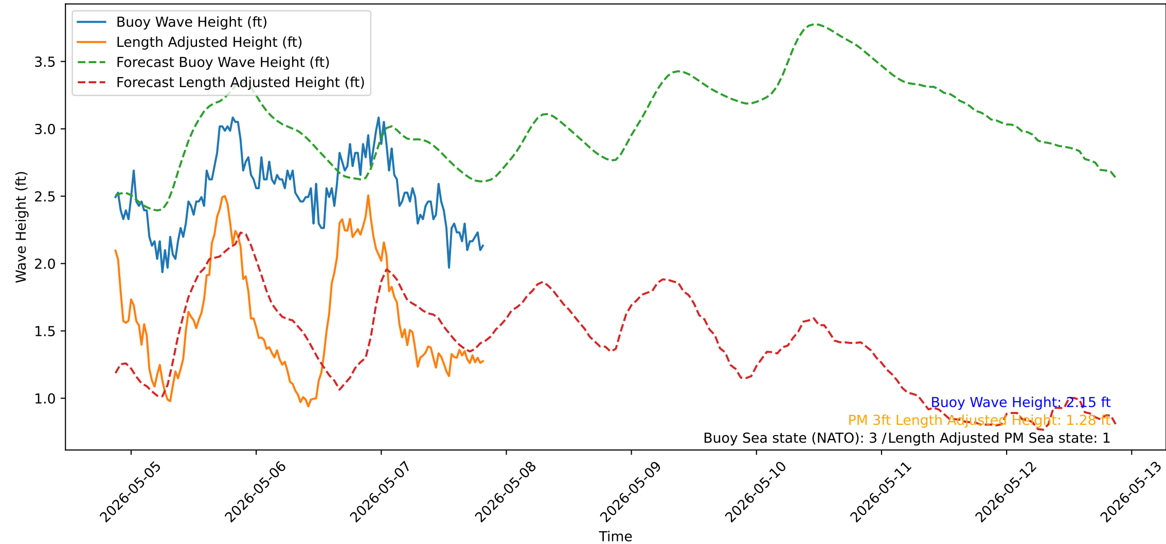
Wave Heights over Time for Red Beach at 2026-05-07 20:40:53
