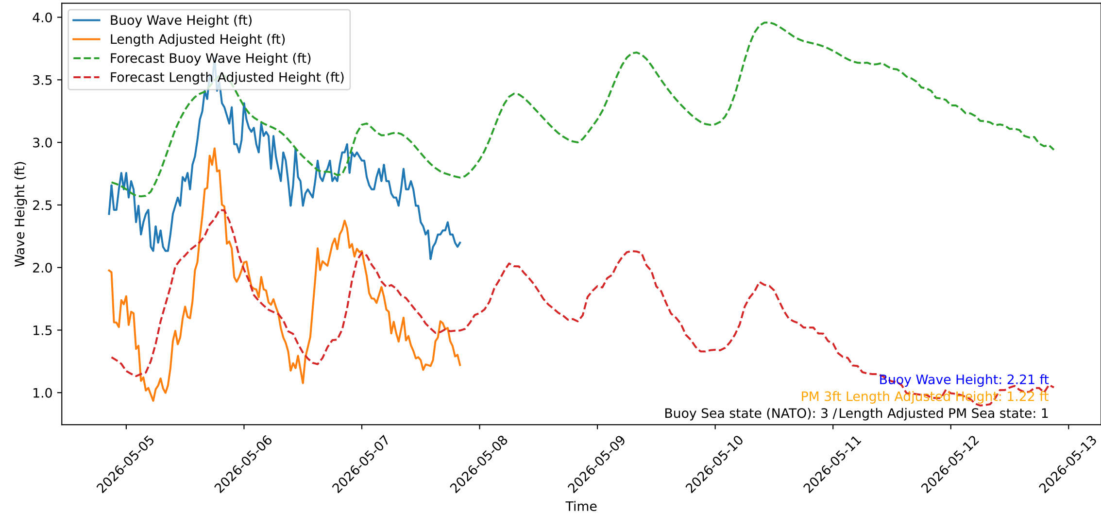
Wave Heights over Time for Green Beach at 2026-05-07 20:41:15
