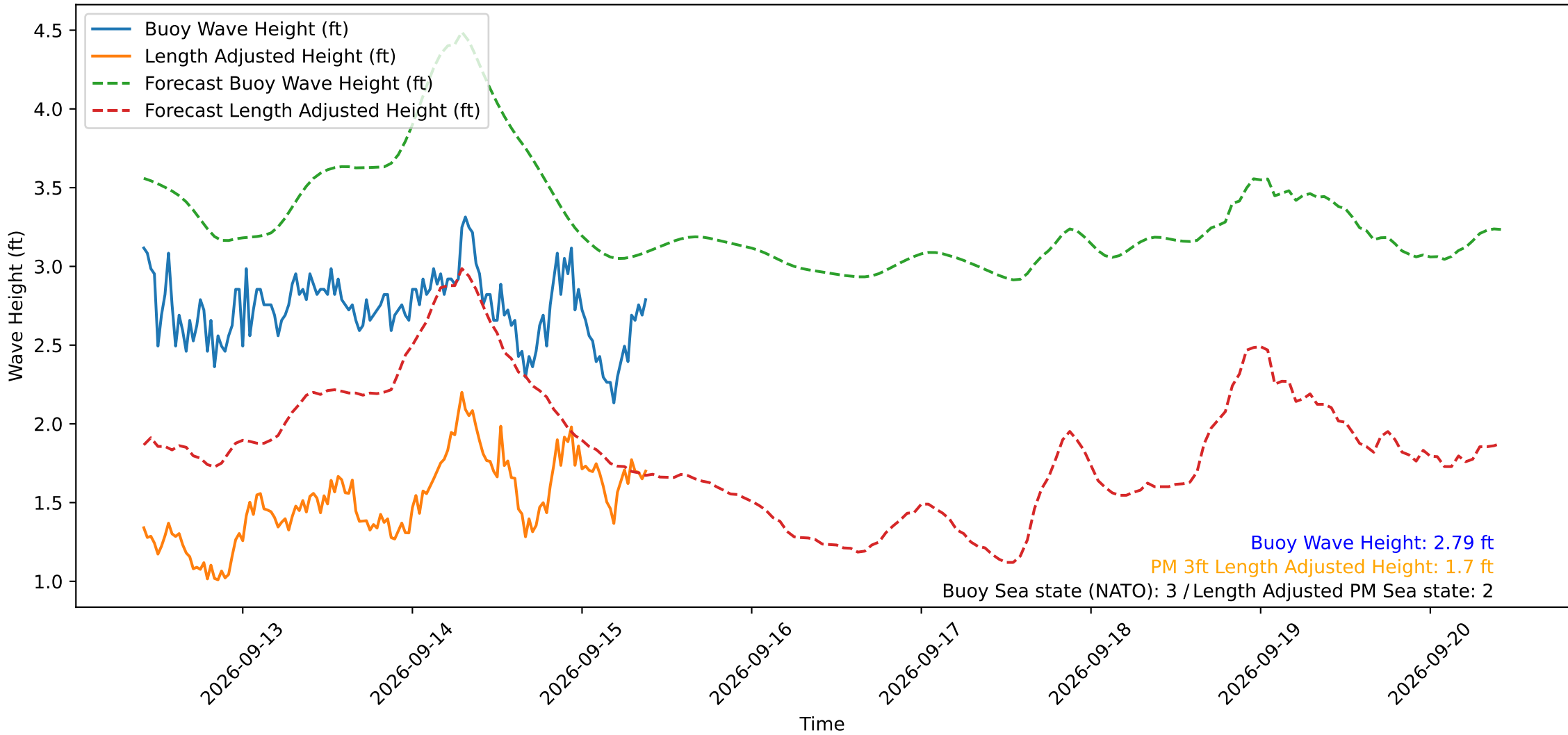
Wave Heights over Time for Green Beach at 2026-09-15 09:51:14
