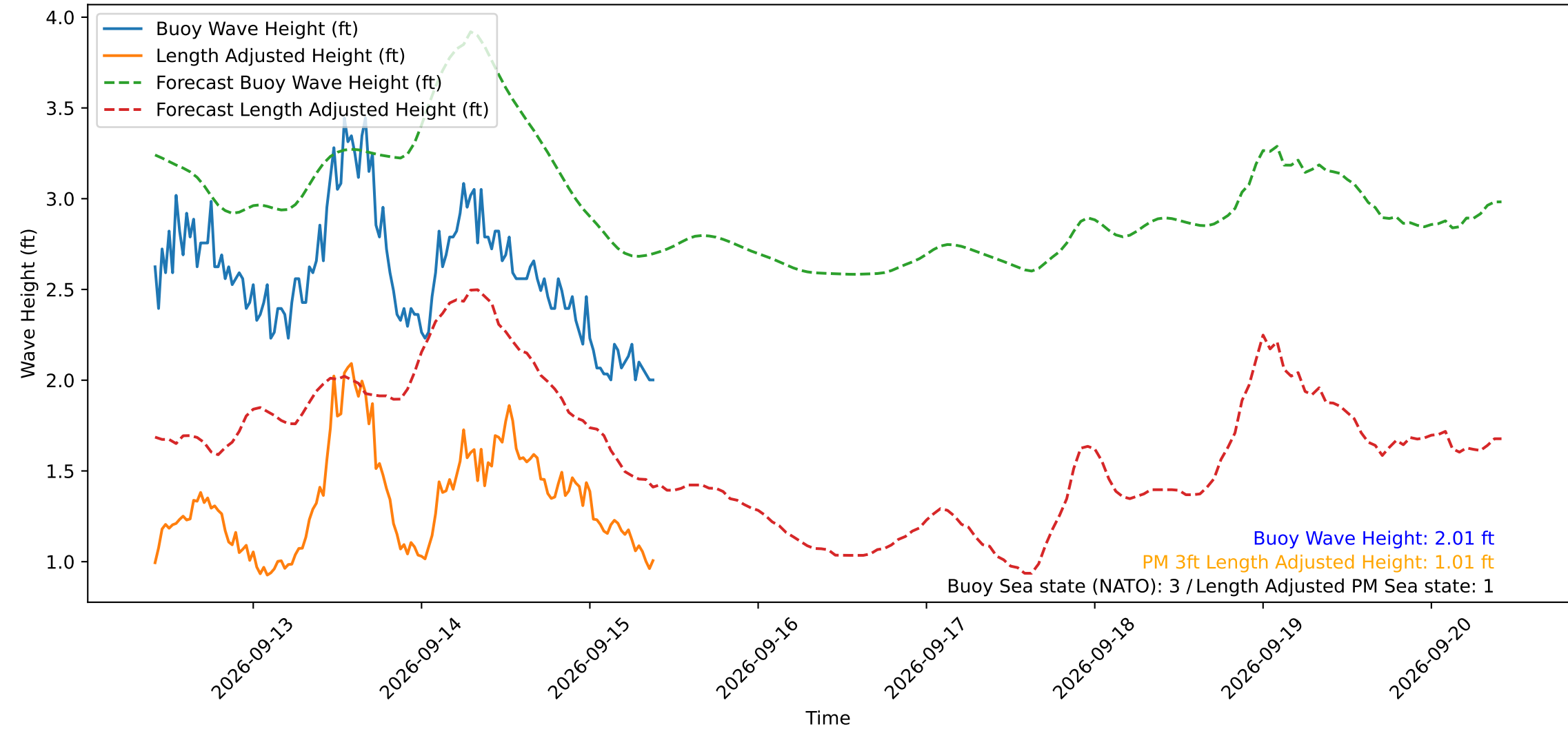
Wave Heights over Time for Red Beach at 2026-09-15 09:50:50
