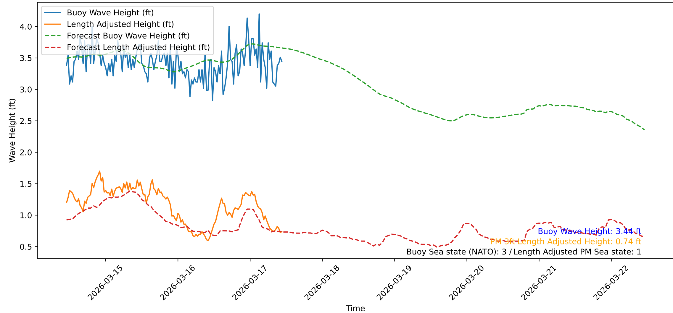
Wave Heights over Time for Green Beach at 2026-03-17 11:11:41
