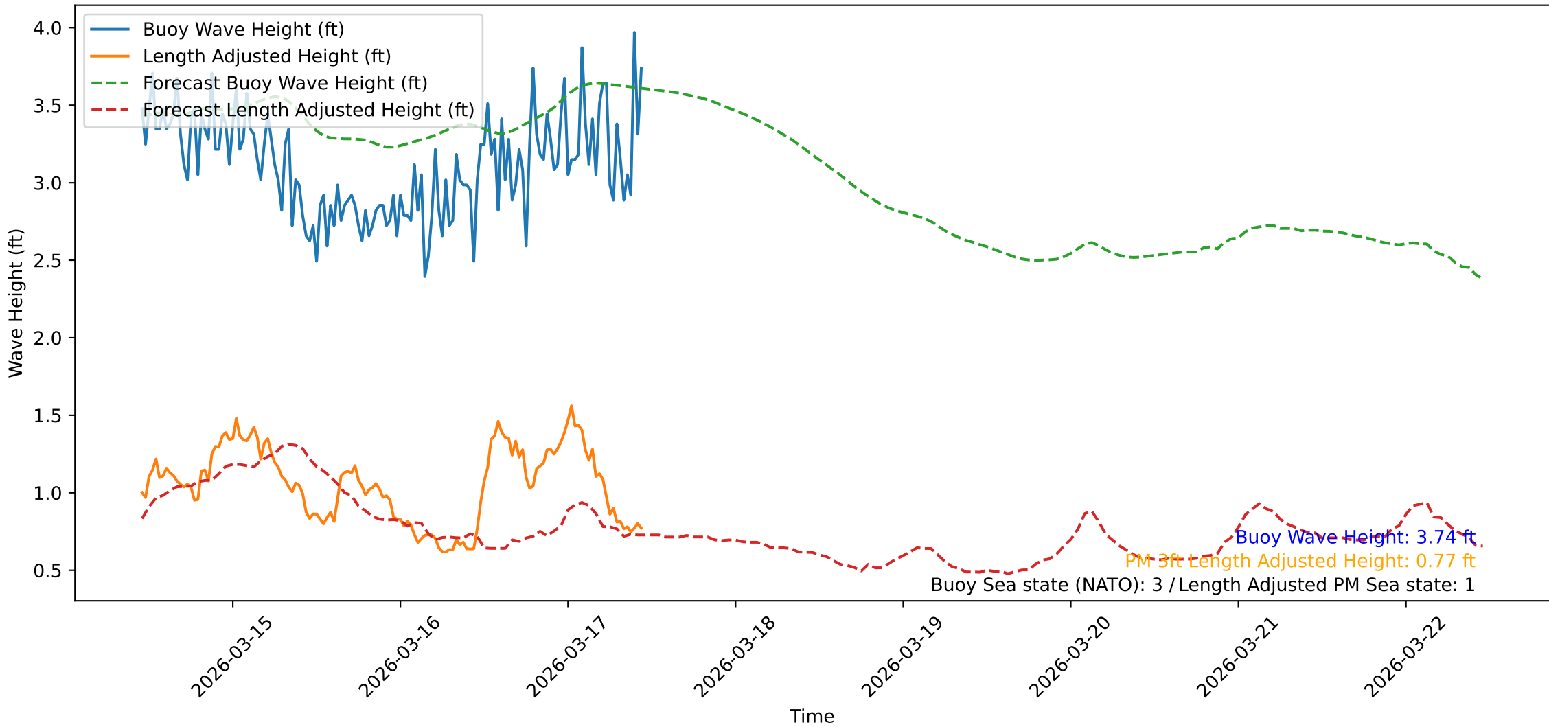
Wave Heights over Time for Oceanside Harbor at 2026-03-17 11:10:43
