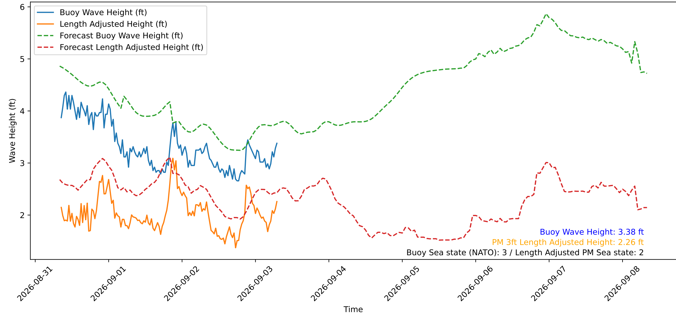
Wave Heights over Time for Green Beach at 2026-09-03 08:01:12
