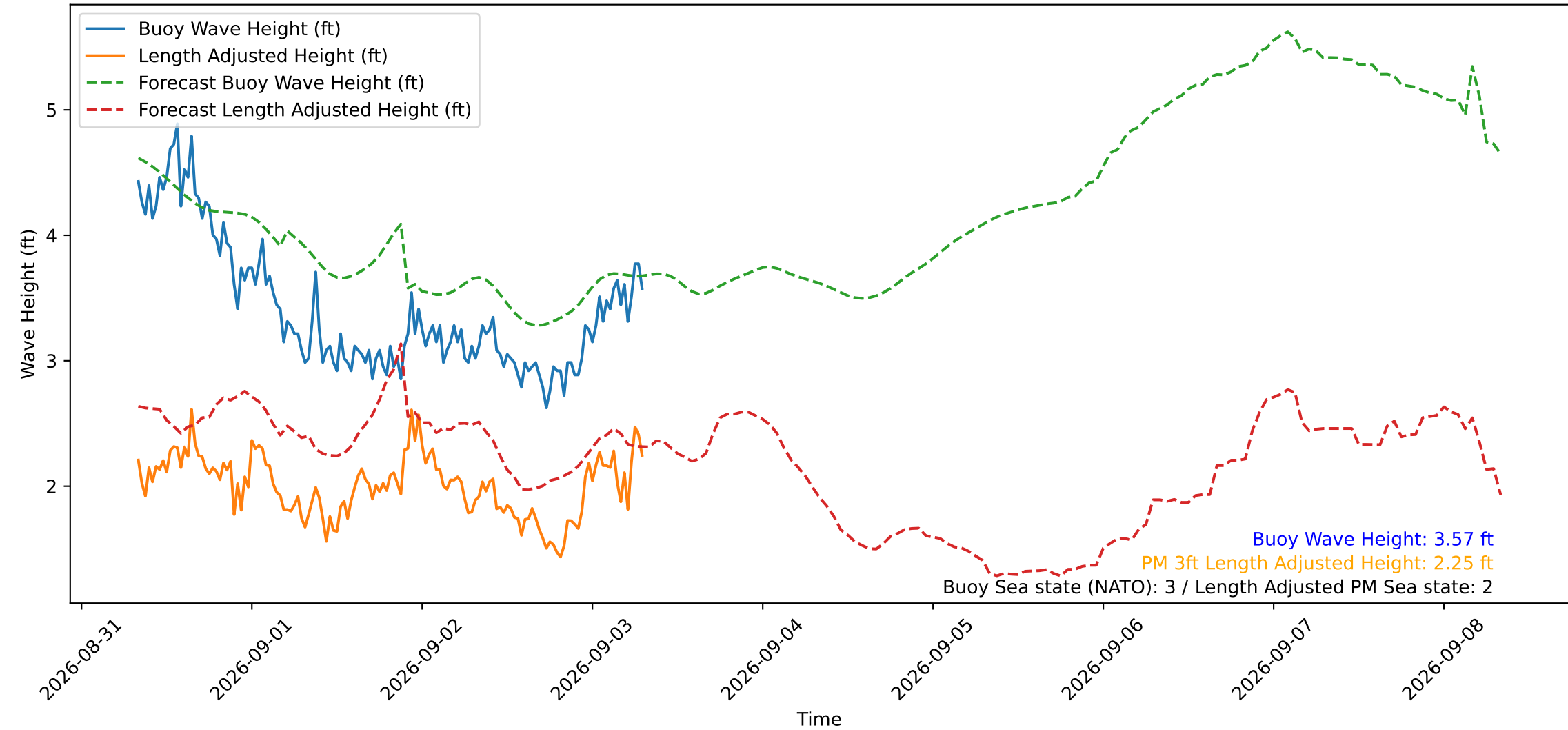
Wave Heights over Time for Oceanside Harbor at 2026-09-03 08:00:30
