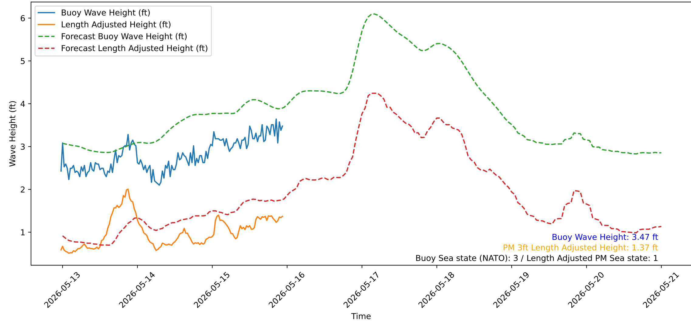
Wave Heights over Time for Green Beach at 2026-05-15 23:31:14
