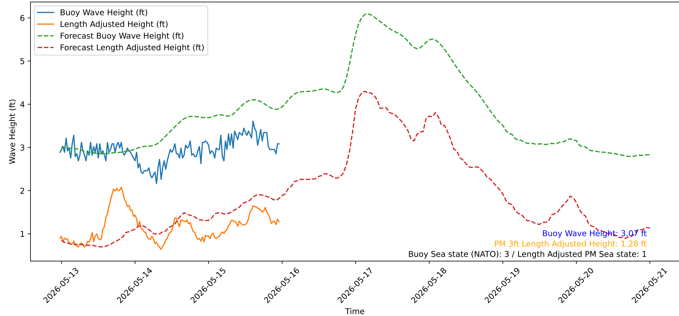
Wave Heights over Time for Oceanside Harbor at 2026-05-15 23:30:32
