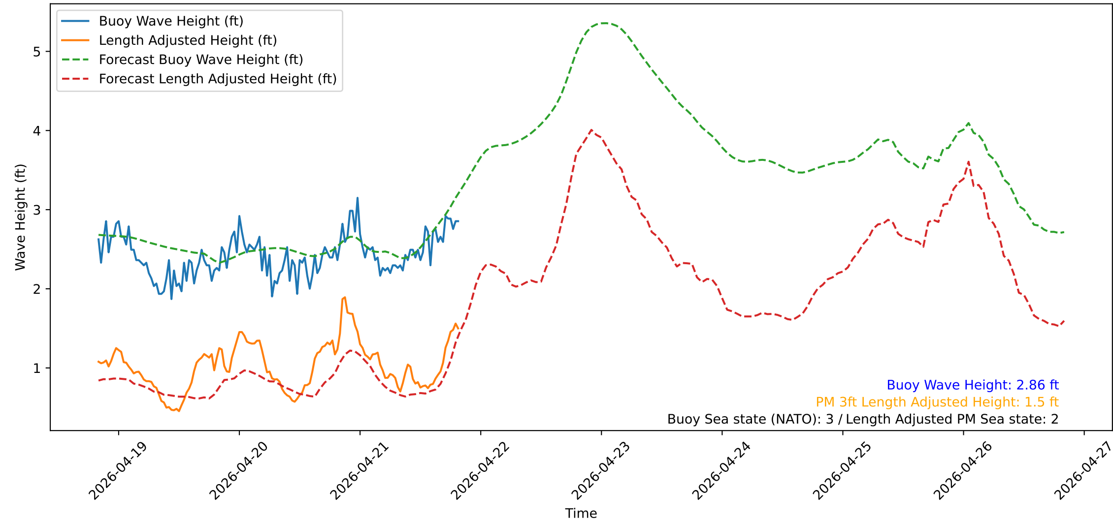
Wave Heights over Time for Green Beach at 2026-04-21 20:11:13
