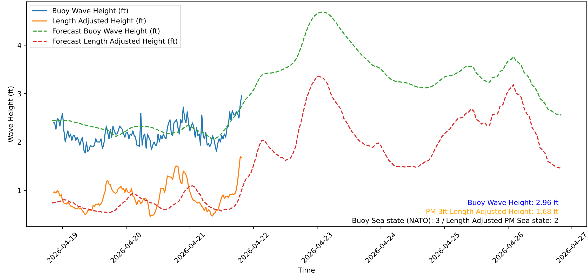
Wave Heights over Time for Red Beach at 2026-04-21 20:10:51
