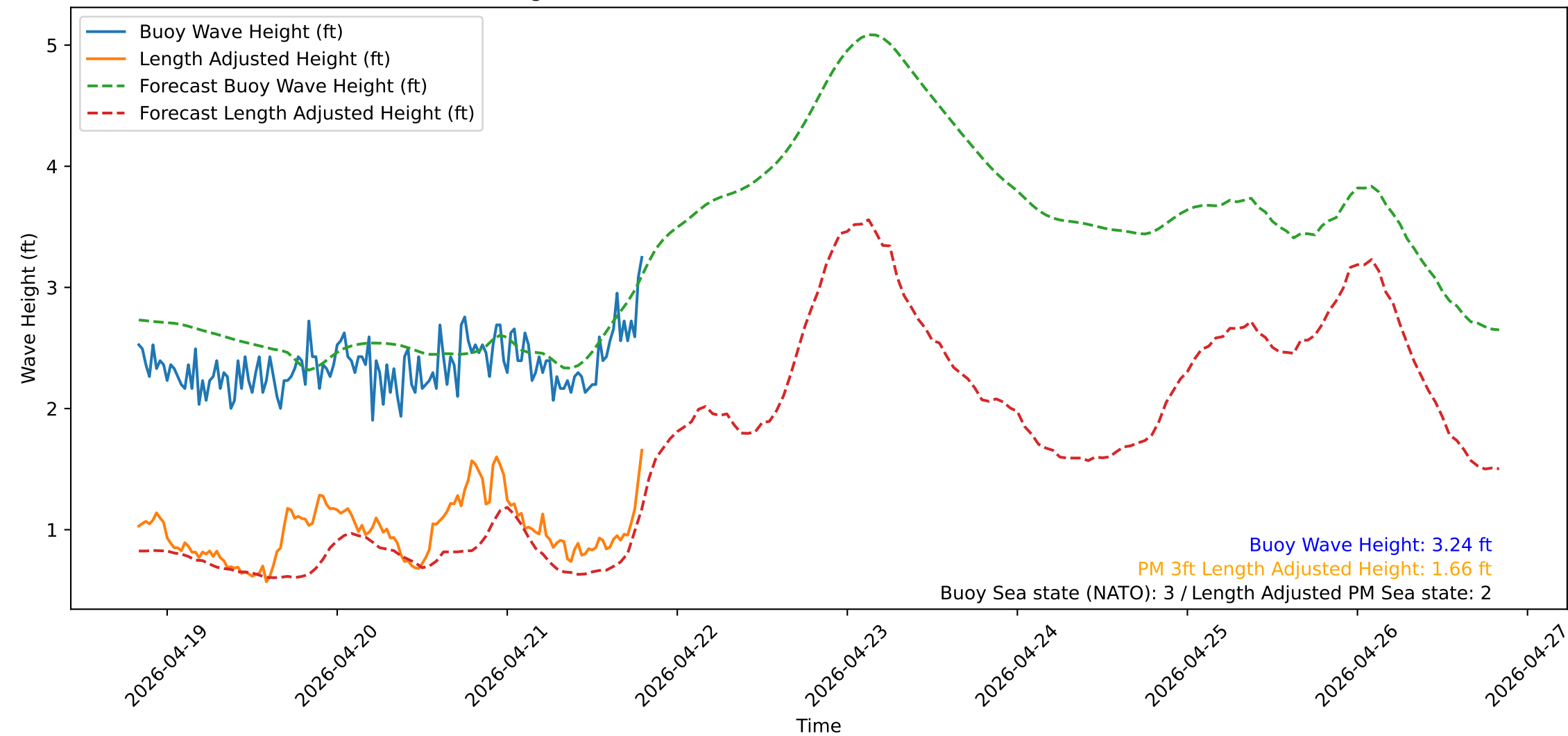
Wave Heights over Time for Oceanside Harbor at 2026-04-21 20:10:32
