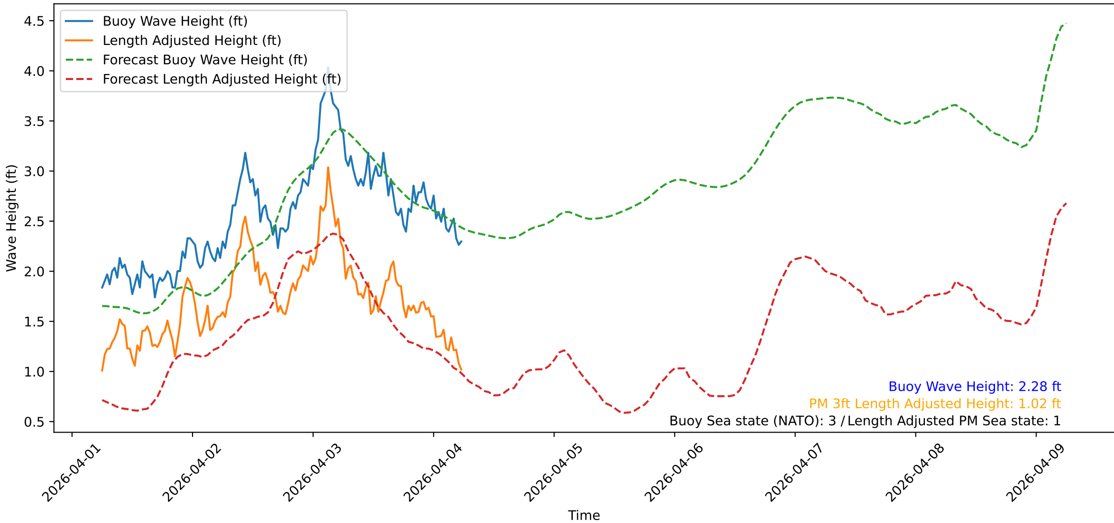
Wave Heights over Time for Oceanside Harbor at 2026-04-04 06:00:31
