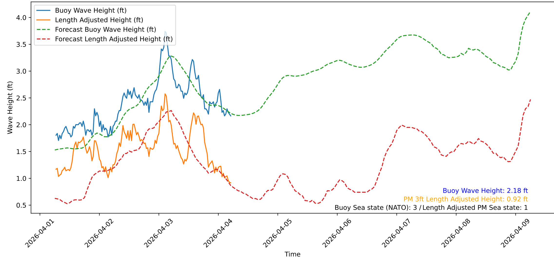
Wave Heights over Time for Red Beach at 2026-04-04 06:00:47
