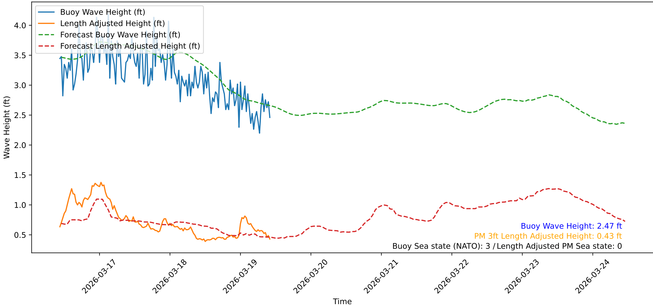
Wave Heights over Time for Green Beach at 2026-03-19 10:41:11
