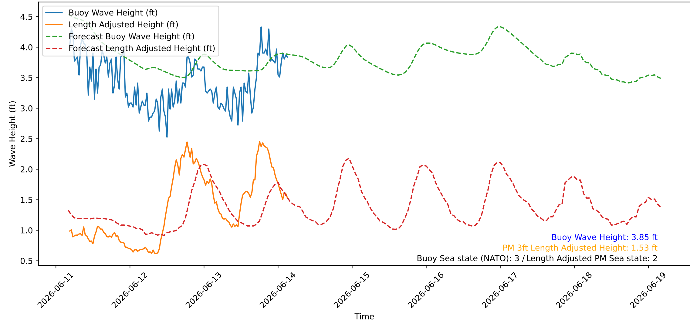
Wave Heights over Time for Red Beach at 2026-06-14 04:00:46
