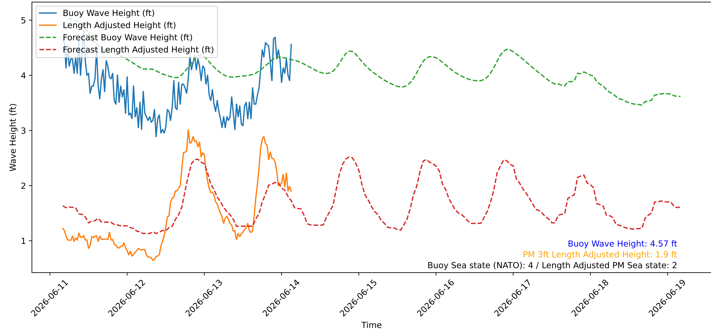
Wave Heights over Time for Green Beach at 2026-06-14 04:01:09
