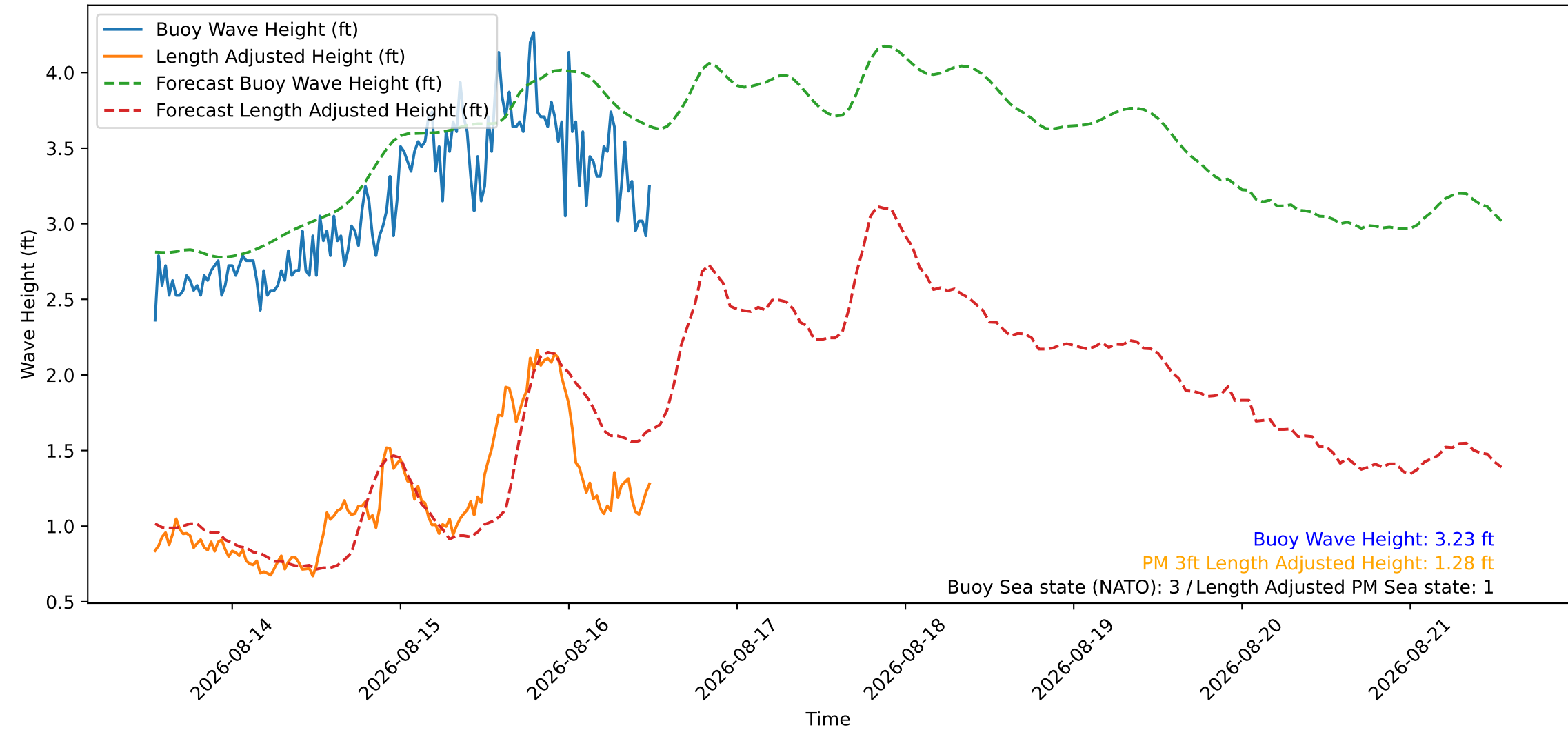
Wave Heights over Time for Green Beach at 2026-08-16 12:31:08
