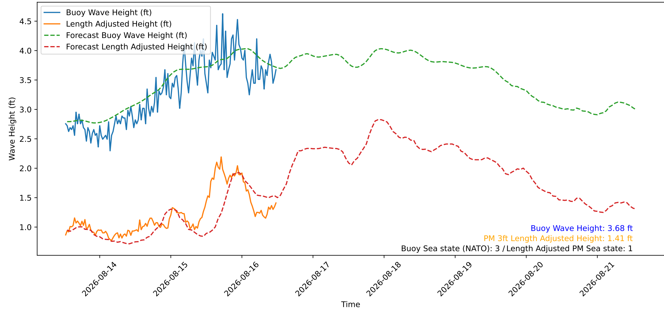
Wave Heights over Time for Oceanside Harbor at 2026-08-16 12:30:26
