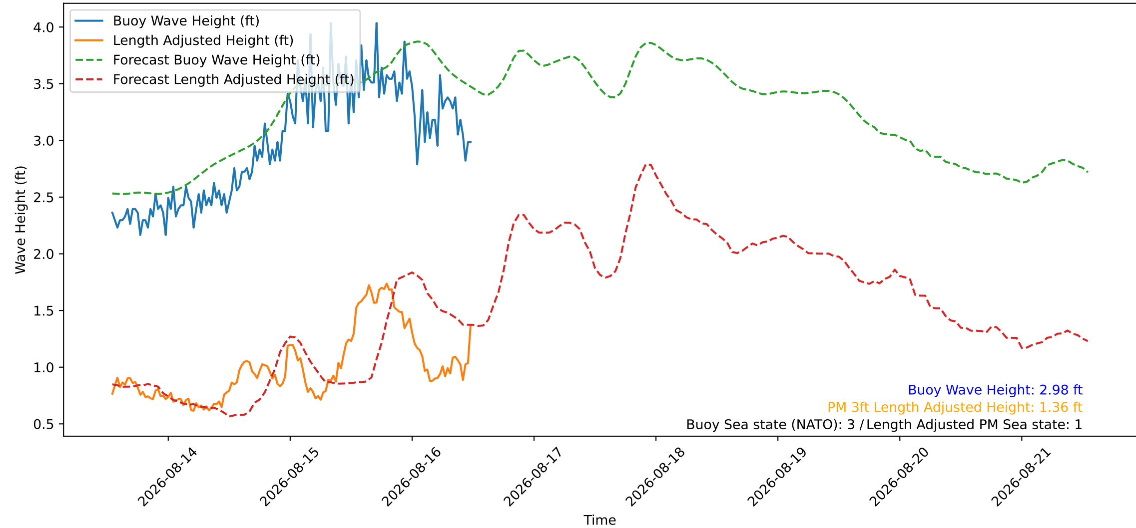
Wave Heights over Time for Red Beach at 2026-08-16 12:30:45
