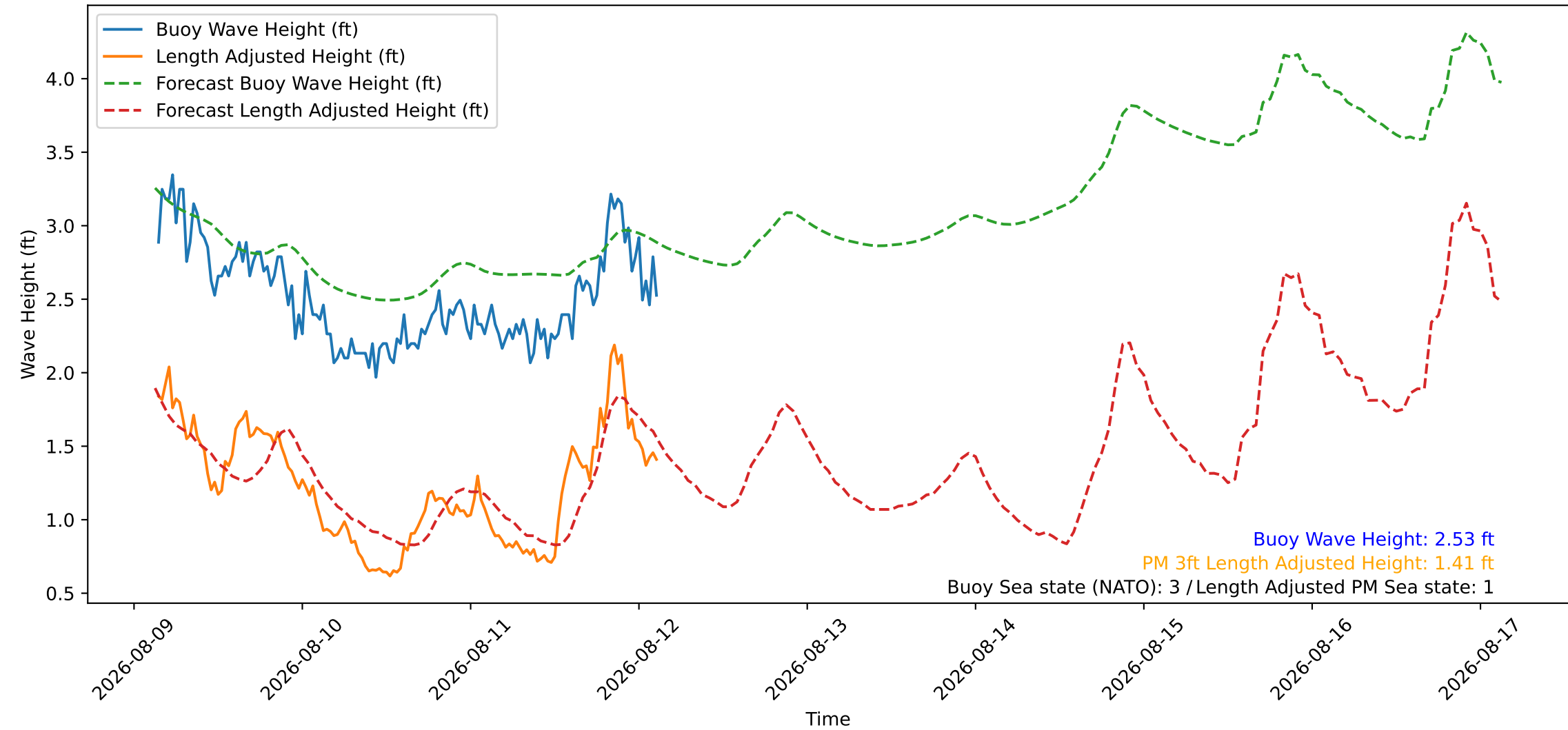
Wave Heights over Time for Green Beach at 2026-08-12 03:21:09
