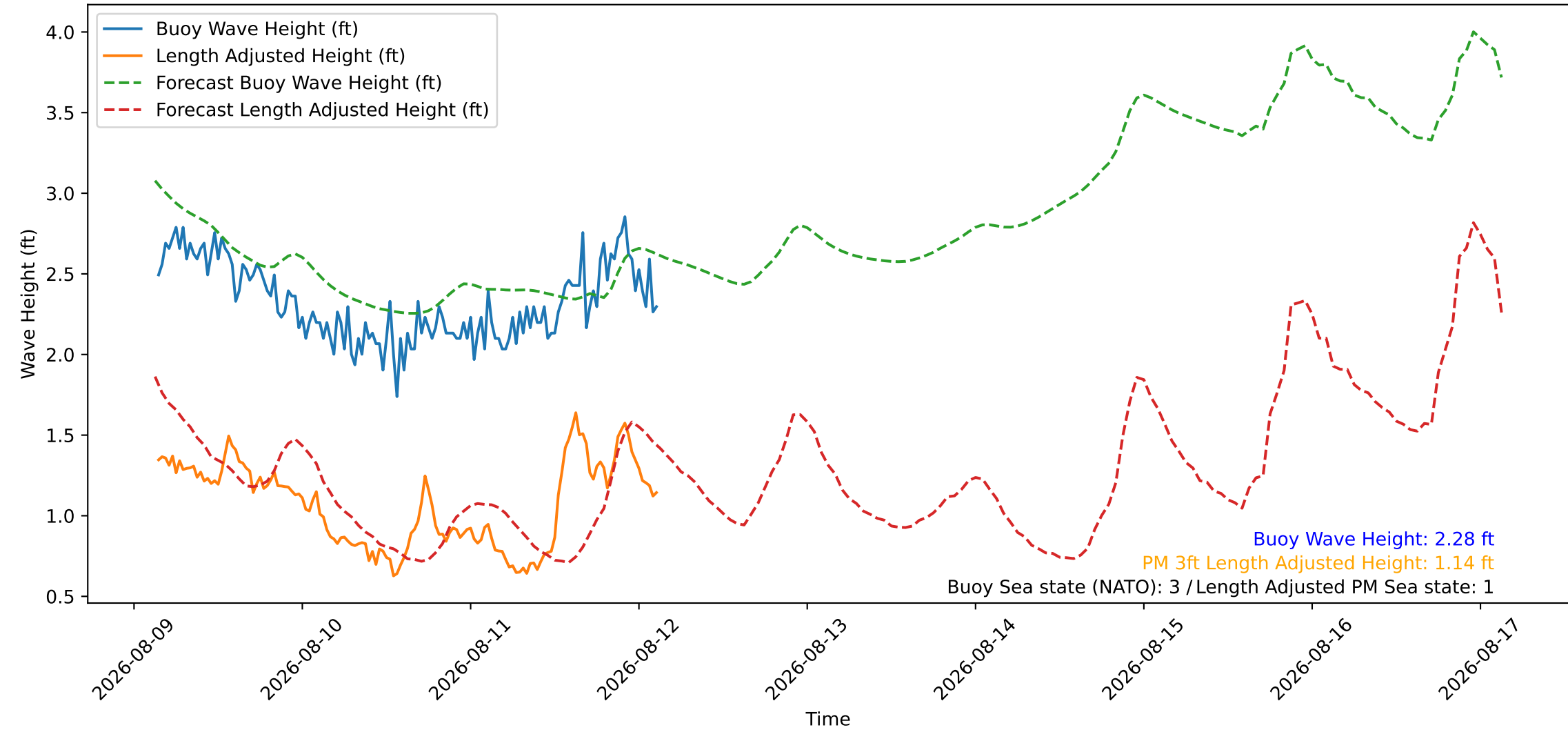
Wave Heights over Time for Red Beach at 2026-08-12 03:20:47
