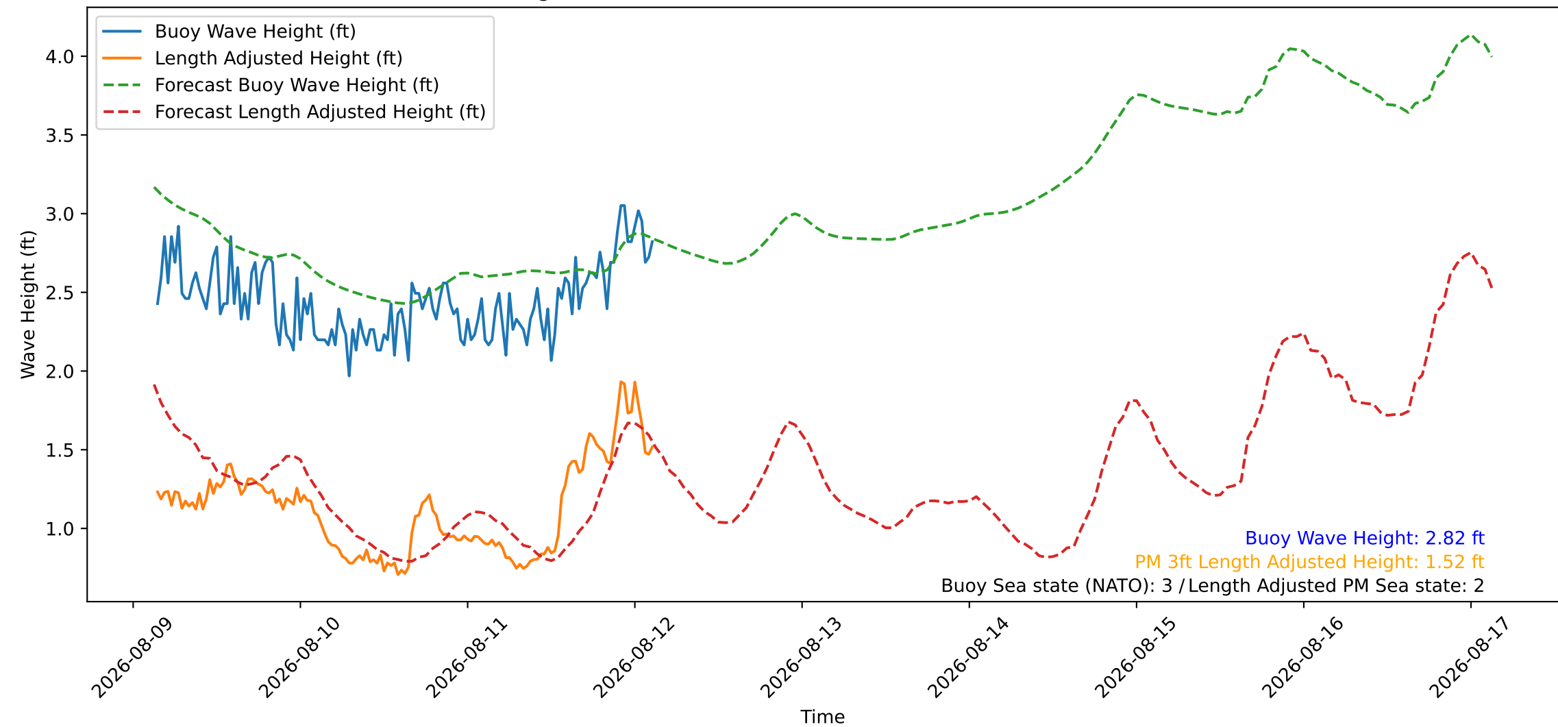
Wave Heights over Time for Oceanside Harbor at 2026-08-12 03:20:26
