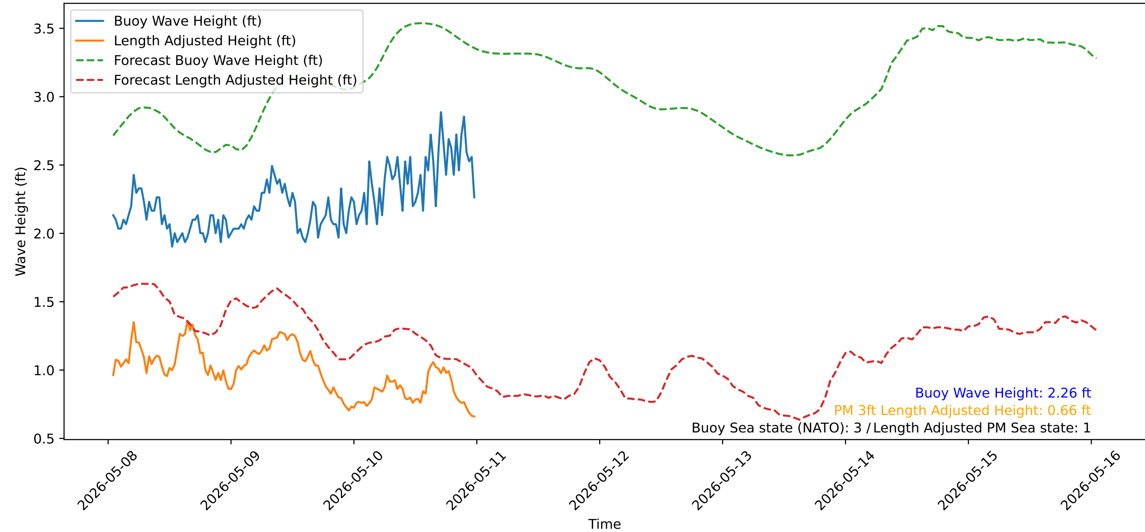
Wave Heights over Time for Red Beach at 2026-05-11 00:30:55
