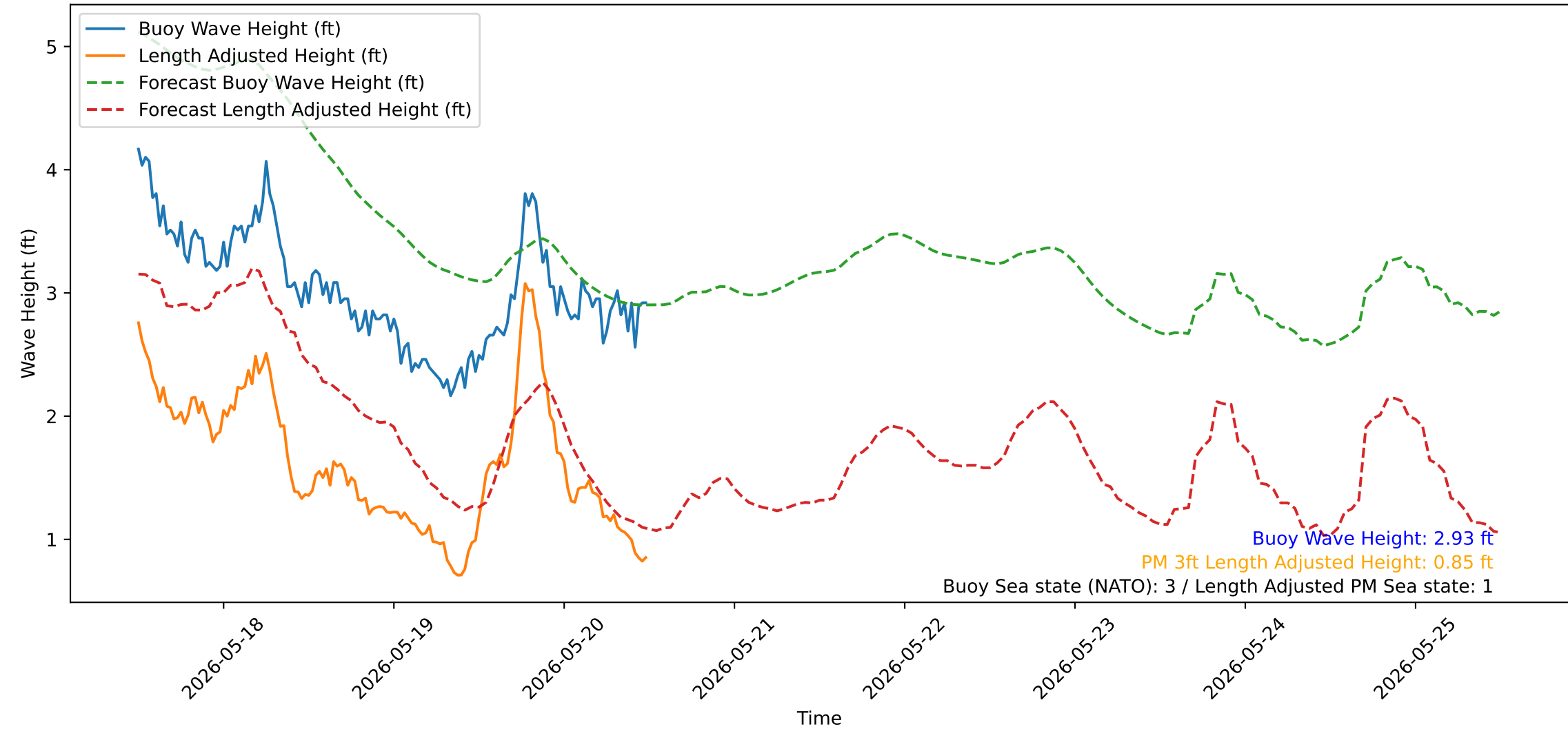
Wave Heights over Time for Green Beach at 2026-05-20 12:11:14
