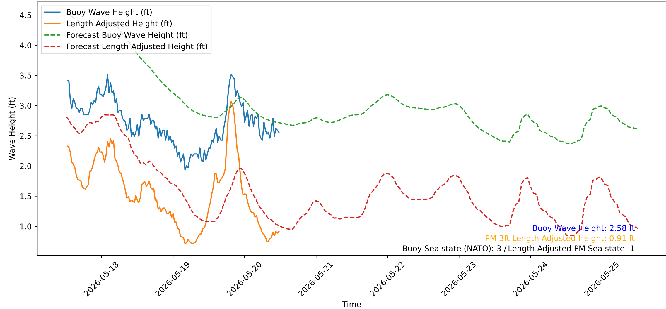
Wave Heights over Time for Red Beach at 2026-05-20 12:10:52
