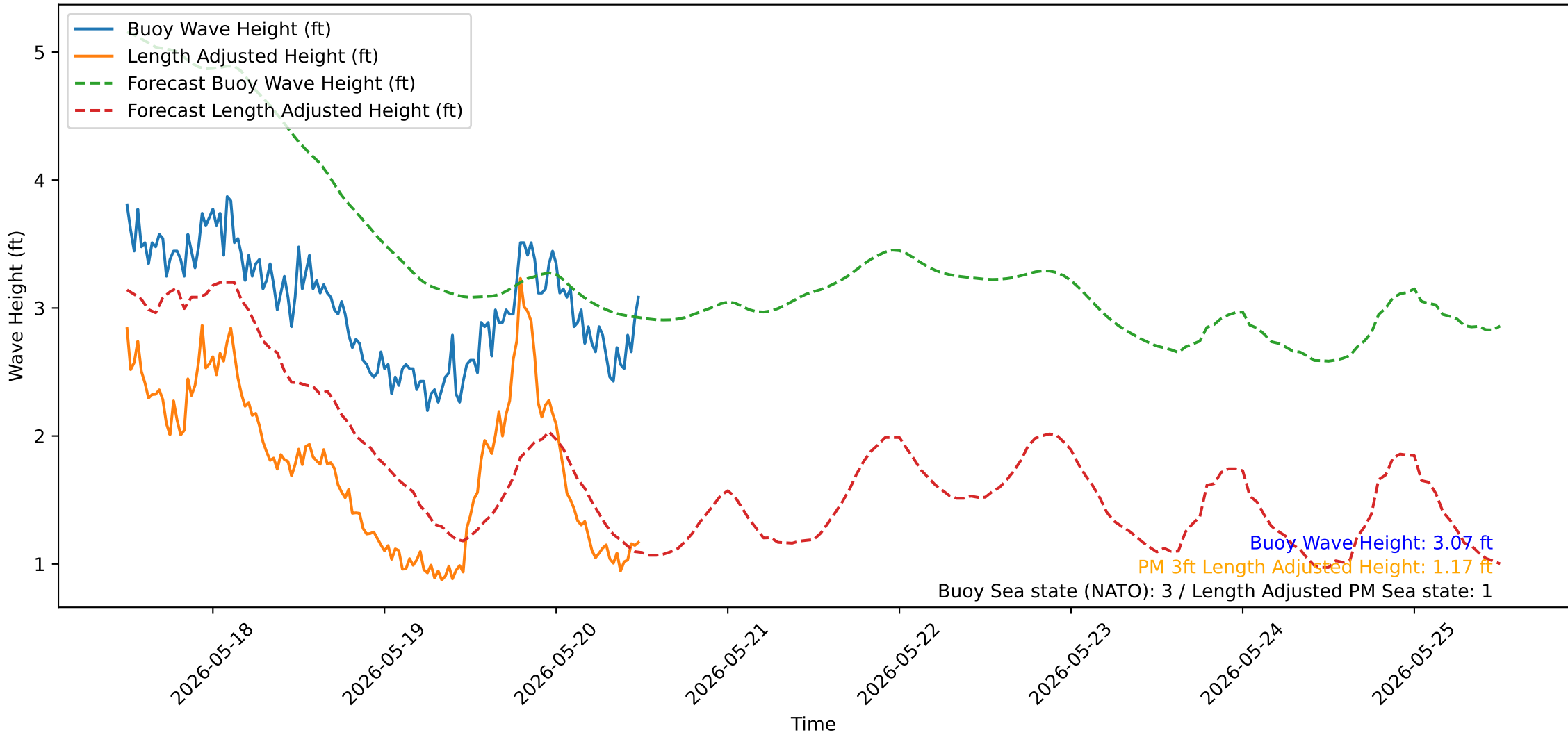
Wave Heights over Time for Oceanside Harbor at 2026-05-20 12:10:32
