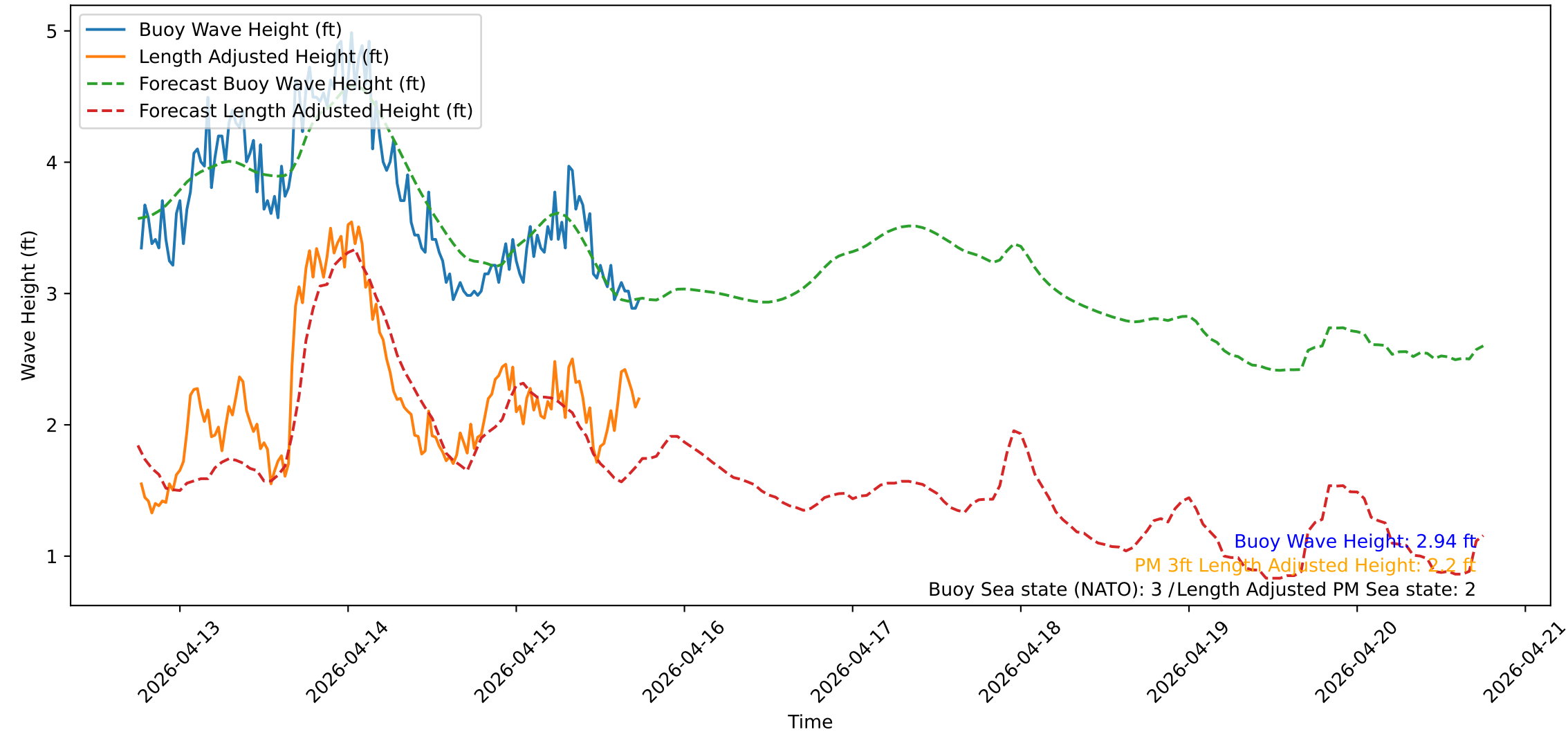
Wave Heights over Time for Green Beach at 2026-04-15 18:21:14
