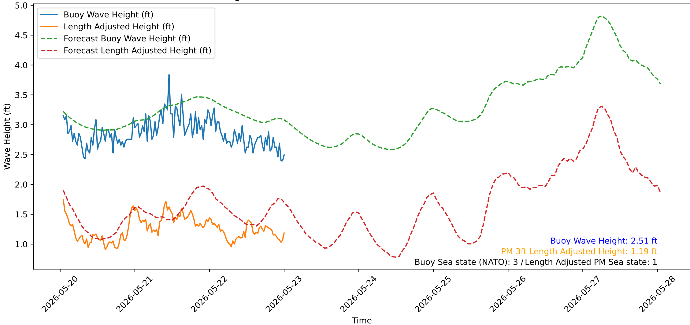
Wave Heights over Time for Oceanside Harbor at 2026-05-23 00:50:31
