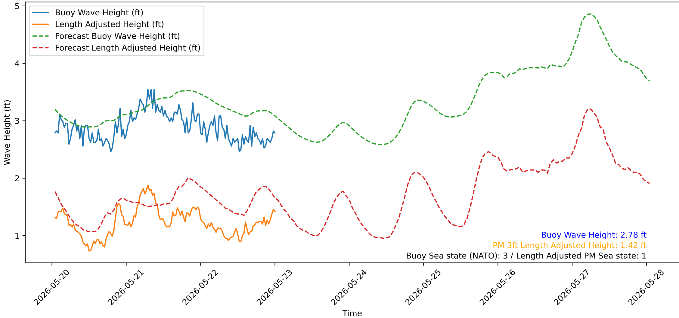
Wave Heights over Time for Green Beach at 2026-05-23 00:51:15
