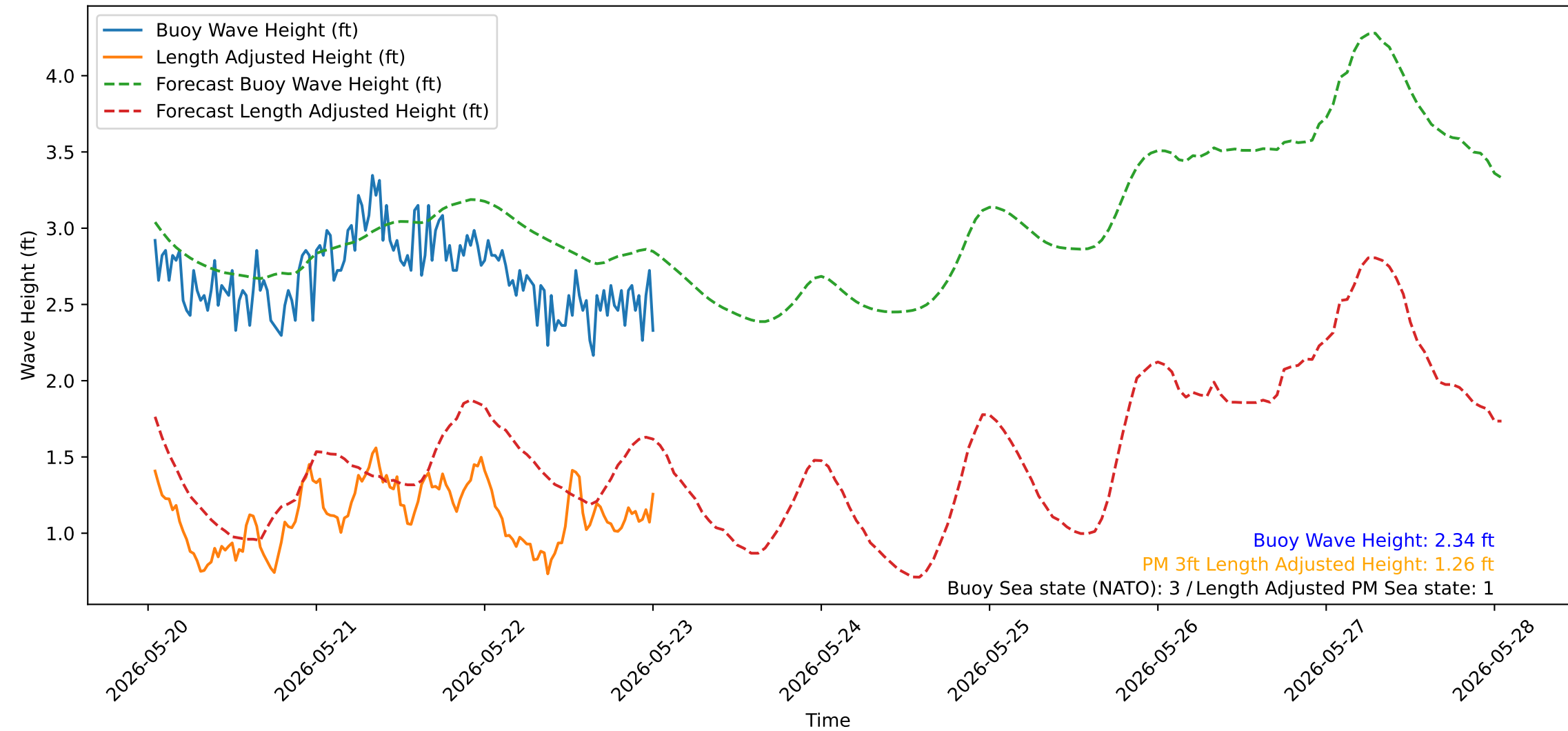
Wave Heights over Time for Red Beach at 2026-05-23 00:50:52
