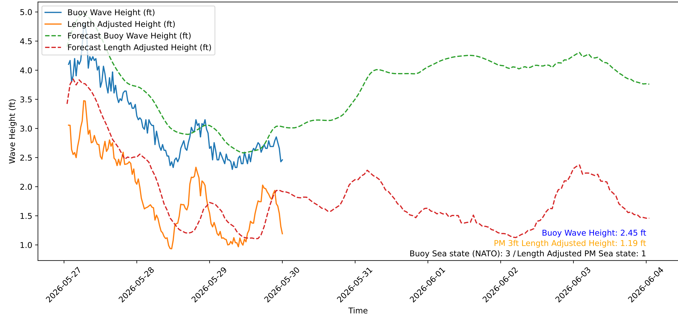
Wave Heights over Time for Red Beach at 2026-05-30 01:00:42
