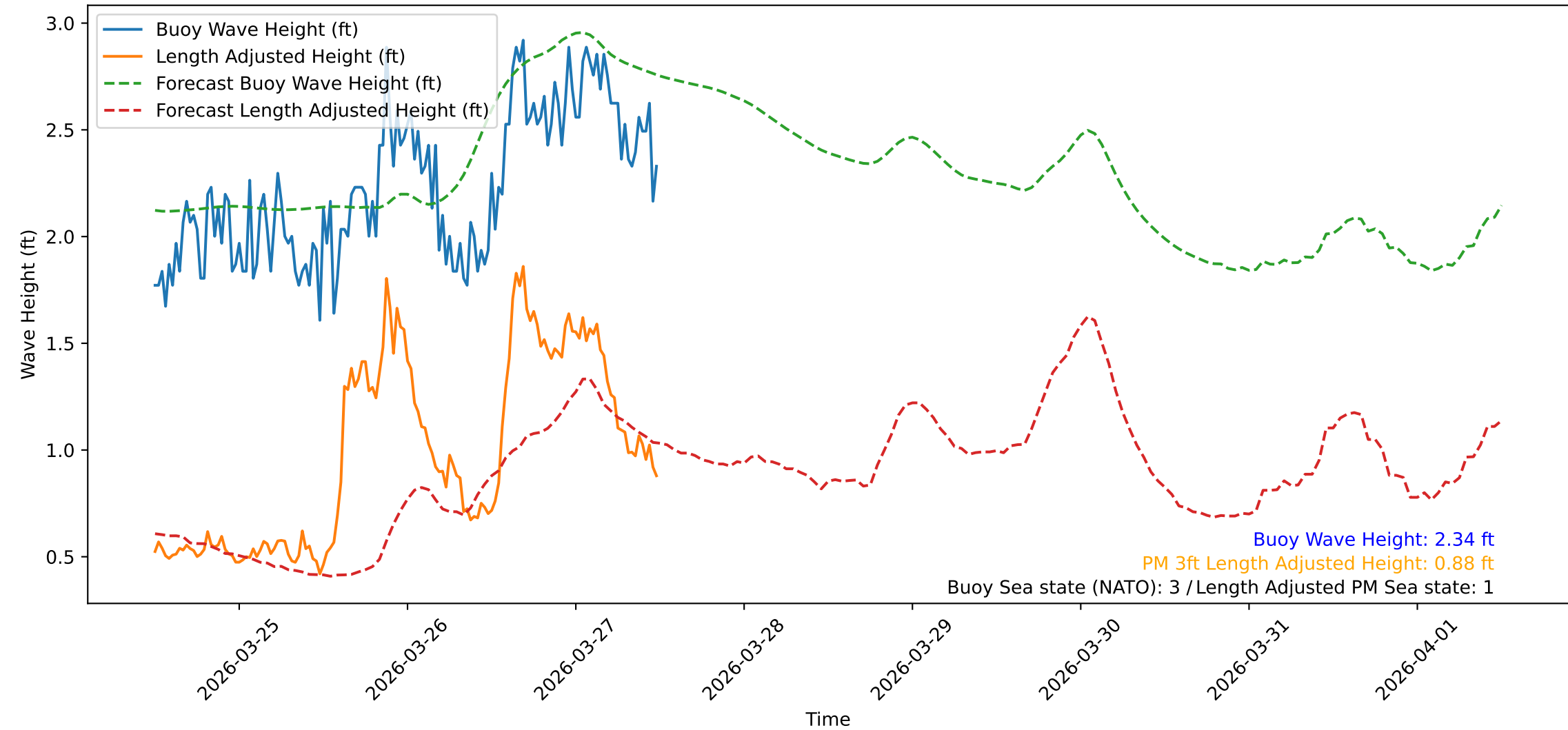
Wave Heights over Time for Oceanside Harbor at 2026-03-27 12:00:31
