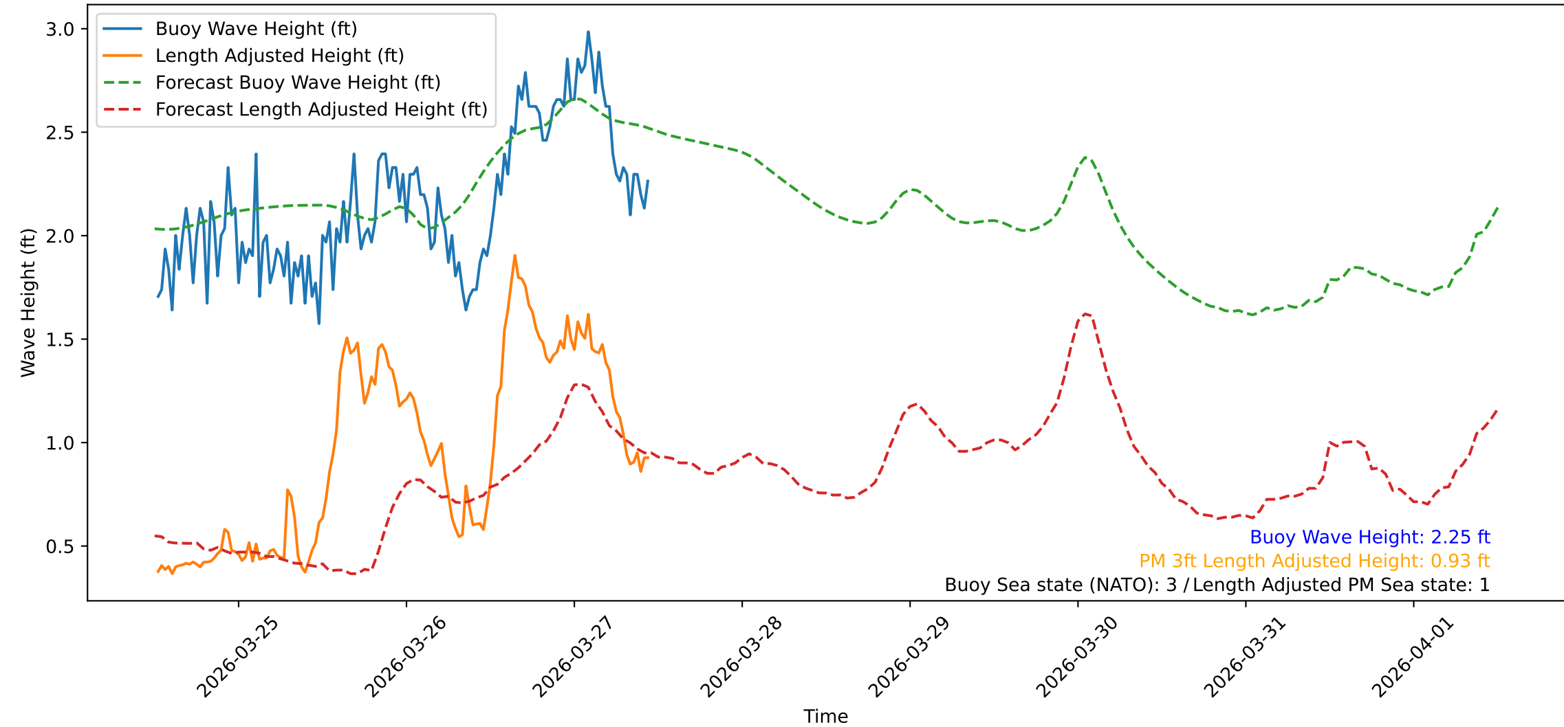
Wave Heights over Time for Red Beach at 2026-03-27 12:00:47
