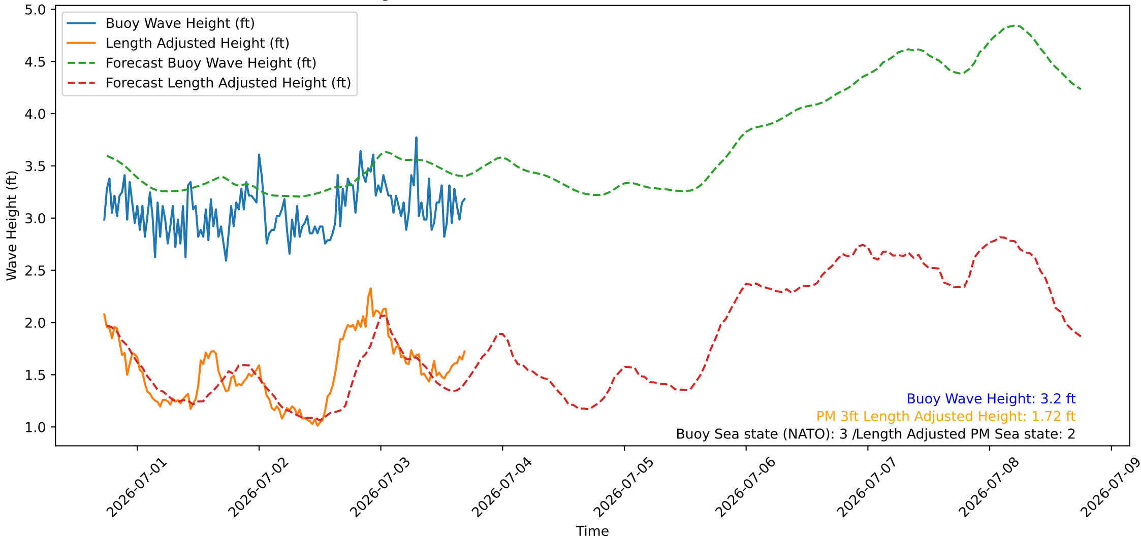
Wave Heights over Time for Oceanside Harbor at 2026-07-03 17:30:27
