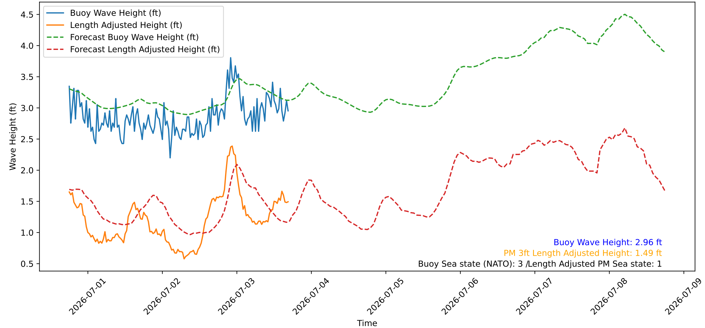
Wave Heights over Time for Red Beach at 2026-07-03 17:30:46
