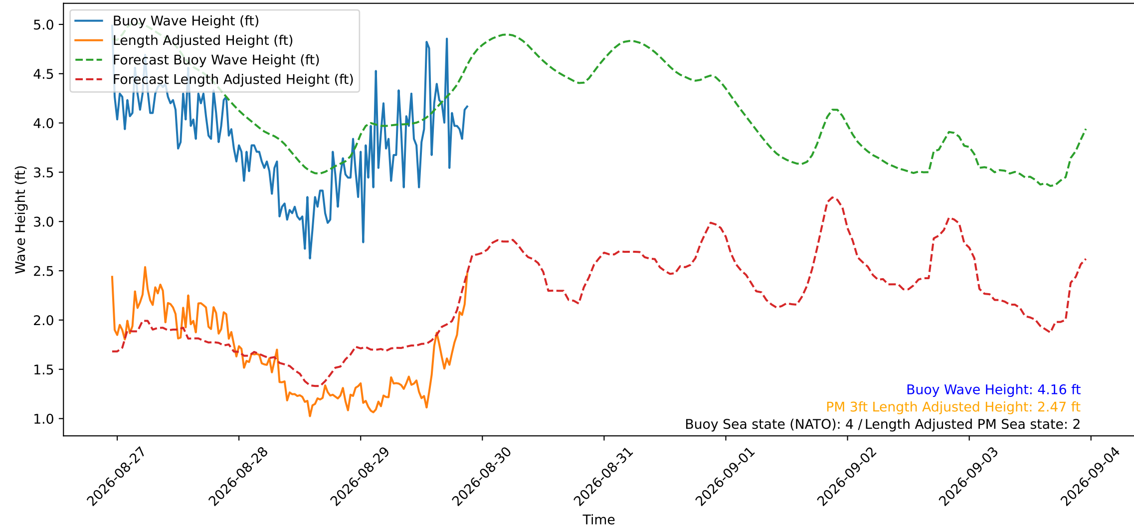
Wave Heights over Time for Green Beach at 2026-08-29 22:31:11
