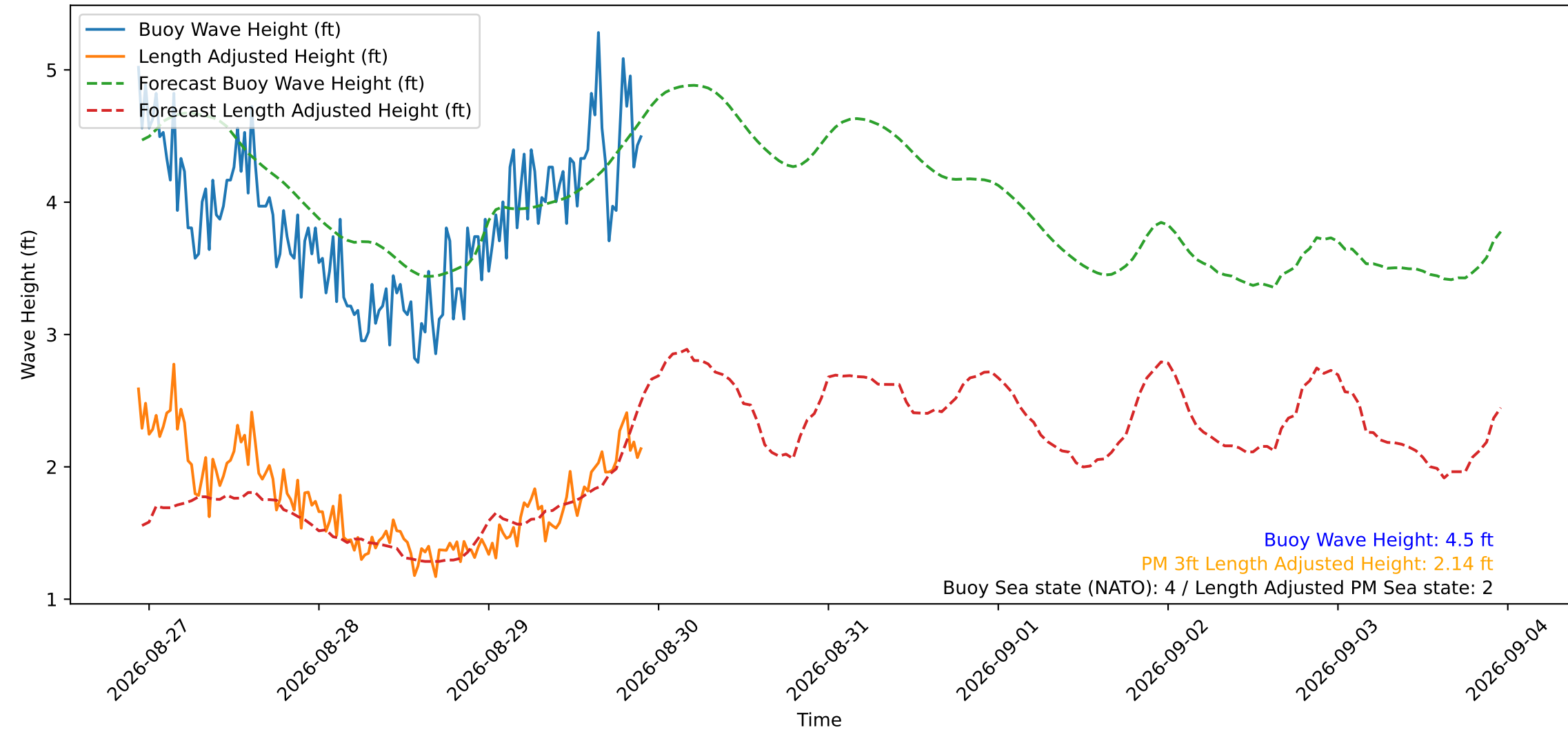
Wave Heights over Time for Oceanside Harbor at 2026-08-29 22:30:30
