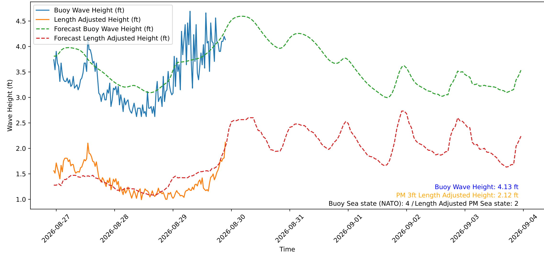
Wave Heights over Time for Red Beach at 2026-08-29 22:30:49
