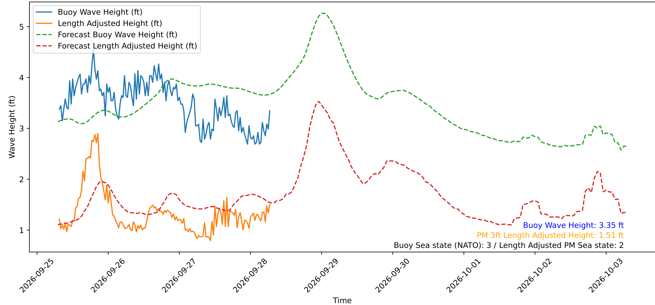
Wave Heights over Time for Green Beach at 2026-09-28 07:11:12
