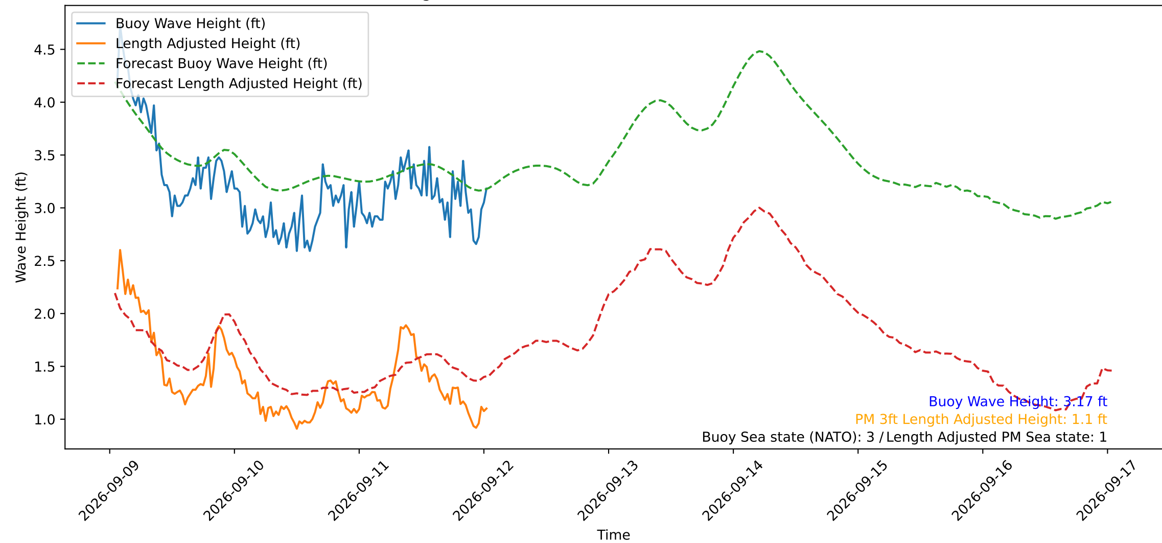
Wave Heights over Time for Green Beach at 2026-09-12 01:11:12
