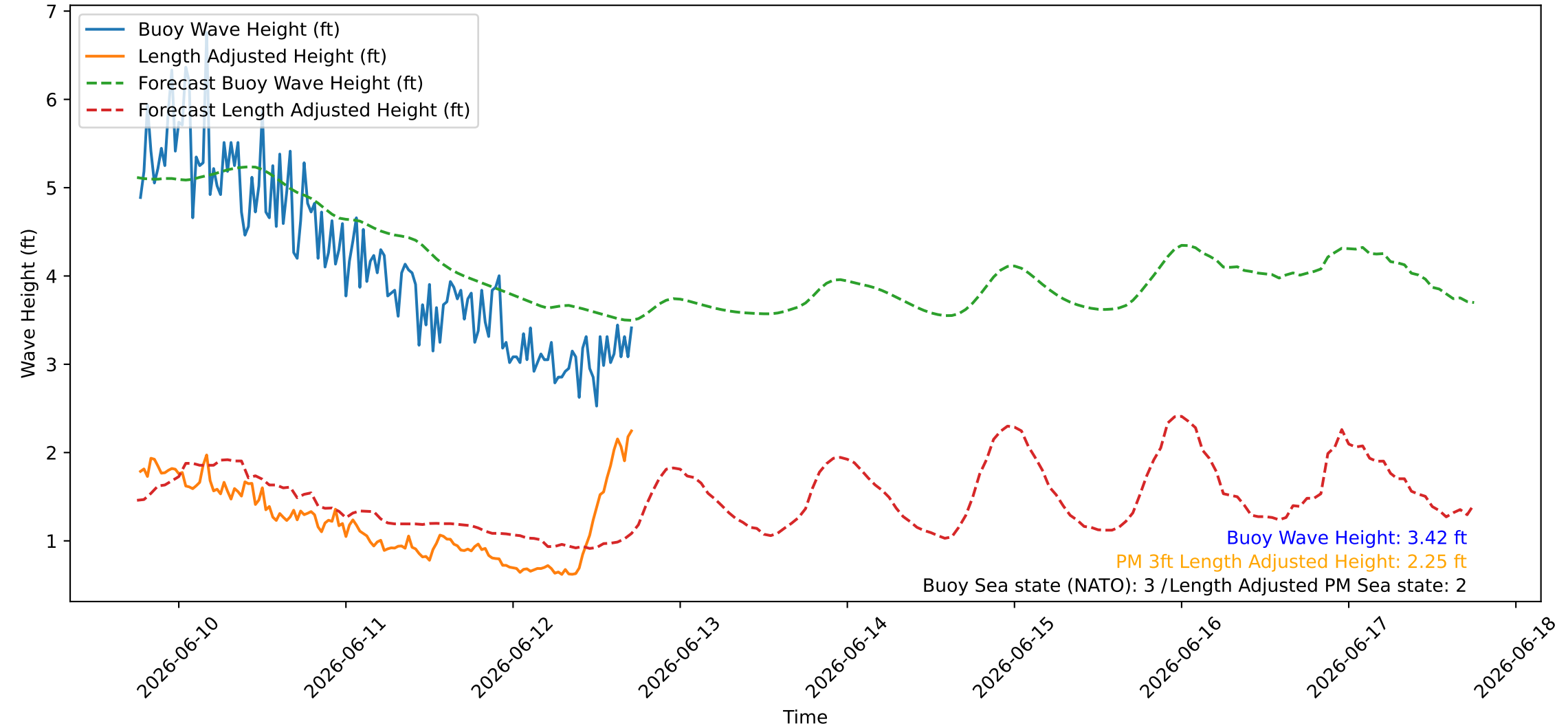
Wave Heights over Time for Red Beach at 2026-06-12 18:20:47
