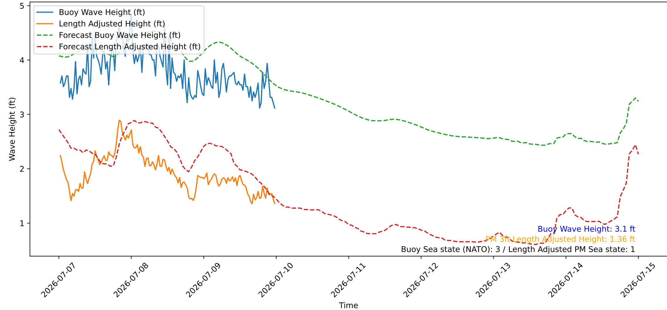
Wave Heights over Time for Red Beach at 2026-07-10 00:10:46
