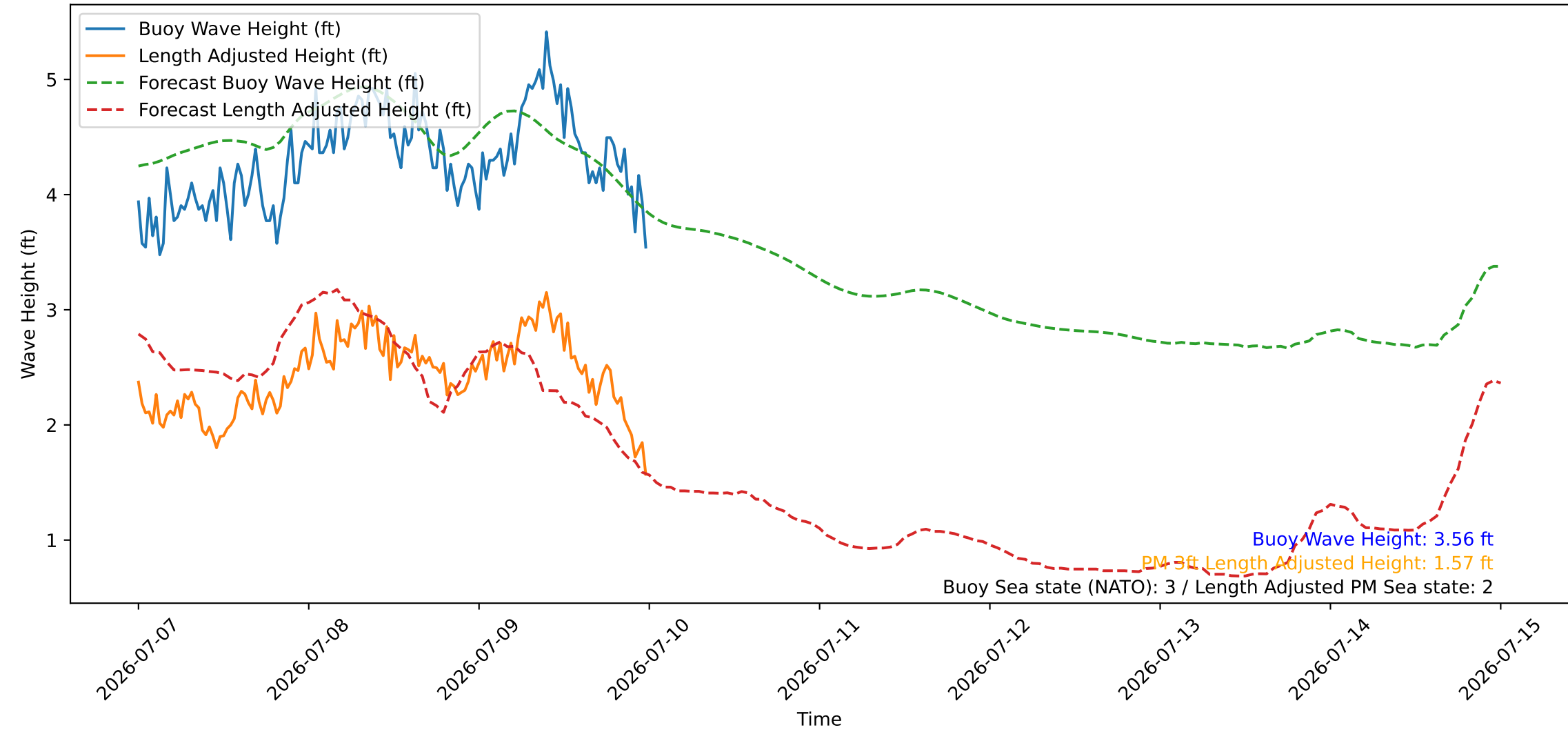
Wave Heights over Time for Oceanside Harbor at 2026-07-10 00:10:27
