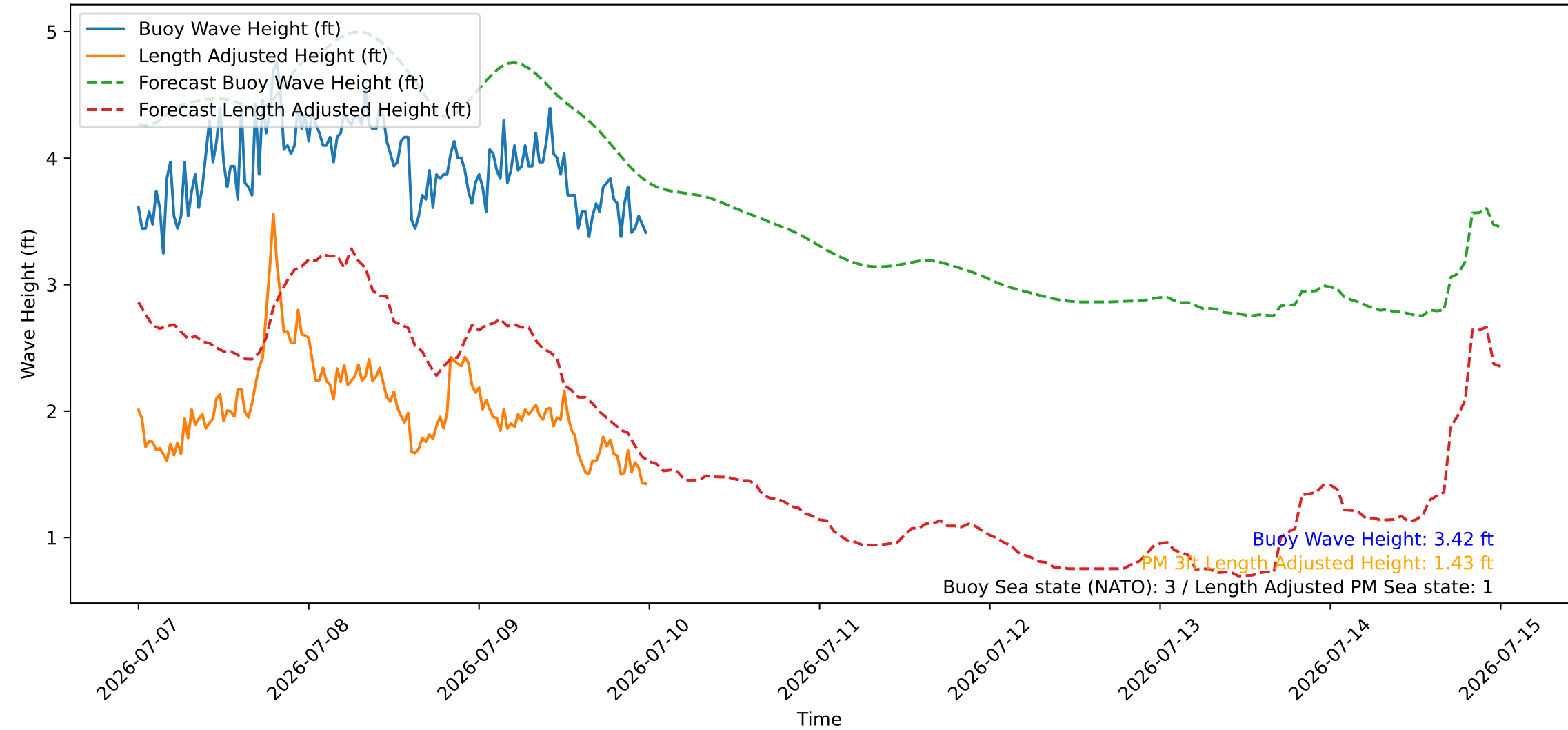
Wave Heights over Time for Green Beach at 2026-07-10 00:11:08
