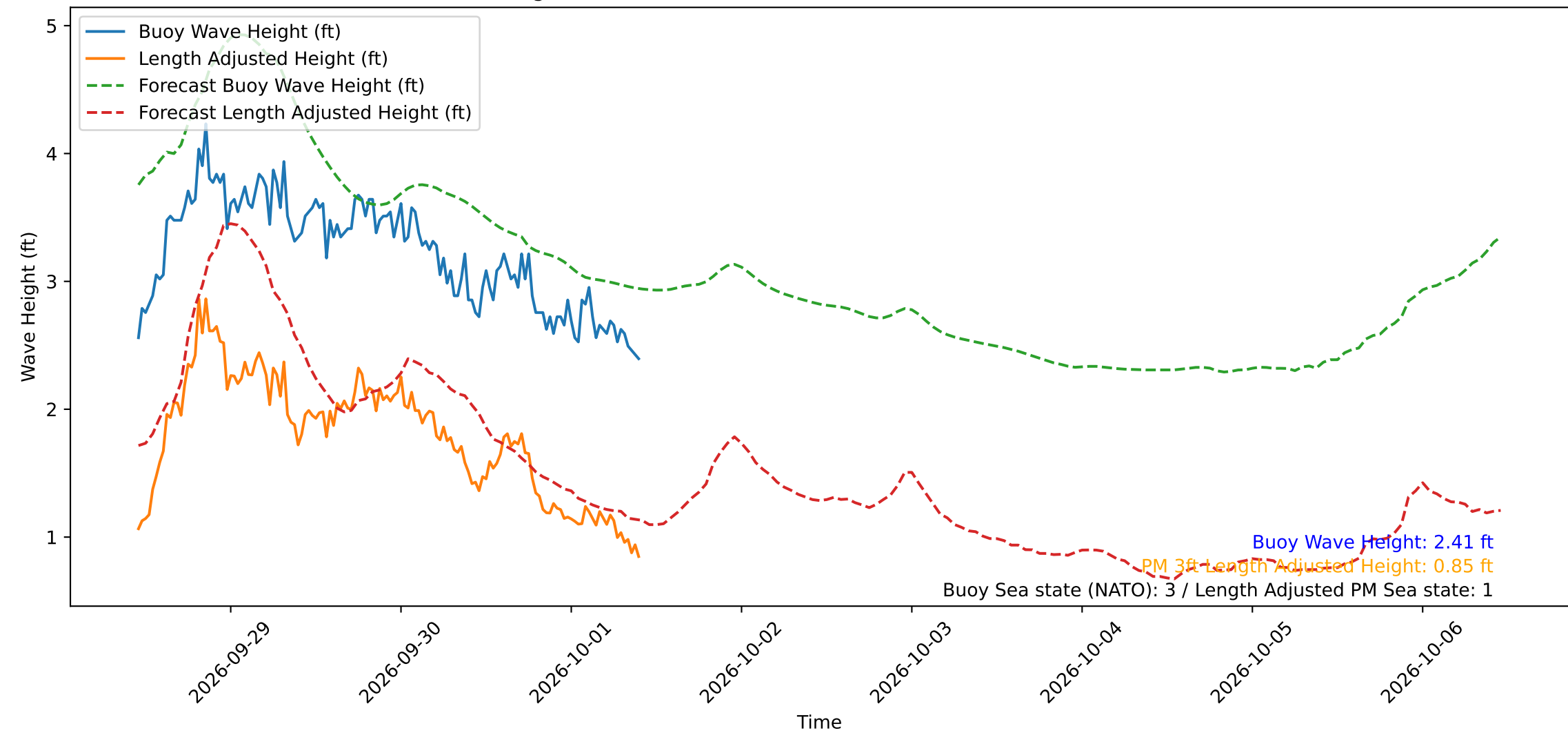
Wave Heights over Time for Oceanside Harbor at 2026-10-01 10:50:30
