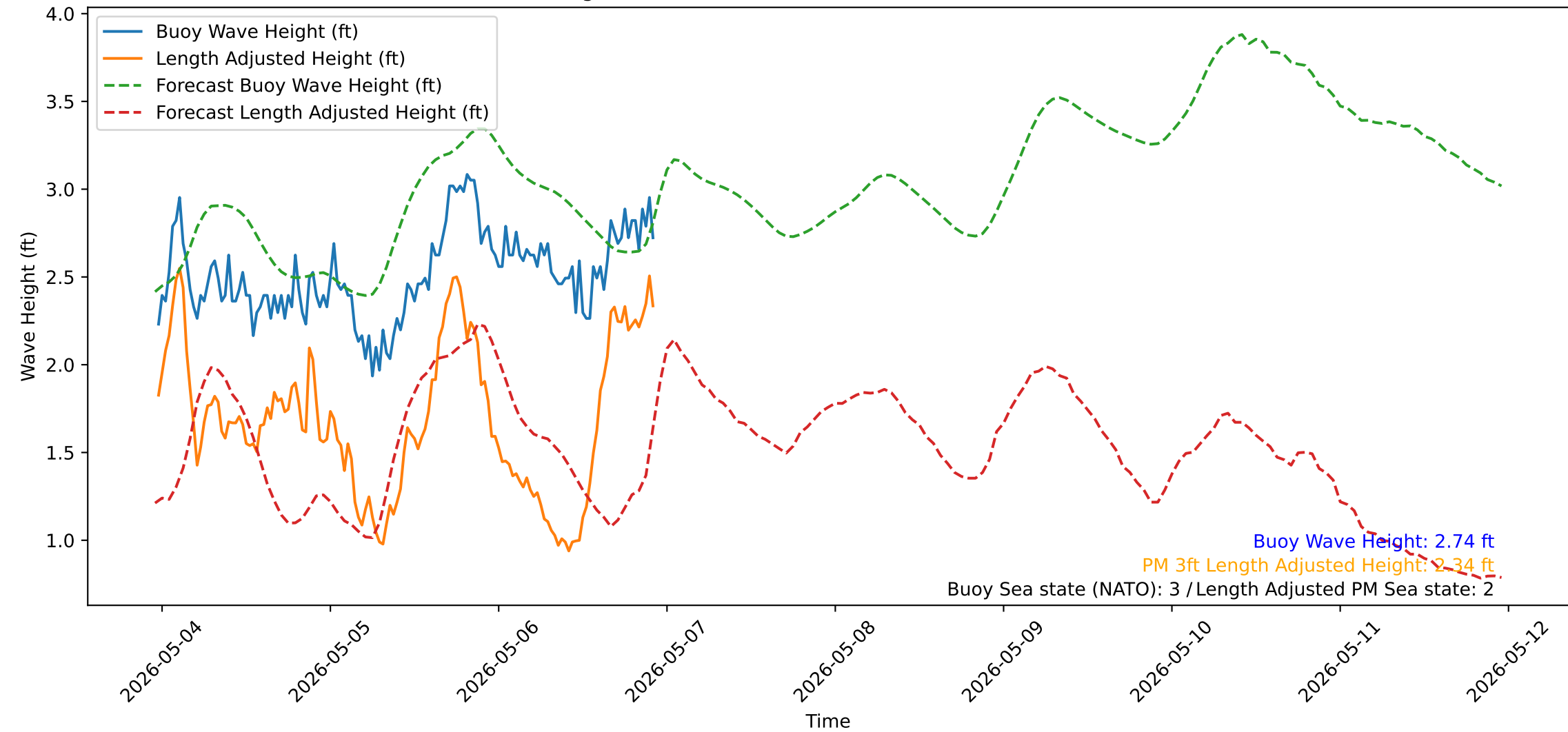
Wave Heights over Time for Red Beach at 2026-05-06 23:10:51
