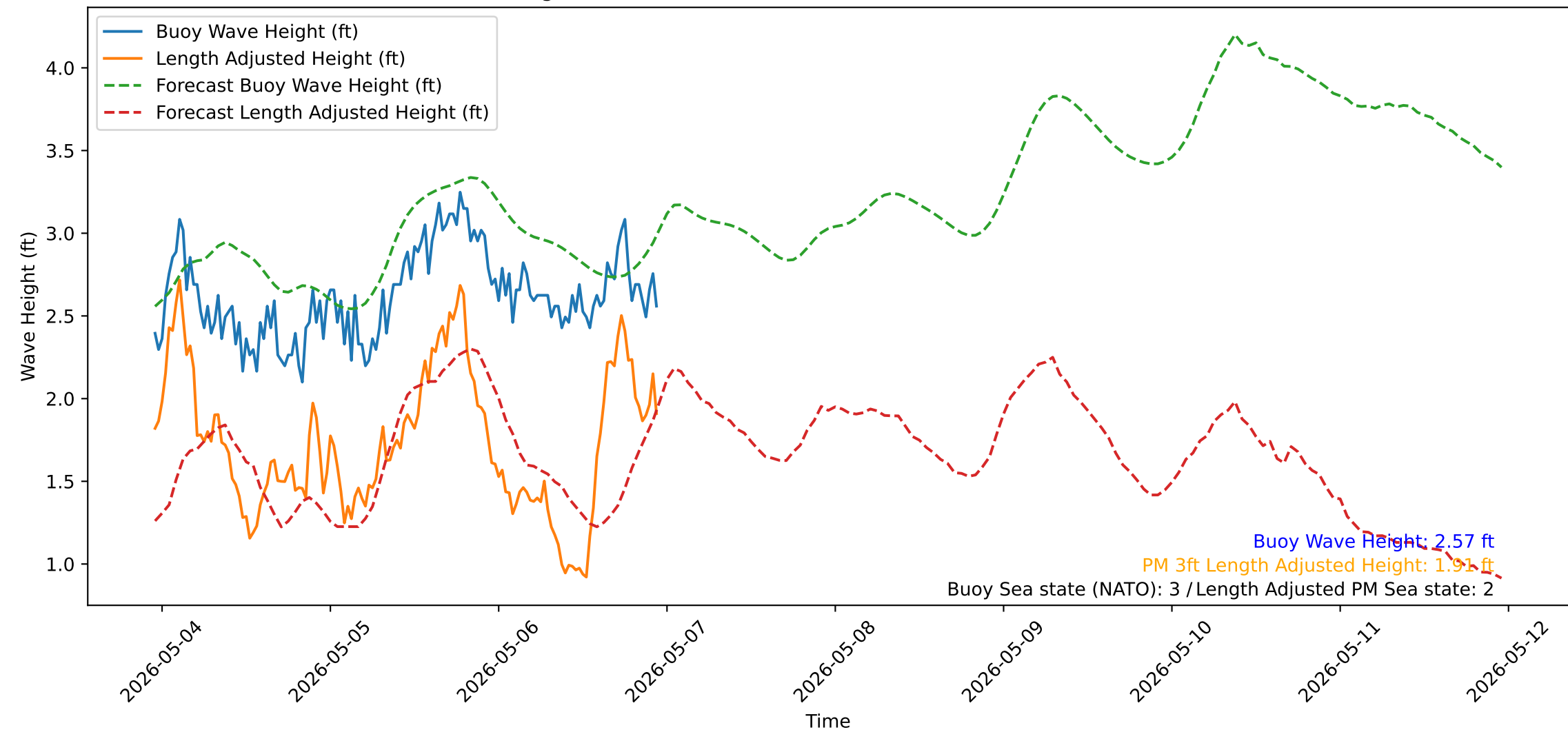
Wave Heights over Time for Oceanside Harbor at 2026-05-06 23:10:32
