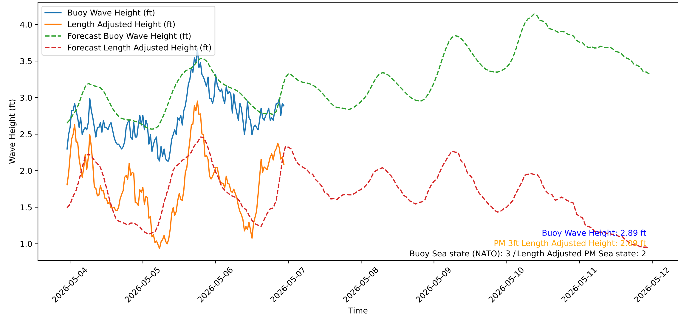
Wave Heights over Time for Green Beach at 2026-05-06 23:11:14
