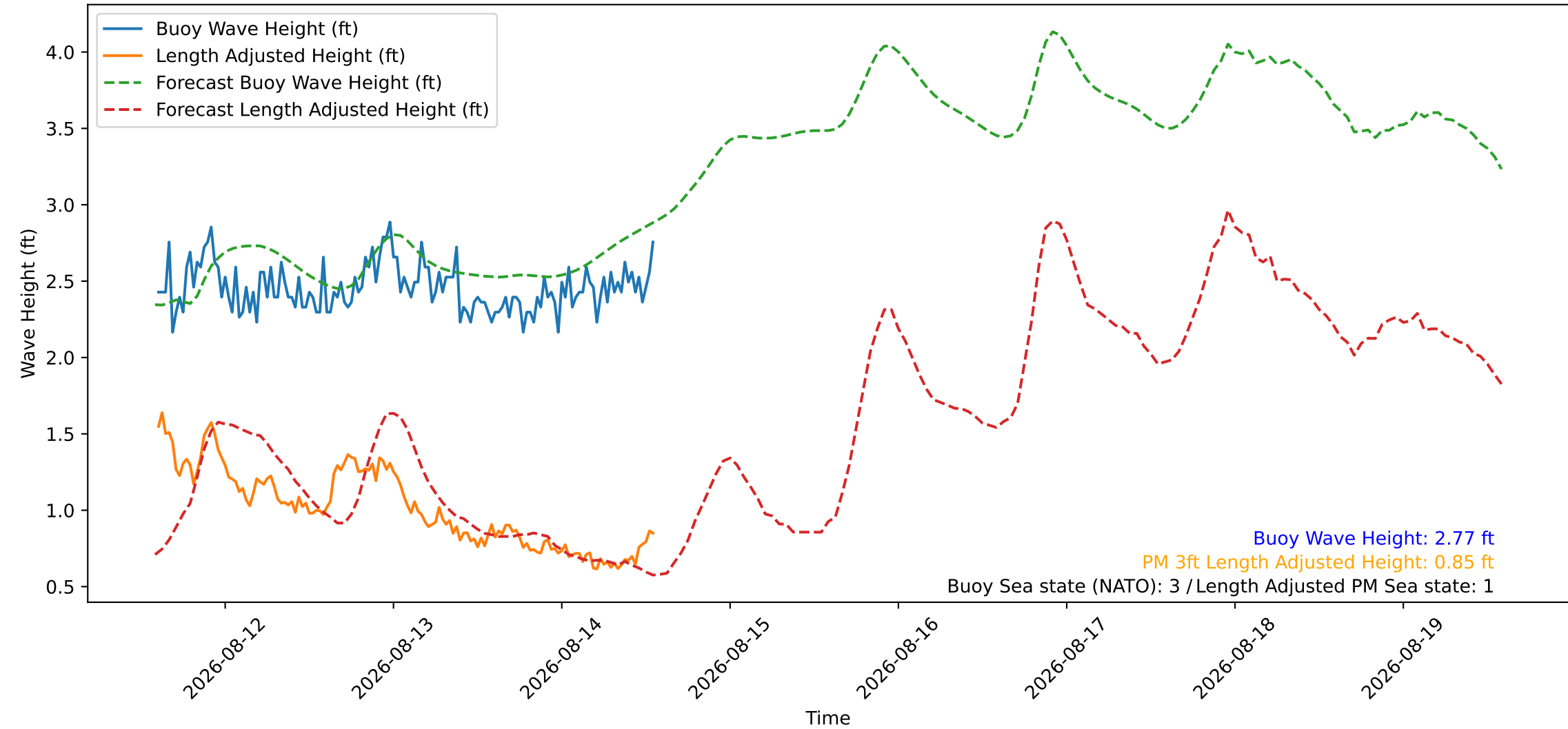
Wave Heights over Time for Red Beach at 2026-08-14 14:20:47
