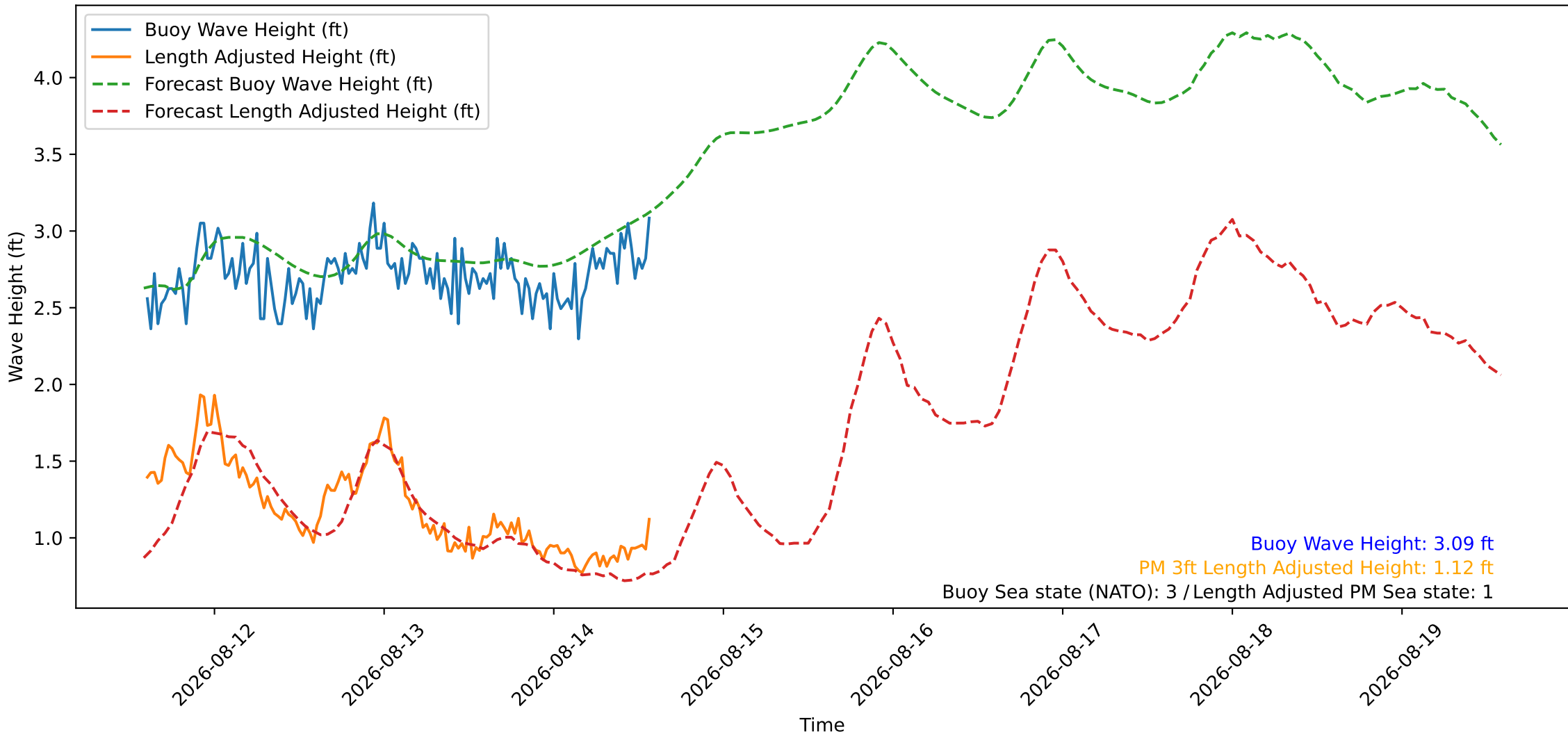
Wave Heights over Time for Oceanside Harbor at 2026-08-14 14:20:26
