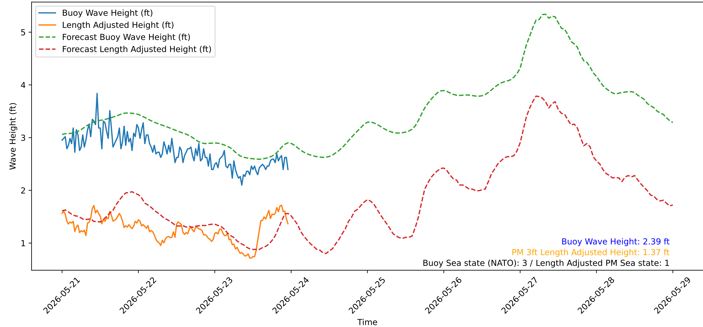
Wave Heights over Time for Oceanside Harbor at 2026-05-23 23:50:31
