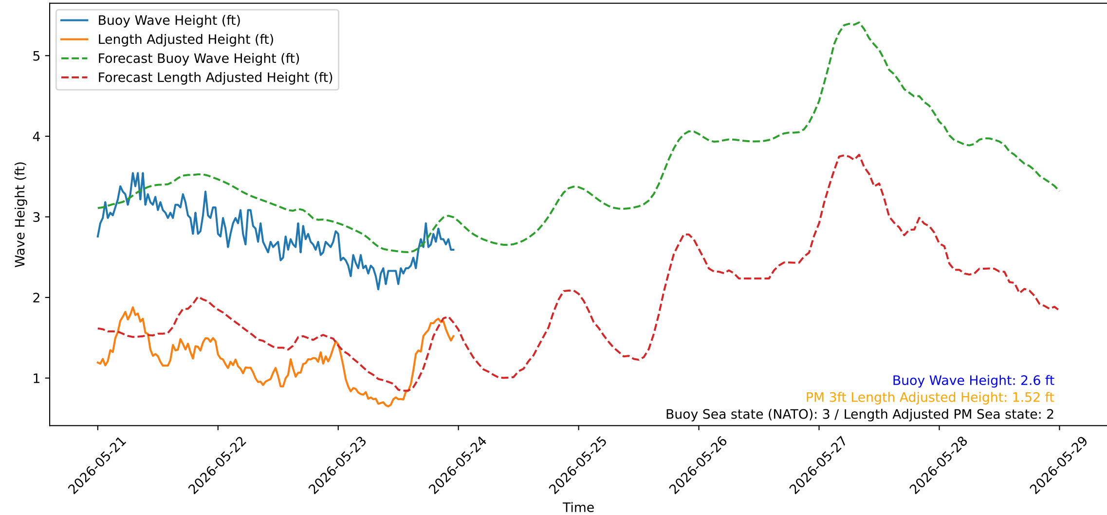
Wave Heights over Time for Green Beach at 2026-05-23 23:51:14
