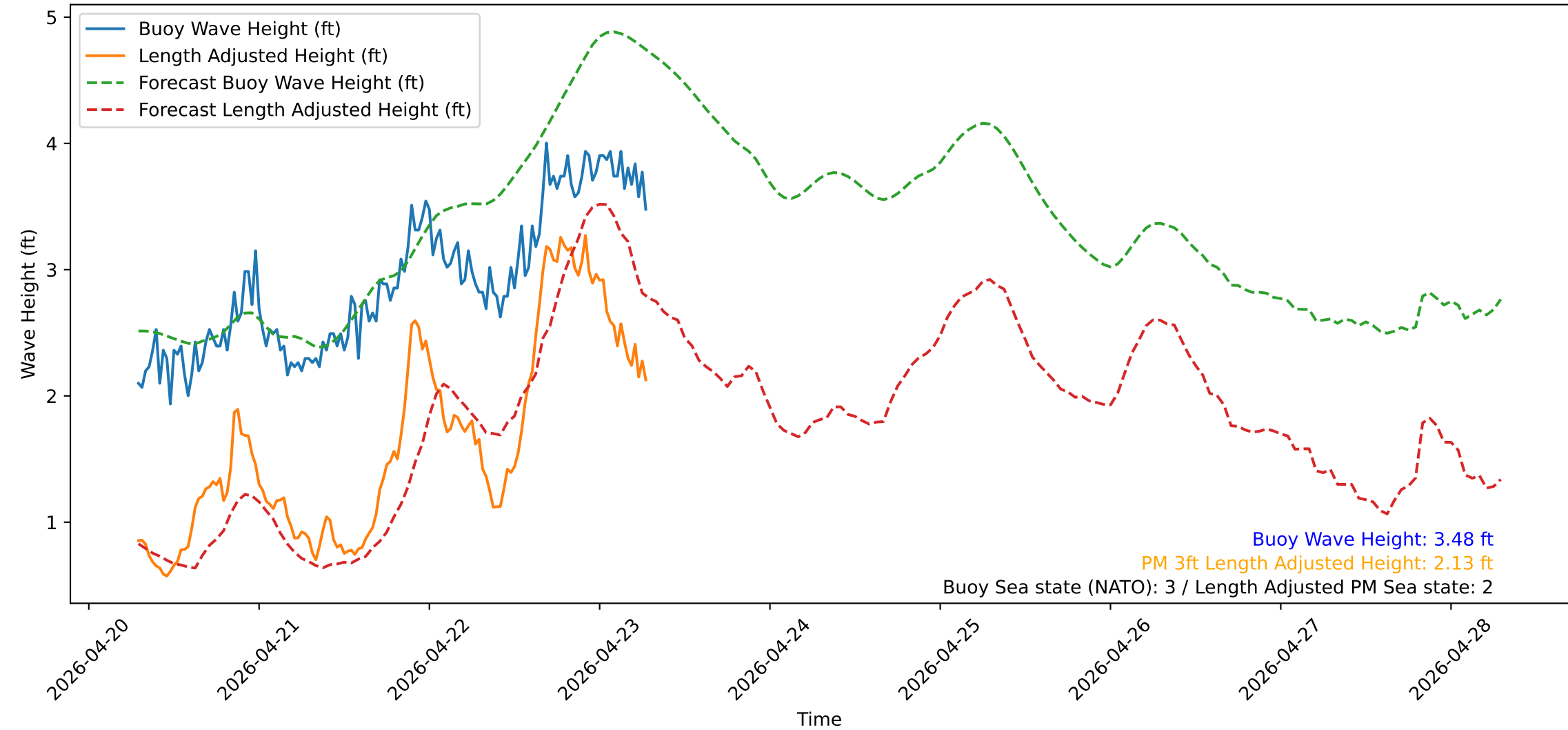
Wave Heights over Time for Green Beach at 2026-04-23 07:11:11
