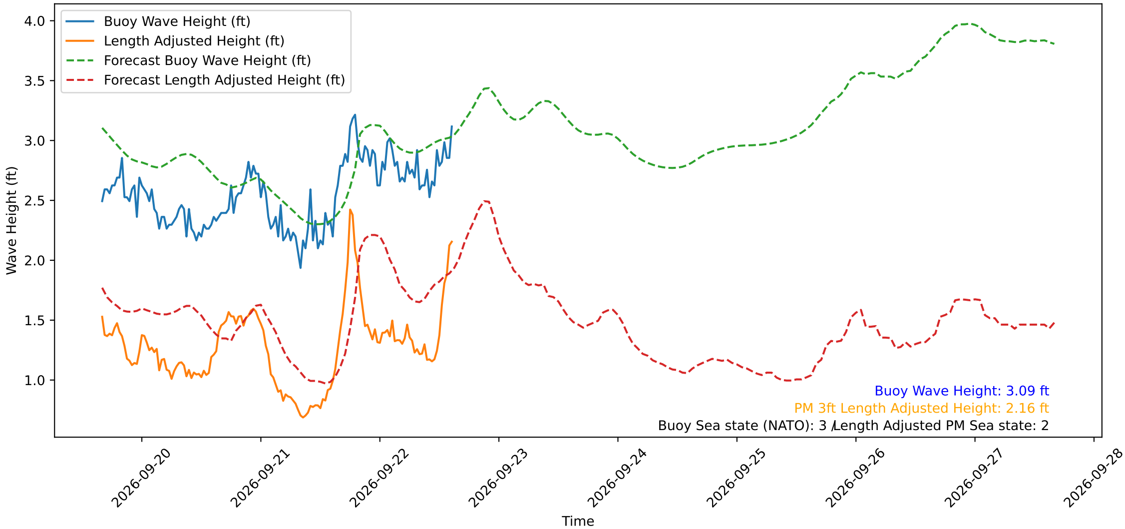
Wave Heights over Time for Green Beach at 2026-09-22 15:31:11
