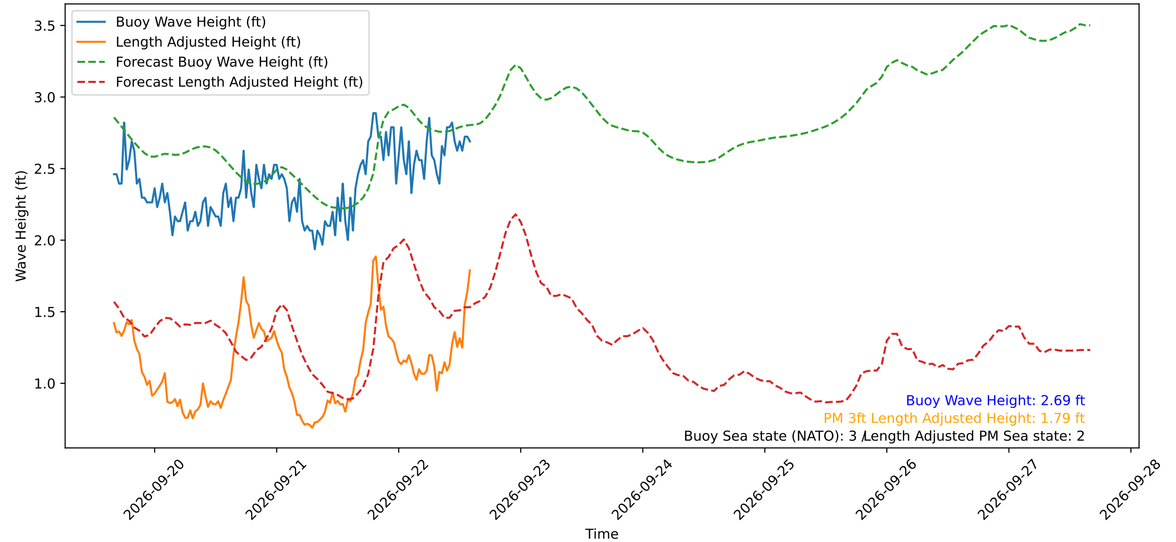
Wave Heights over Time for Red Beach at 2026-09-22 15:30:49
