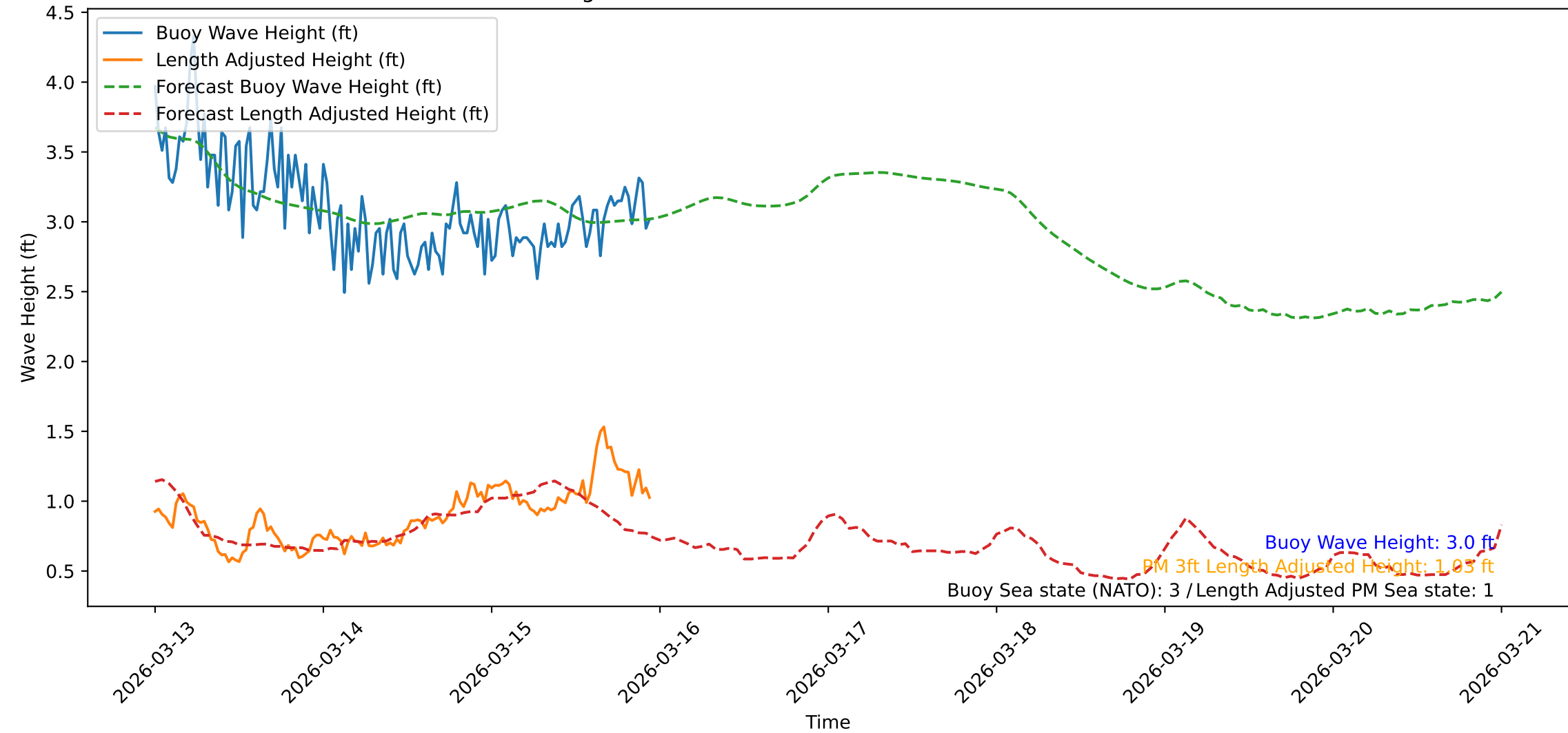
Wave Heights over Time for Red Beach at 2026-03-15 23:31:06
