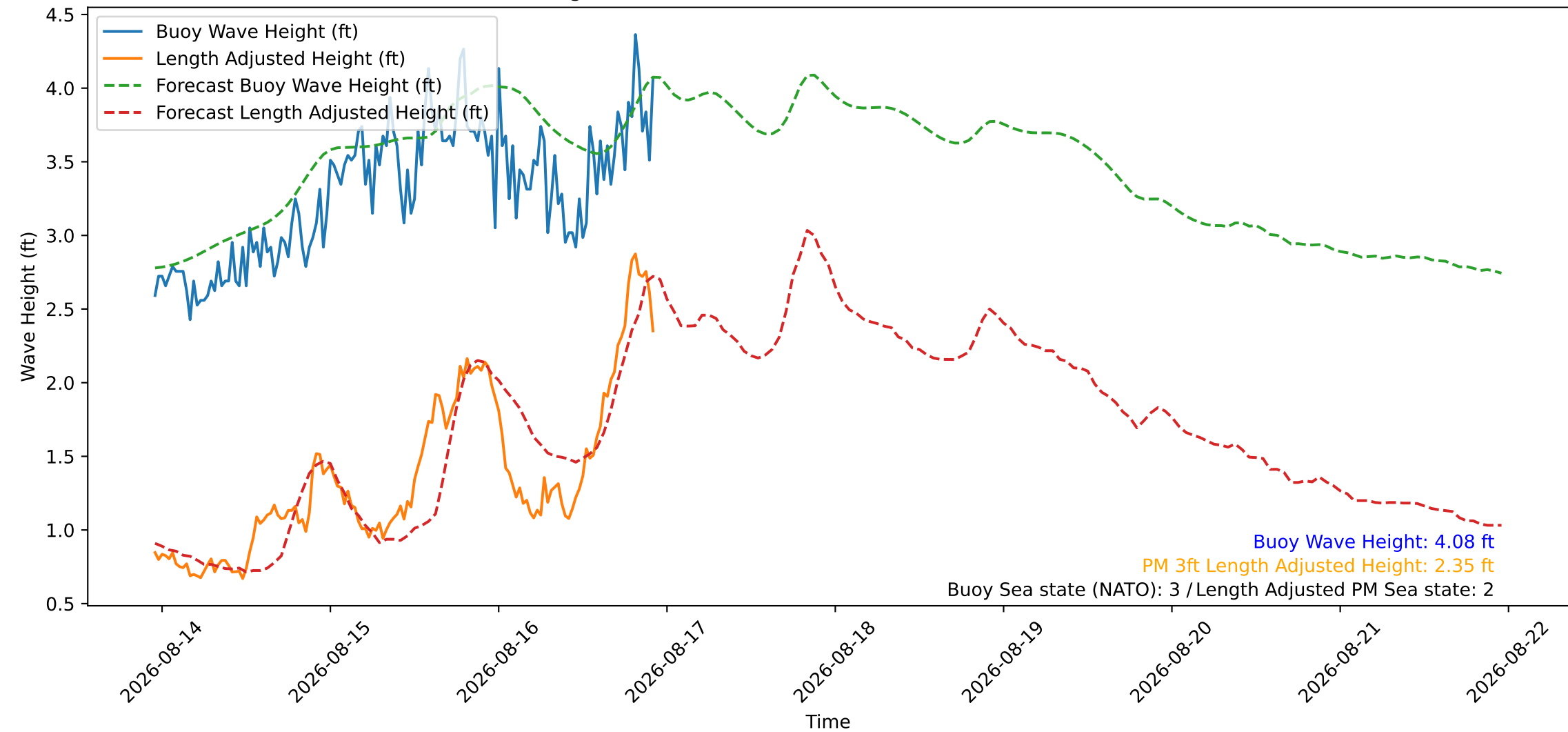
Wave Heights over Time for Green Beach at 2026-08-16 22:41:07
