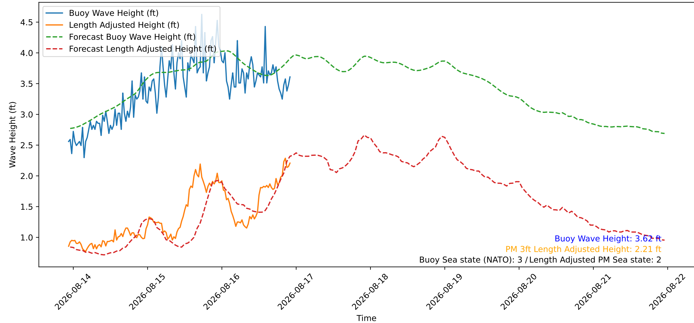
Wave Heights over Time for Oceanside Harbor at 2026-08-16 22:40:26
