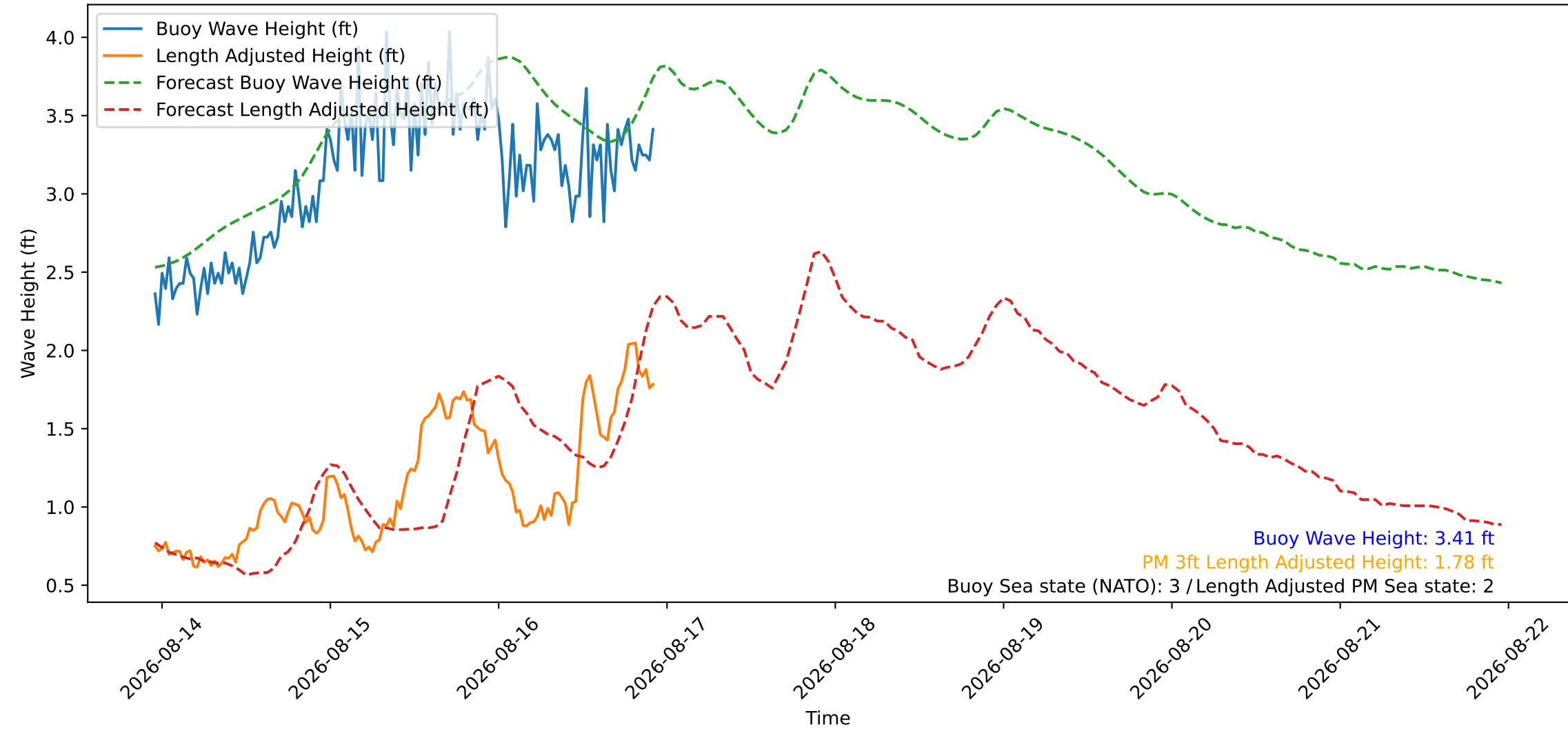
Wave Heights over Time for Red Beach at 2026-08-16 22:40:45
