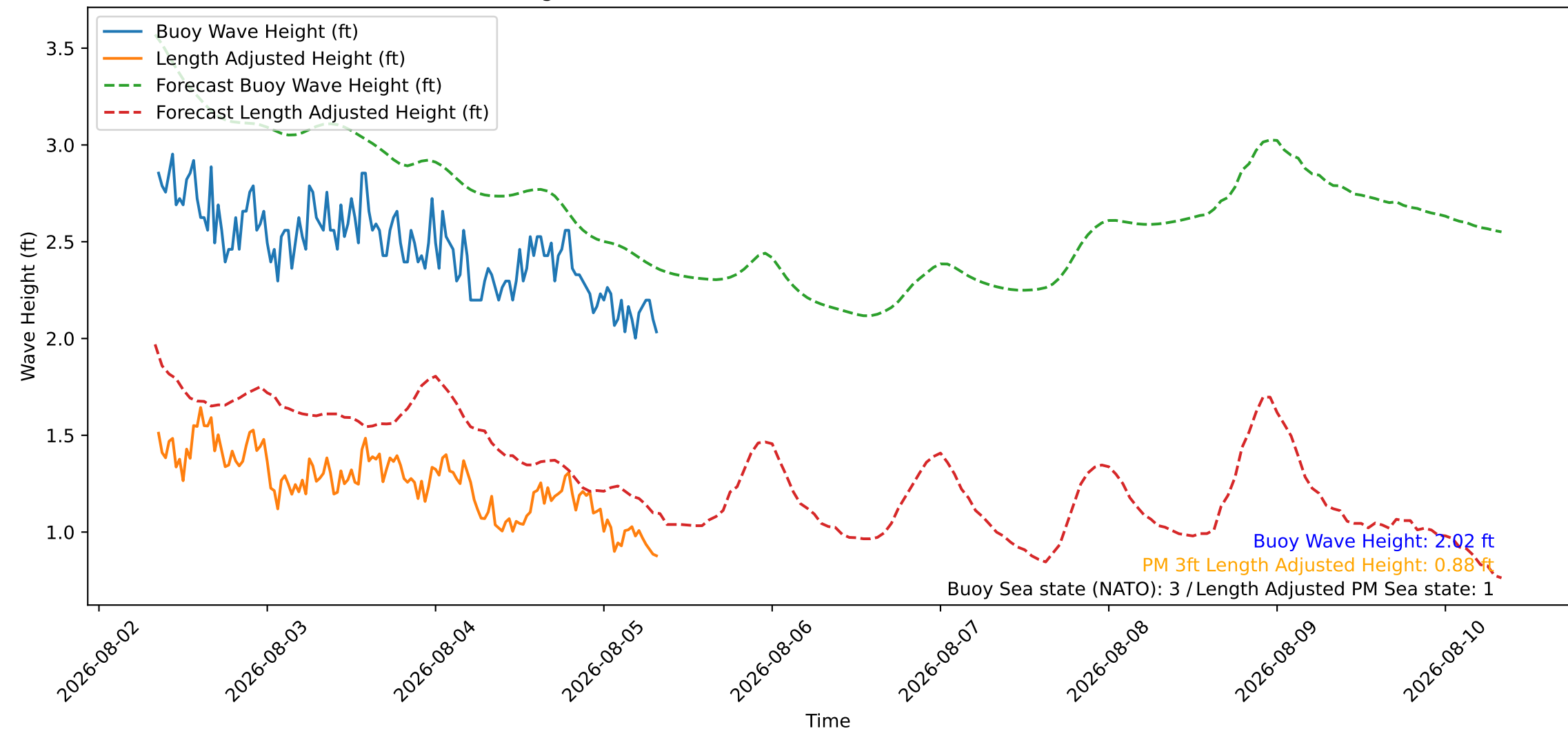
Wave Heights over Time for Oceanside Harbor at 2026-08-05 08:20:27
