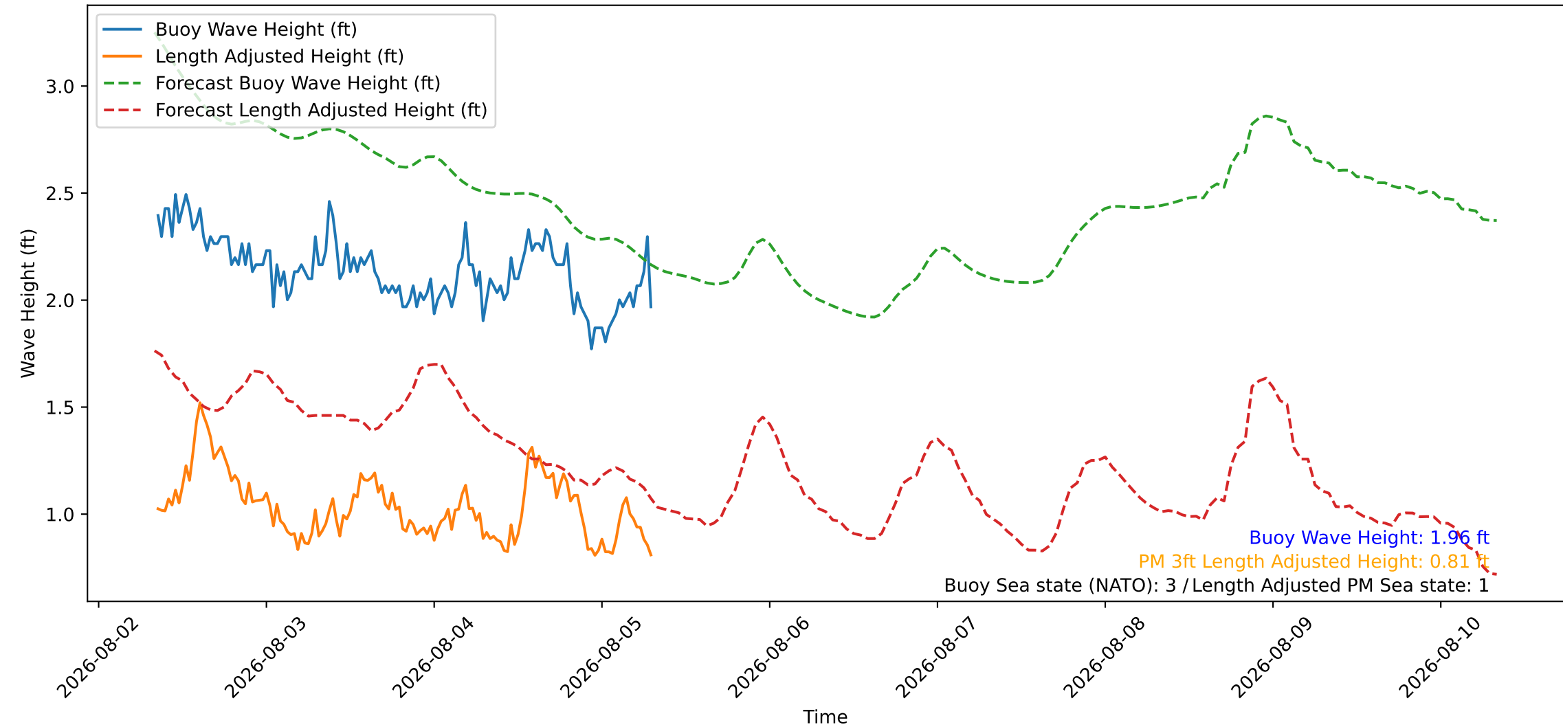
Wave Heights over Time for Red Beach at 2026-08-05 08:20:47
