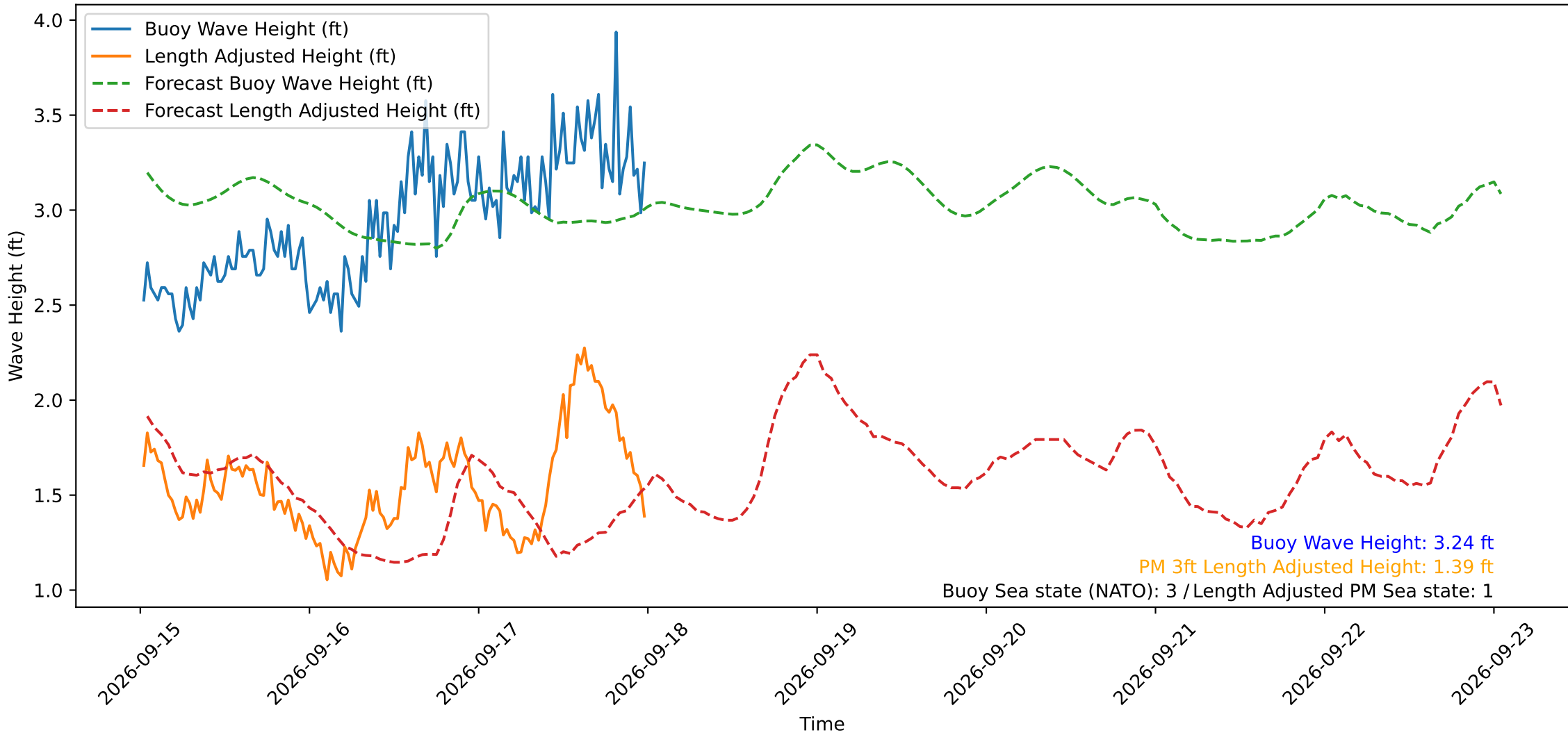
Wave Heights over Time for Oceanside Harbor at 2026-09-18 00:30:30
