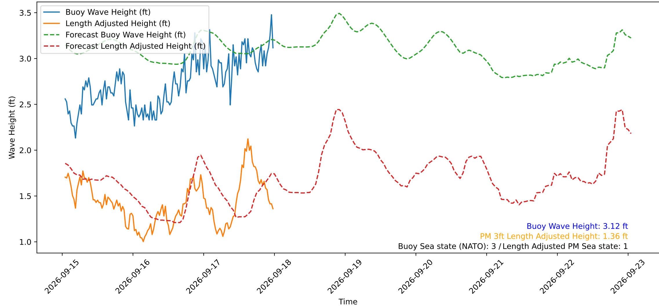
Wave Heights over Time for Green Beach at 2026-09-18 00:31:12
