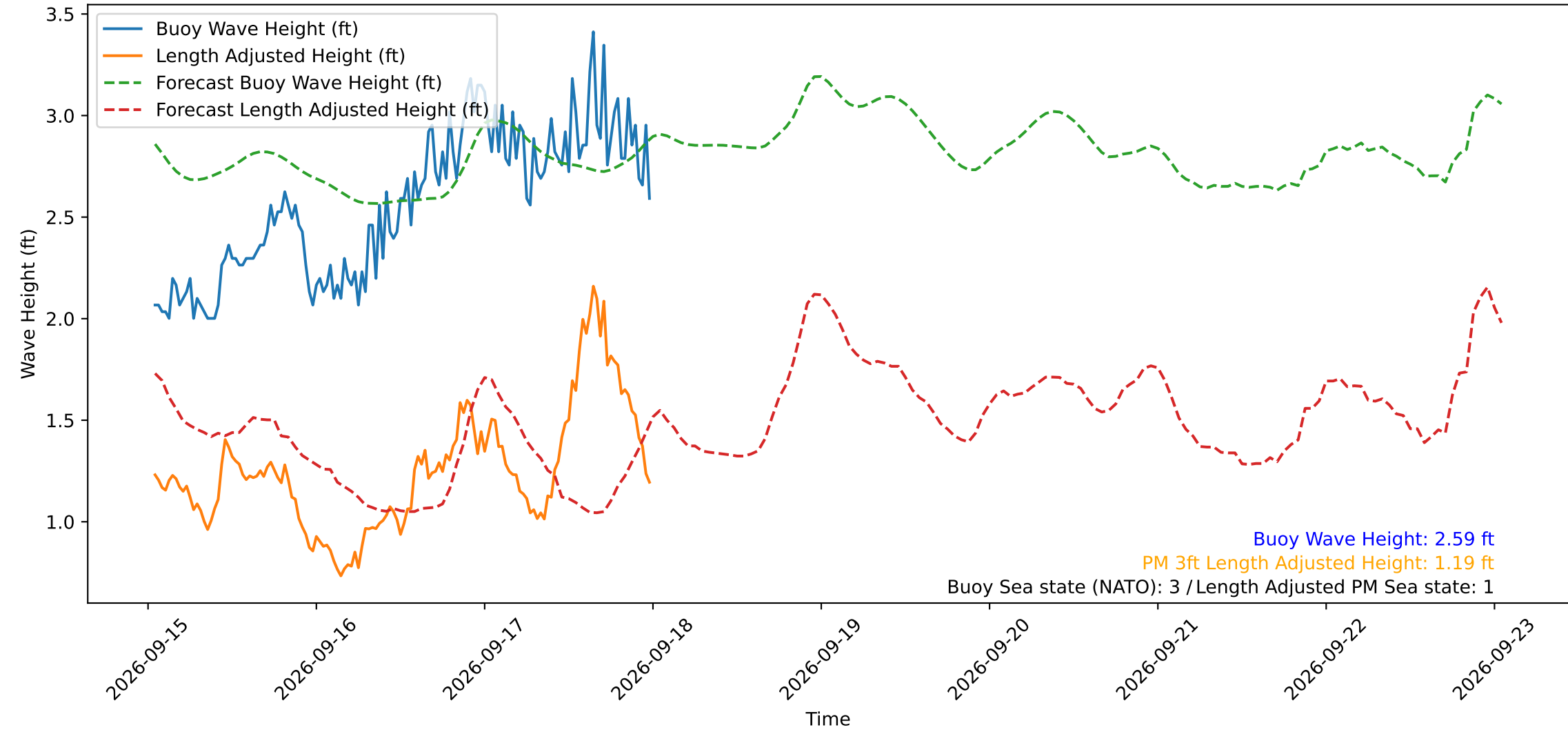
Wave Heights over Time for Red Beach at 2026-09-18 00:30:50
