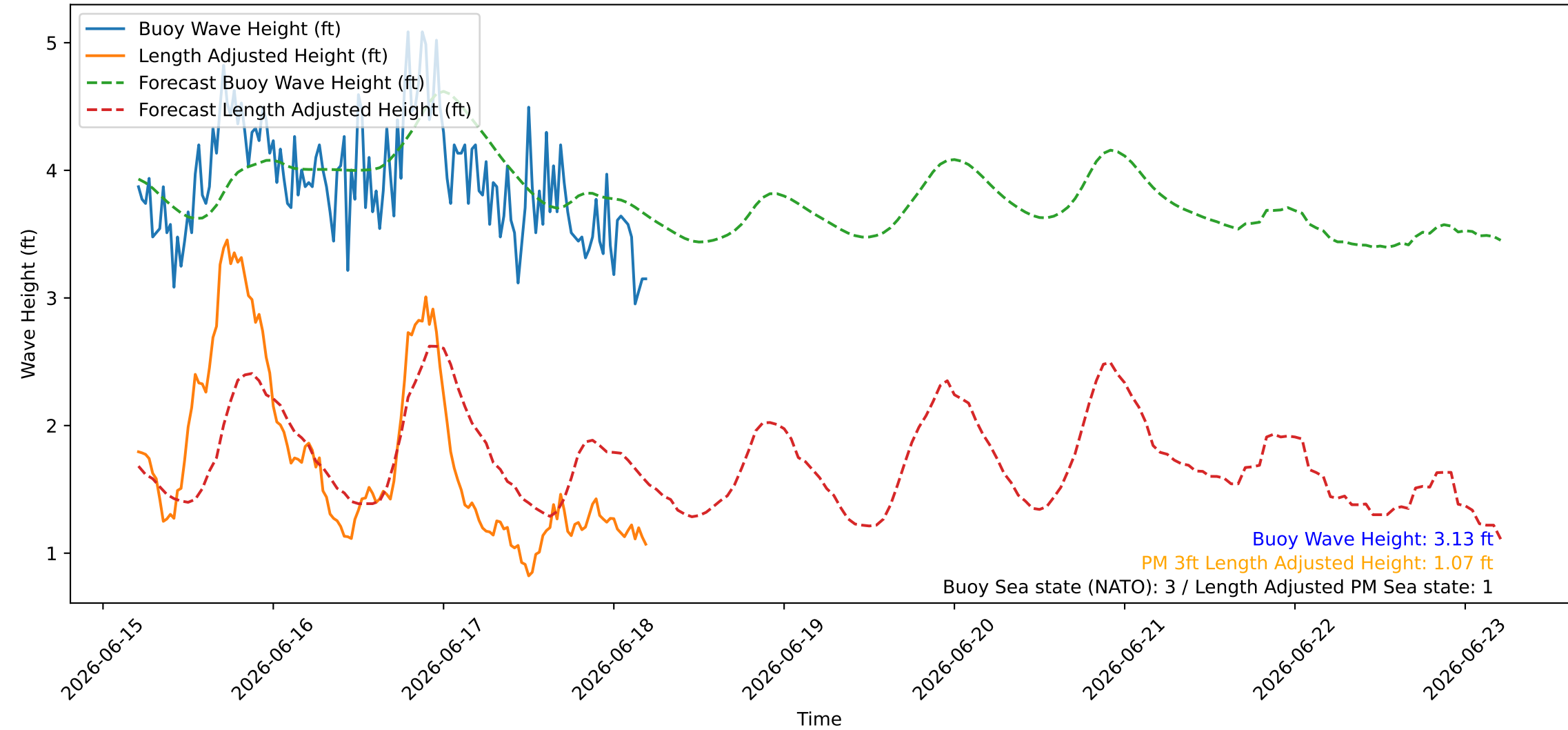
Wave Heights over Time for Green Beach at 2026-06-18 05:11:09
