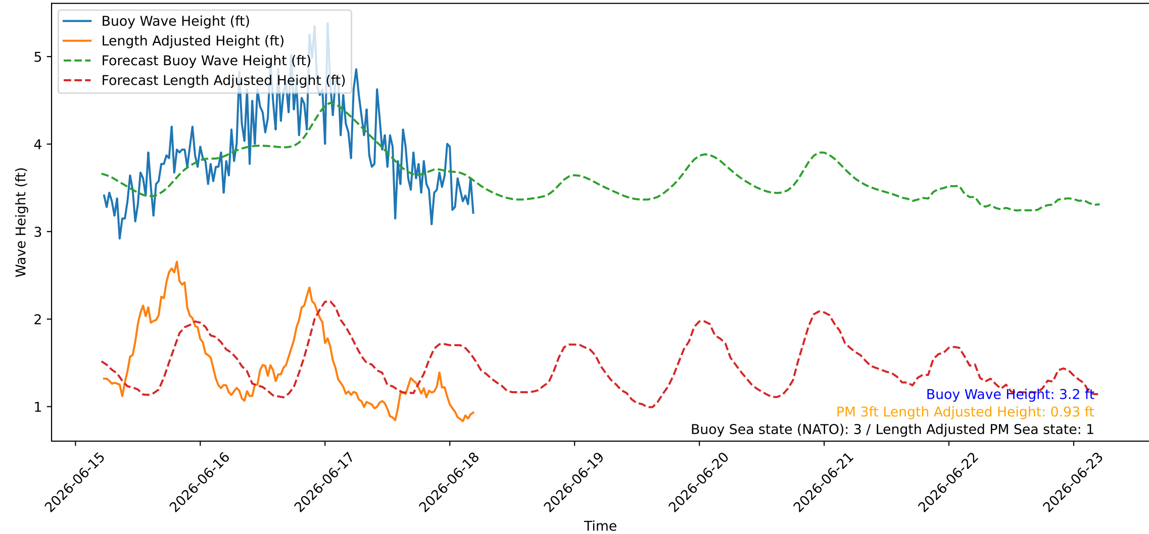
Wave Heights over Time for Red Beach at 2026-06-18 05:10:46
