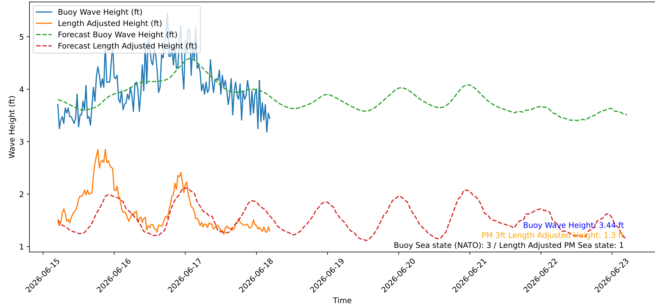
Wave Heights over Time for Oceanside Harbor at 2026-06-18 05:10:26
