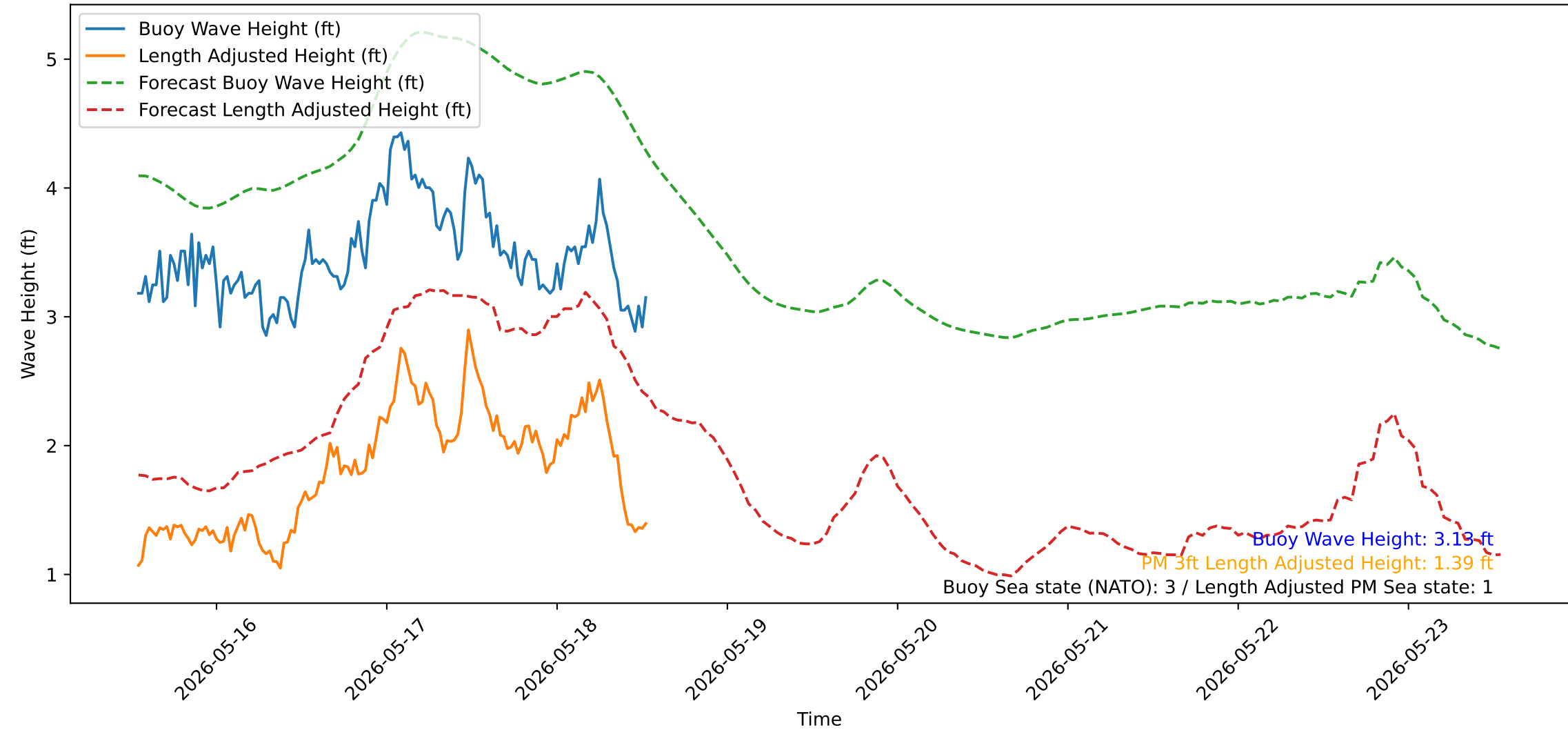
Wave Heights over Time for Green Beach at 2026-05-18 13:11:13
