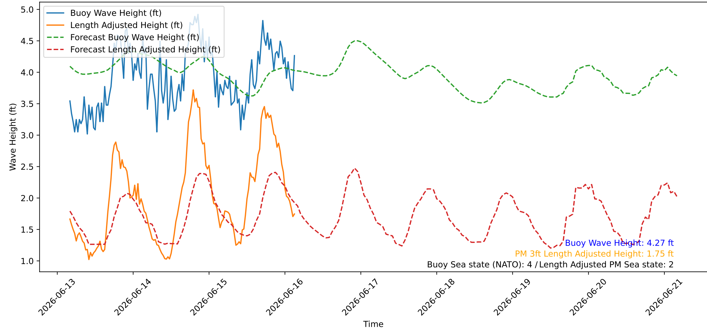
Wave Heights over Time for Green Beach at 2026-06-16 03:51:08
