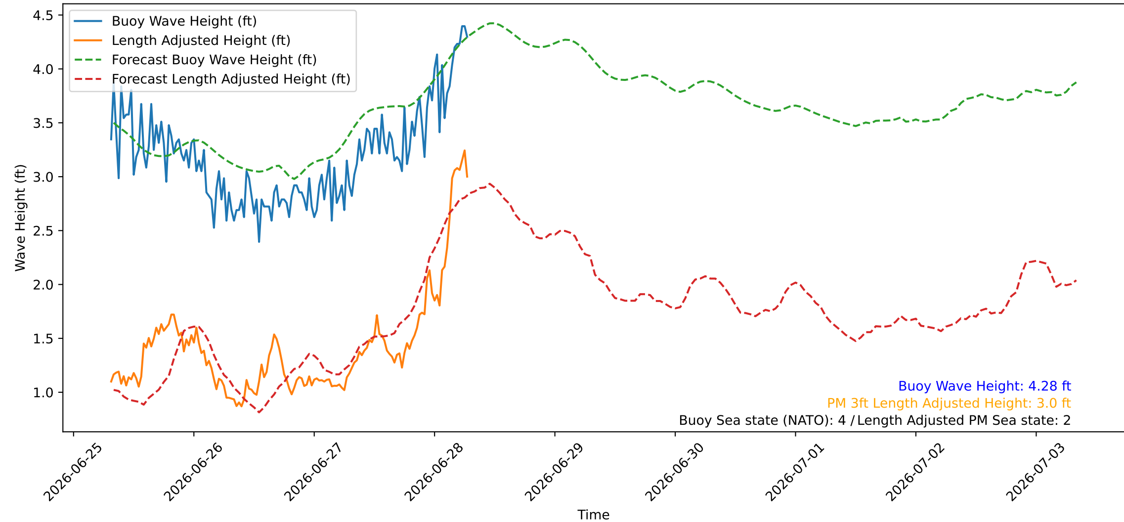
Wave Heights over Time for Oceanside Harbor at 2026-06-28 07:30:26
