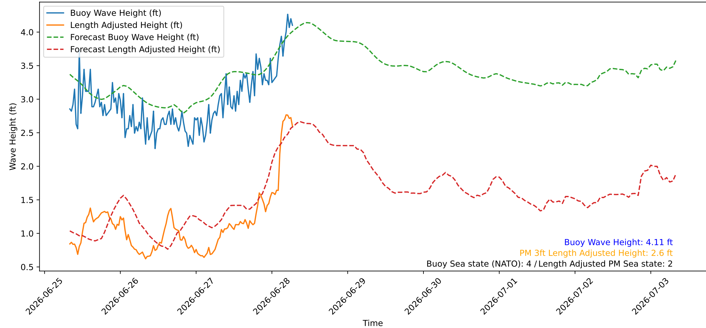
Wave Heights over Time for Red Beach at 2026-06-28 07:30:45
