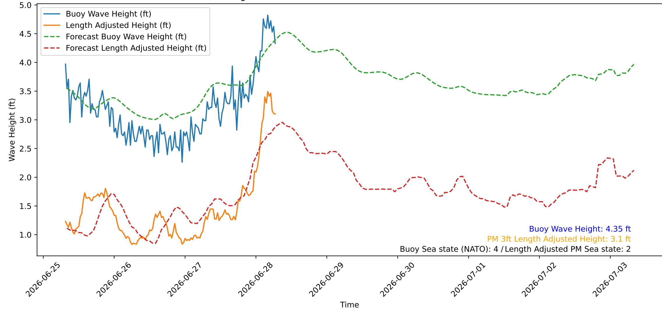
Wave Heights over Time for Green Beach at 2026-06-28 07:31:07
