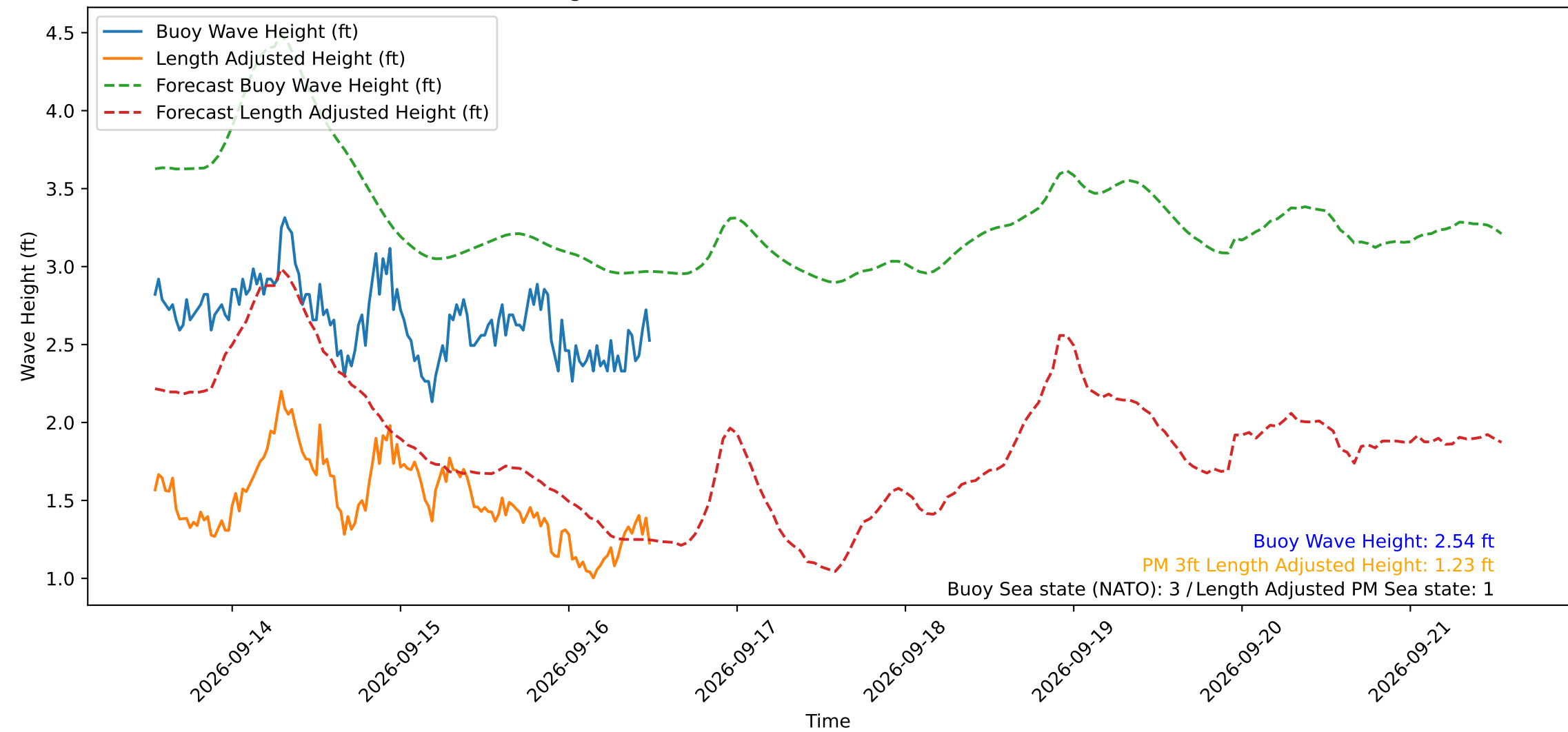
Wave Heights over Time for Green Beach at 2026-09-16 12:31:12
