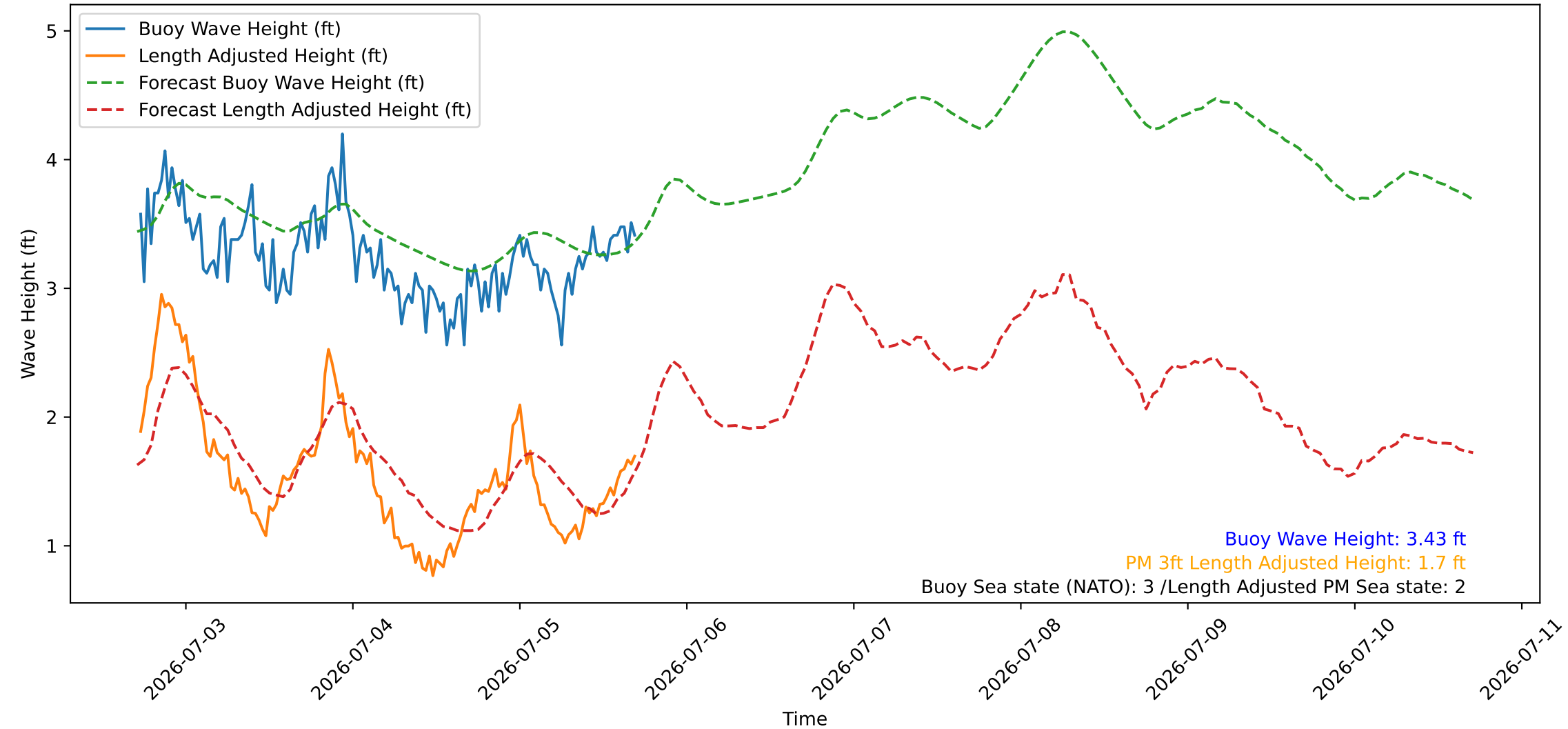
Wave Heights over Time for Green Beach at 2026-07-05 17:21:09
