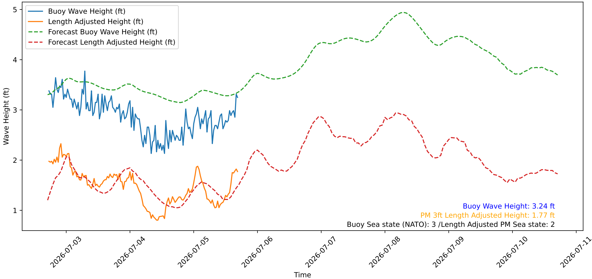
Wave Heights over Time for Oceanside Harbor at 2026-07-05 17:20:26
