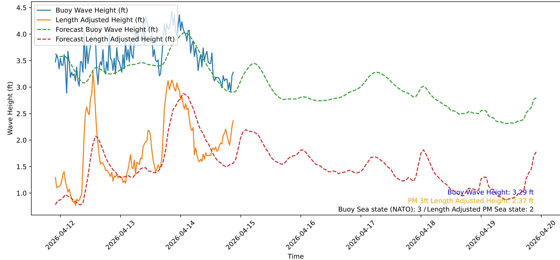
Wave Heights over Time for Red Beach at 2026-04-14 21:40:50
