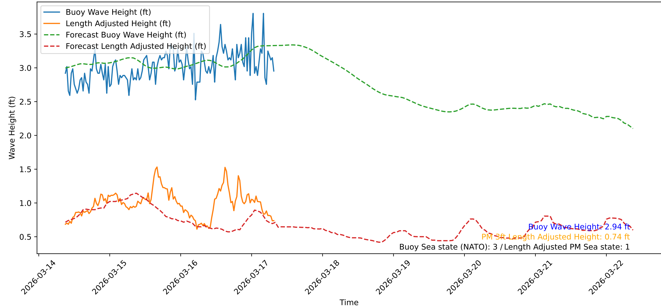
Wave Heights over Time for Red Beach at 2026-03-17 08:31:08
