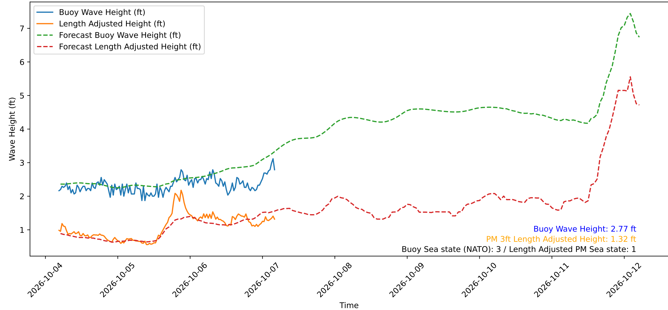
Wave Heights over Time for Oceanside Harbor at 2026-10-07 04:40:29
