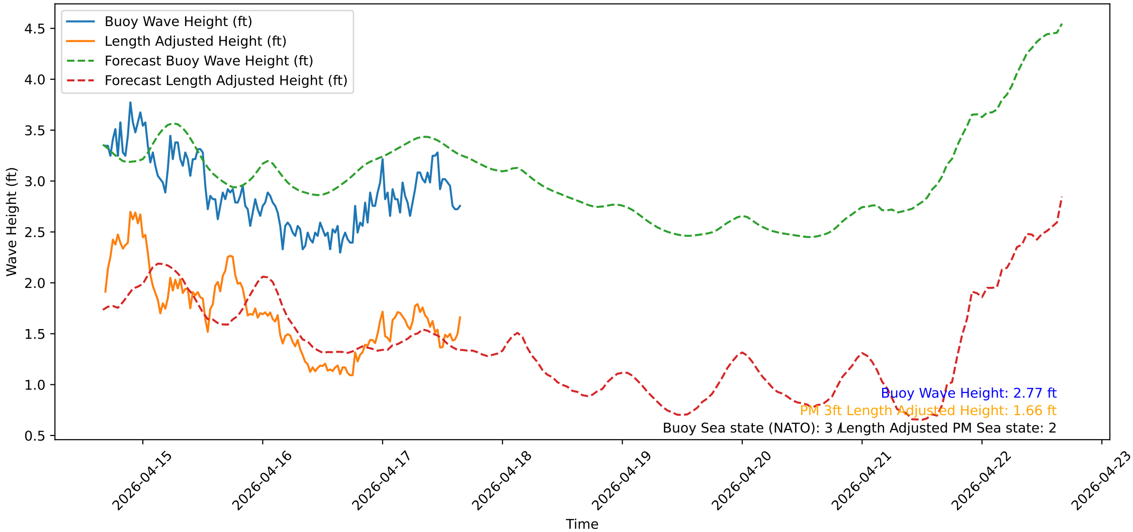
Wave Heights over Time for Oceanside Harbor at 2026-04-17 16:20:31
