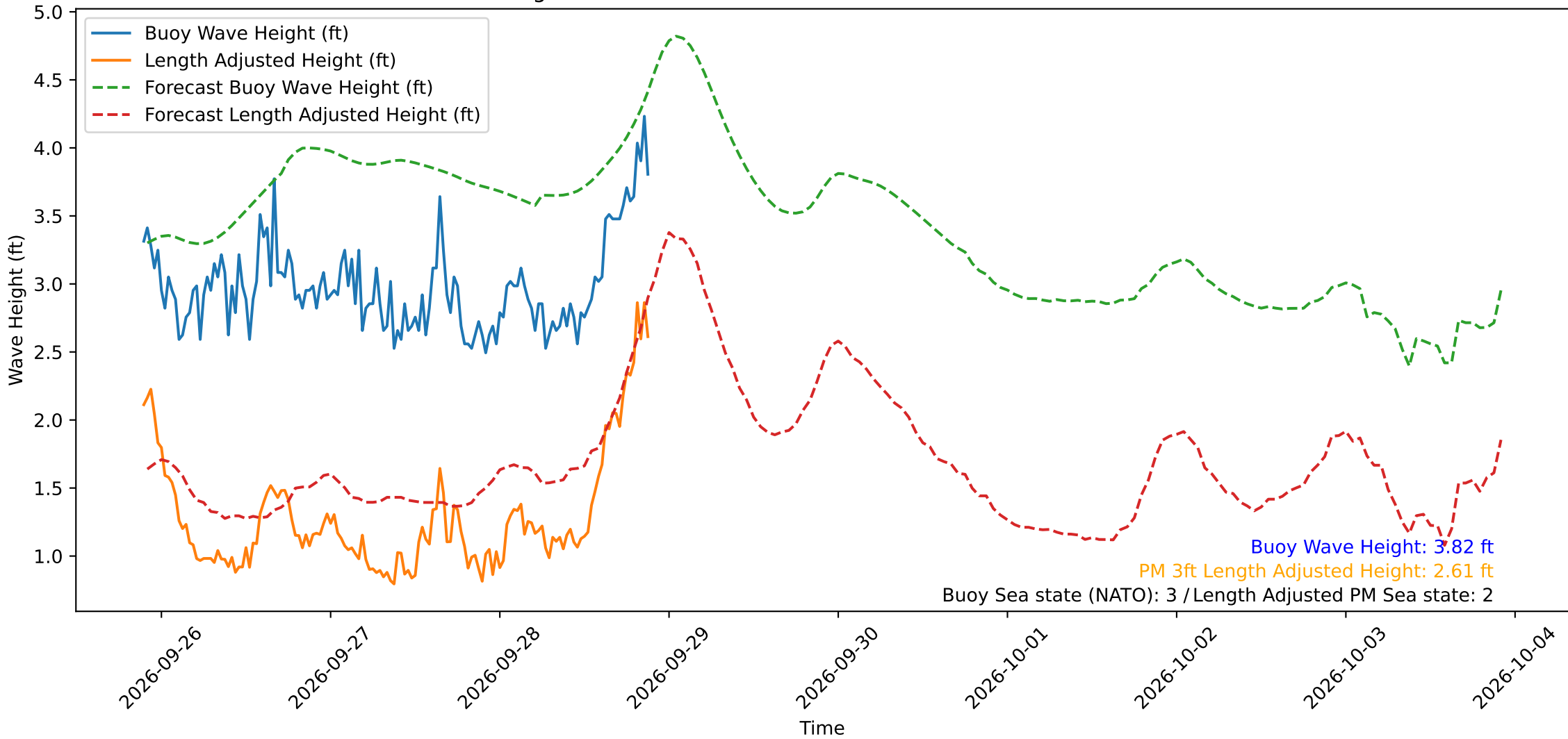
Wave Heights over Time for Oceanside Harbor at 2026-09-28 21:40:29
