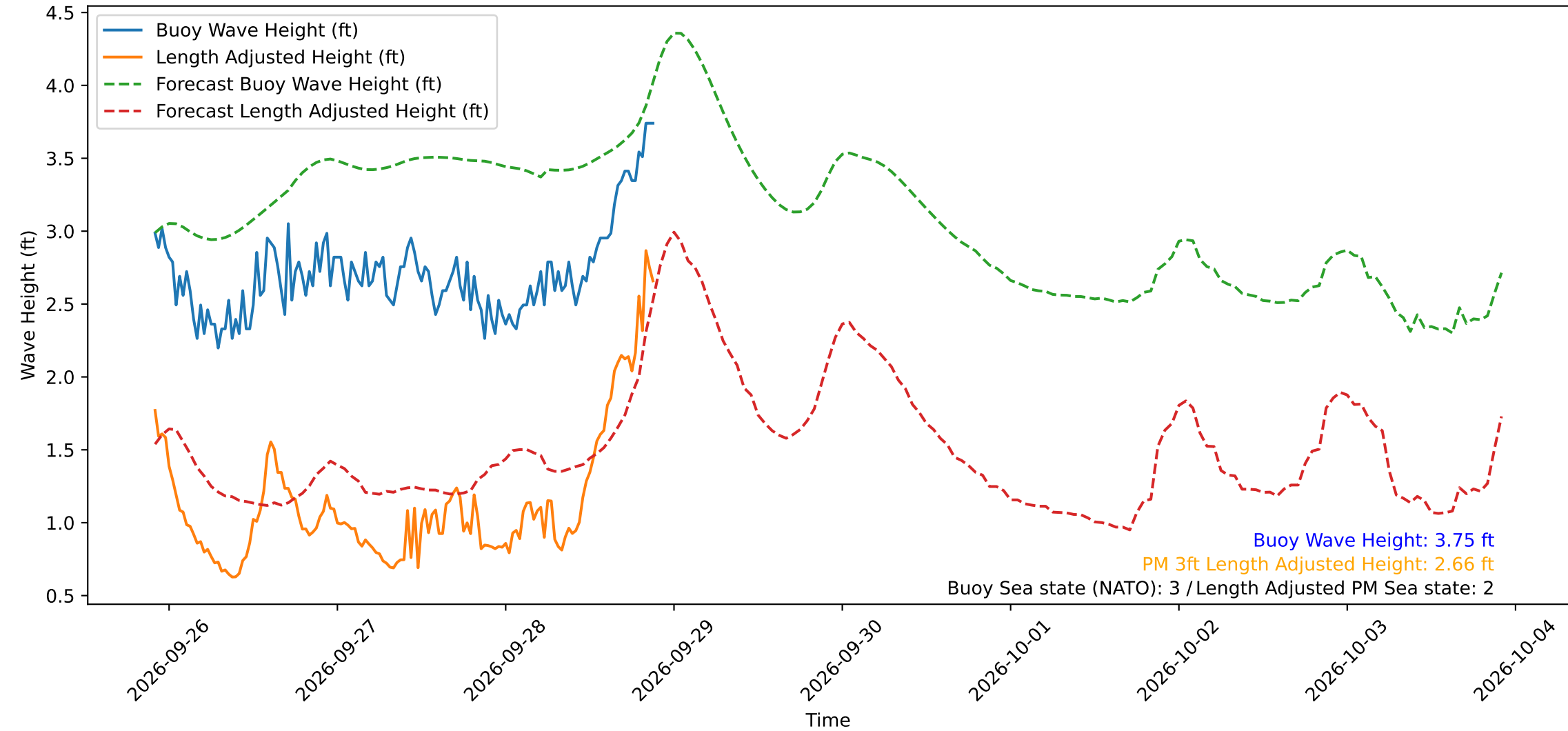
Wave Heights over Time for Red Beach at 2026-09-28 21:40:49
