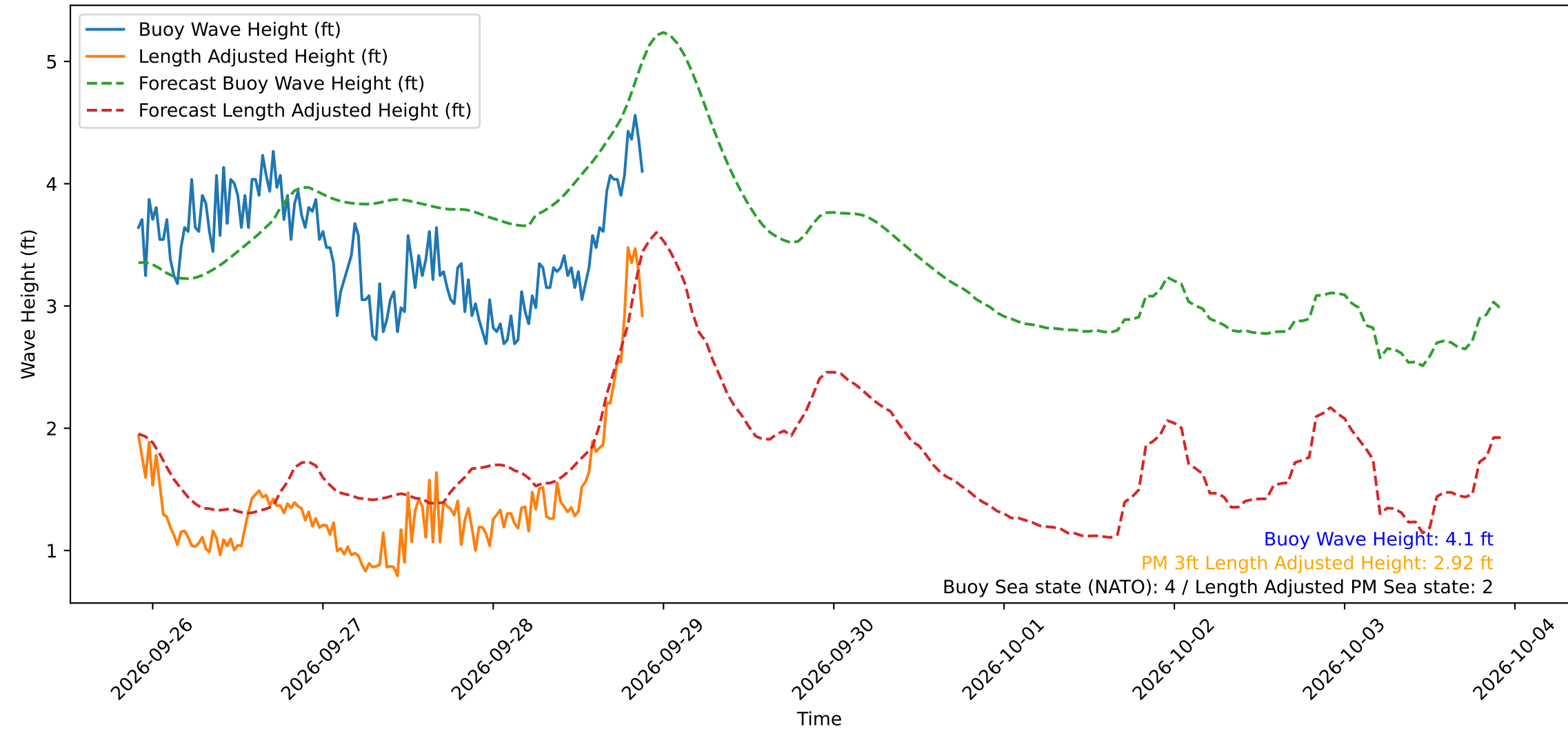
Wave Heights over Time for Green Beach at 2026-09-28 21:41:12
