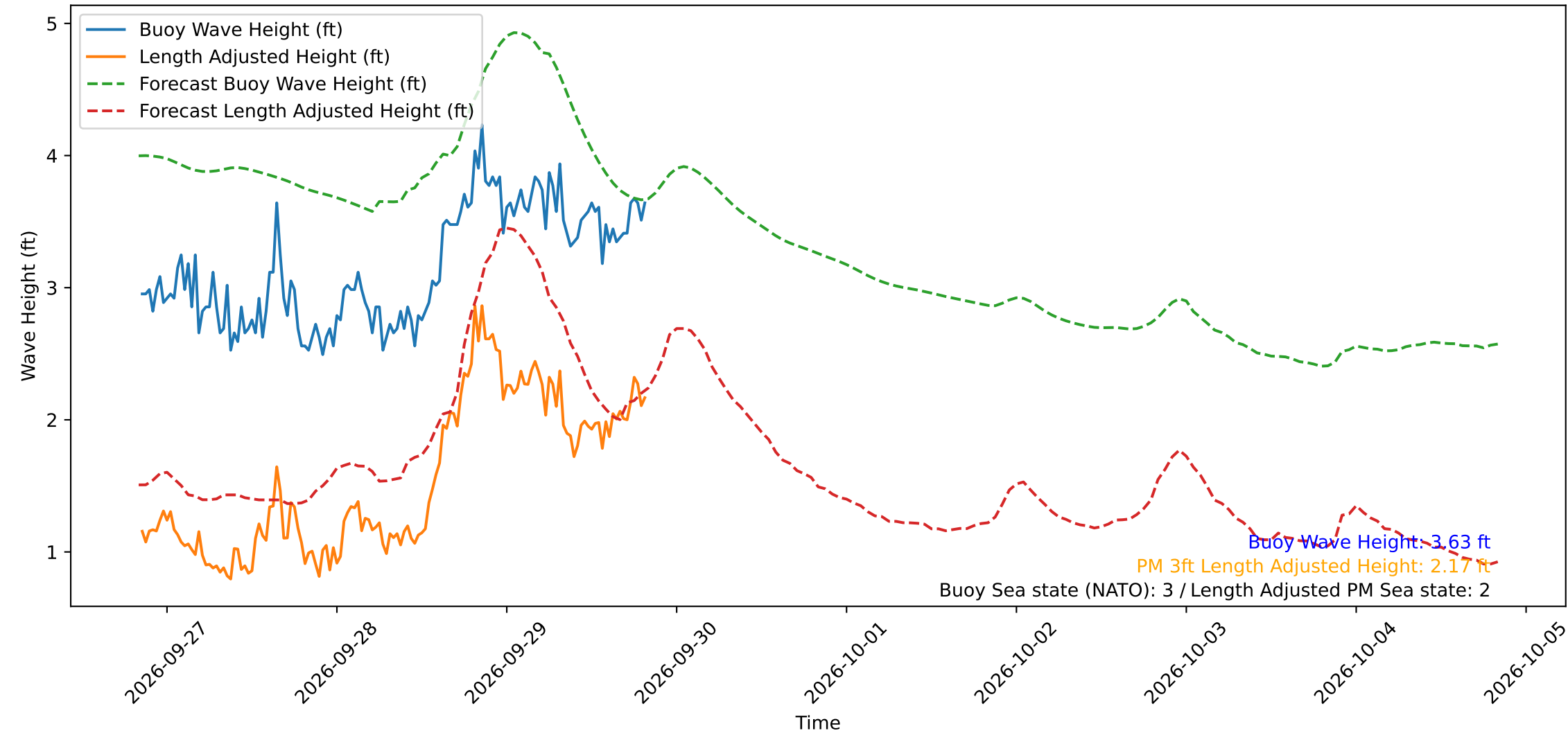
Wave Heights over Time for Oceanside Harbor at 2026-09-29 20:20:30
