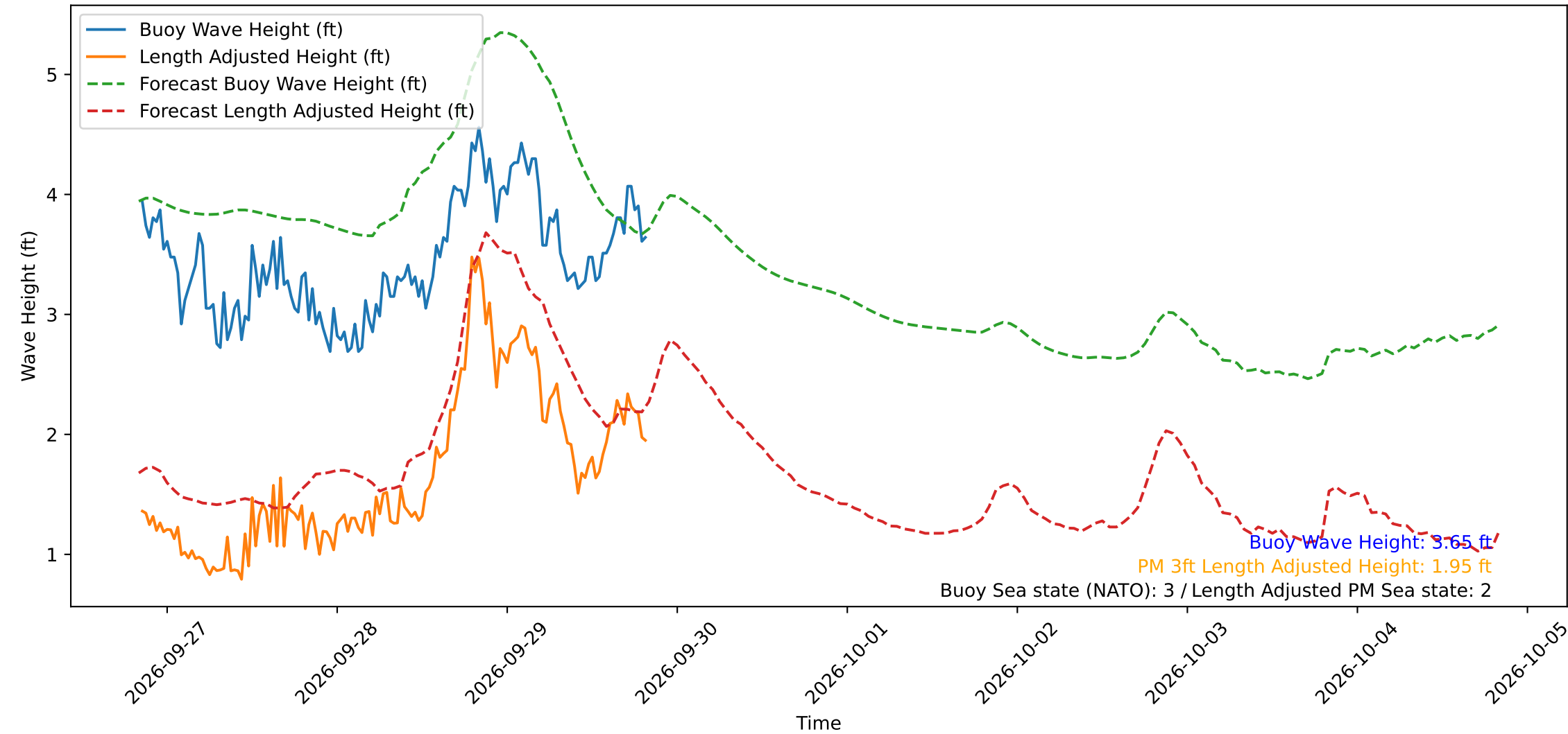
Wave Heights over Time for Green Beach at 2026-09-29 20:21:15
