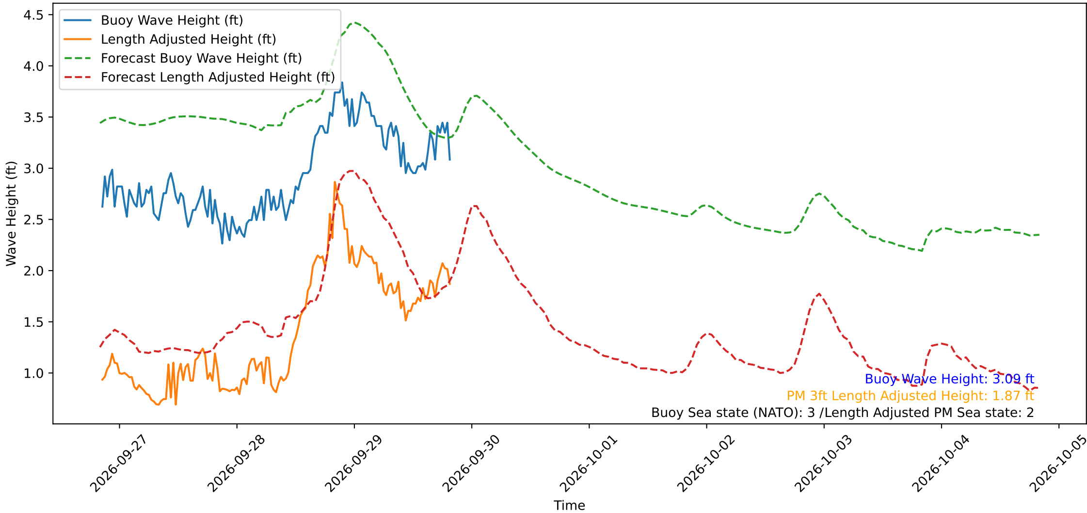
Wave Heights over Time for Red Beach at 2026-09-29 20:20:51
