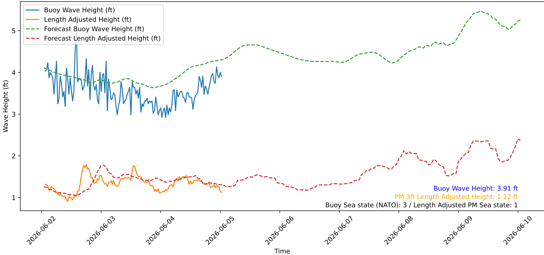
Wave Heights over Time for Oceanside Harbor at 2026-06-05 01:20:26
